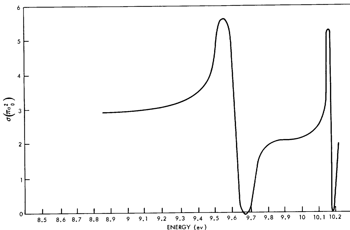
Figure 3—Singlet S-wave cross-section corresponding to the phase shifts in Figure 2. The value a_0 is the Bohr radius.
