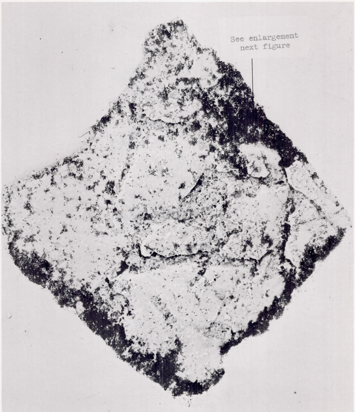
L-63-72 Figure 21.- Electron micrograph of magnesium oxide inclusion in as-received Cr-MgO composite sheet. x12,500.
