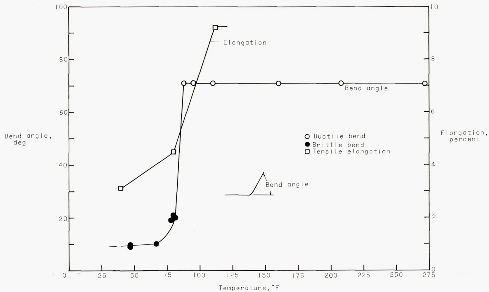
Figure 10.- Curves showing brittle to ductile transition in bending and tension.
