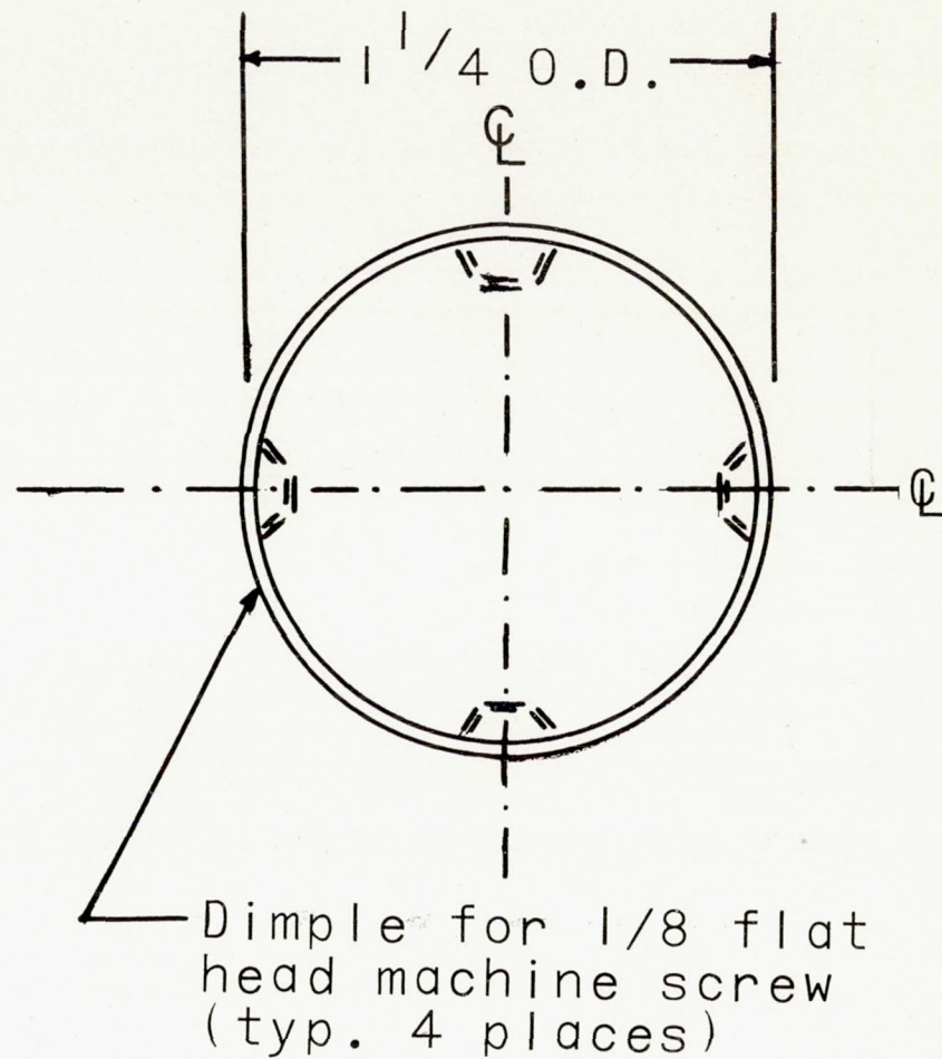
Figure 26.- Proposed dynamic-oxidation specimen for testing in the hypersonic wind tunnel. Specimen failed on fabrication.
