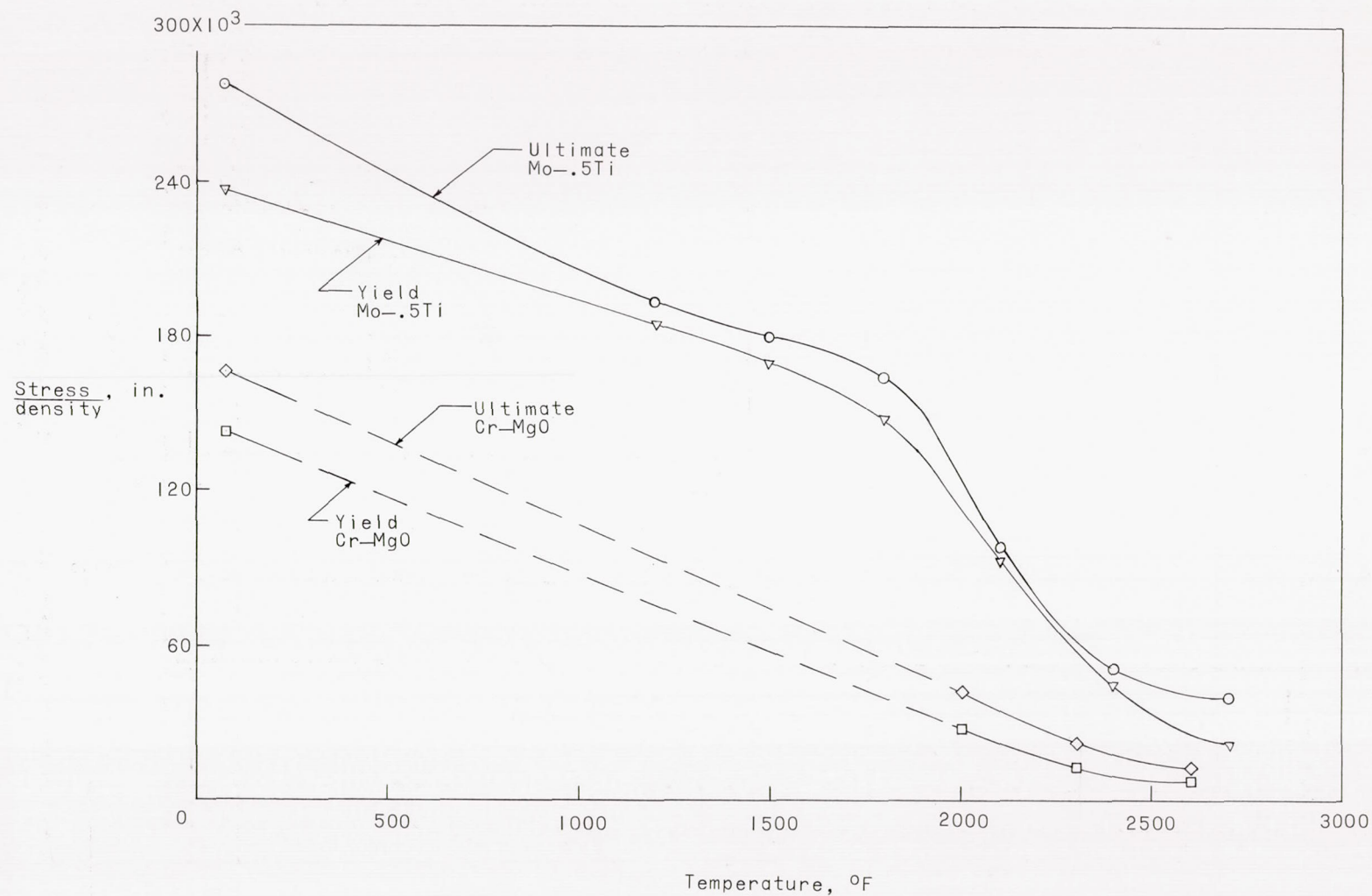
Figure 9.- Comparison of Cr-MgO composite sheet and Mo-0.5 Ti sheet on a weight-strength basis for temperatures ranging from 100° F to 2600° F.
