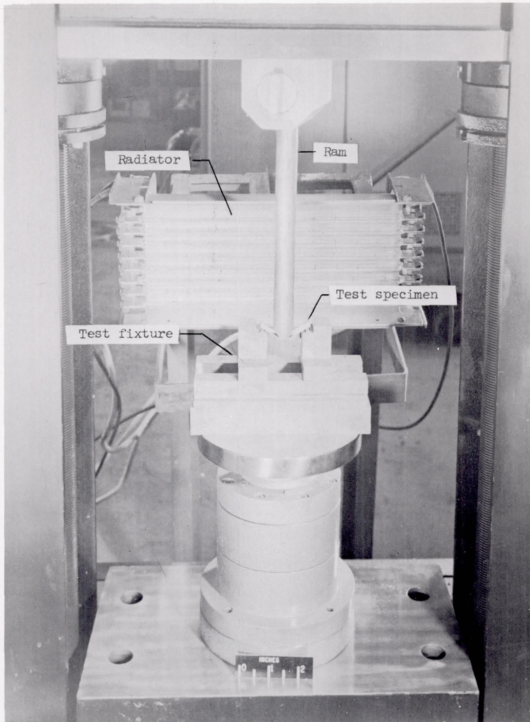
Figure 3.- Test equipment for determining bend transition temperature. One bank of radiators removed.
