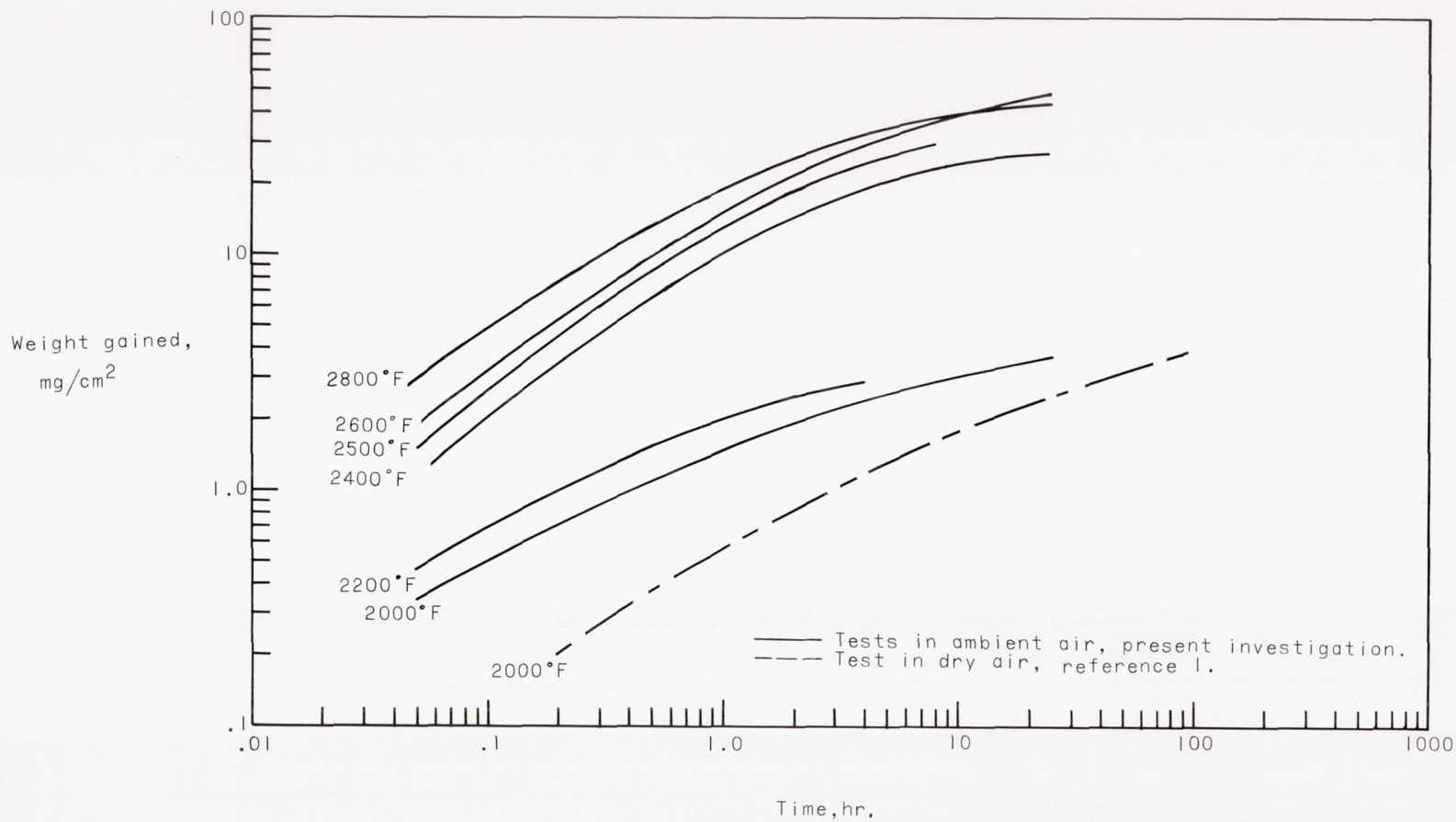
Figure 11.- Oxidation curves for the Cr-MgO composite showing variation of weight gain with time.
