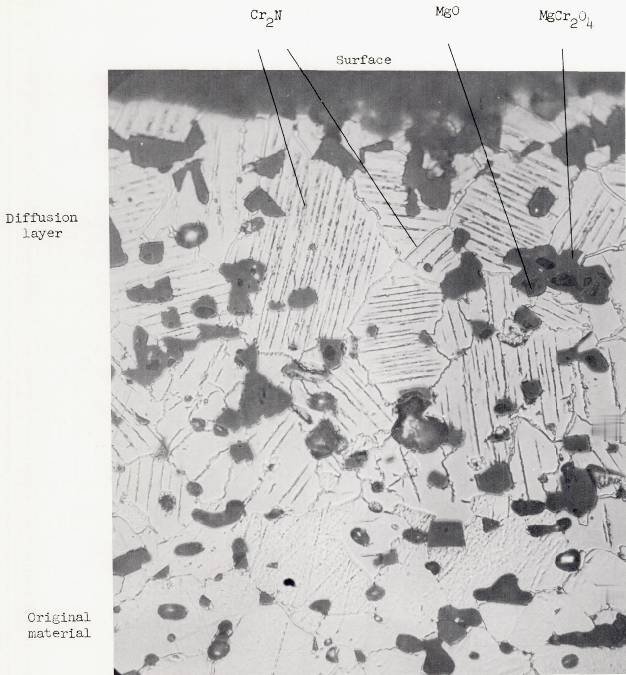
I-63-71 Figure 20.- Microstructure of Cr-MgO composite sheet, after exposure of 4 hours at 2500° F in air. Transverse section. x1000.
