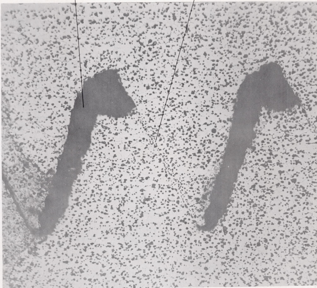
Figure 25.- Microstructure showing the threads of a sectioned bolt and nut assembly after exposure for 1 hour at 2500° F. x100.
