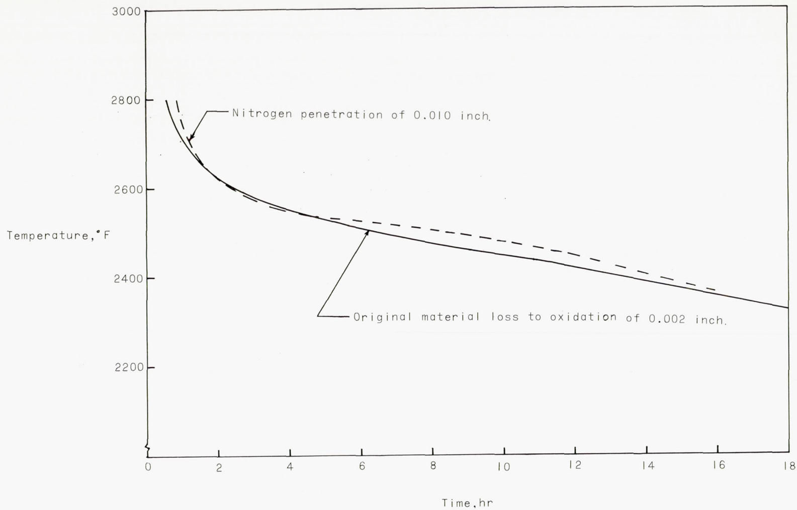
Figure 14.- Temperature-time curves showing 0.002-inch loss of material to oxidation and 0.010 inch of material to nitrogen penetration on 0.020-inch-thick sheet.
