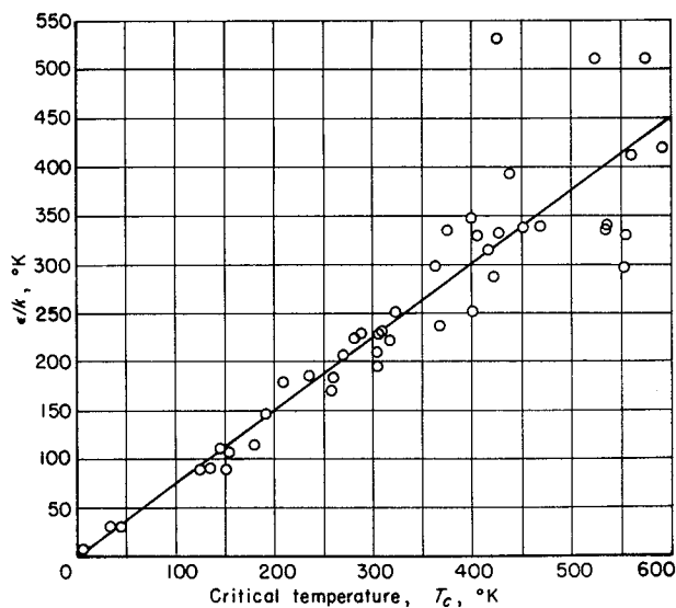
FIGURE 6.—Correlation between \epsilon/k and the critical temperature.
