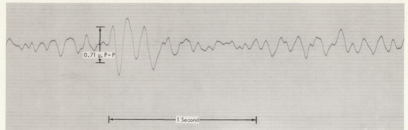
(b) Lateral plus 90-degree axis. Signal of the 9-cps vibration.
