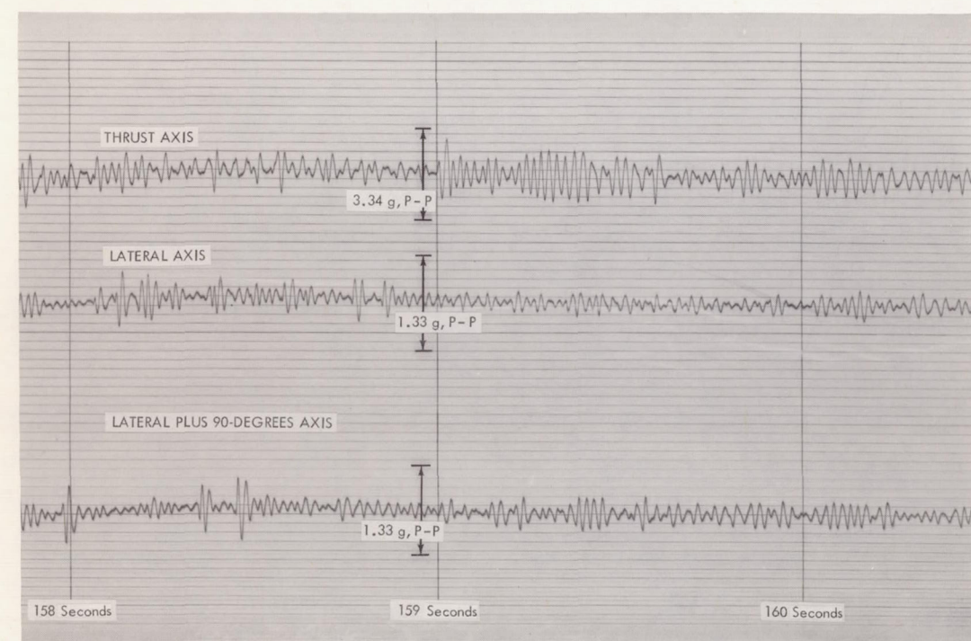
Figure 14—Vibrations at first-stage engine cutoff; instantaneous acceleration versus time; signal filtered with a narrow-band filter. Signal of the 46.5-cps vibration.
