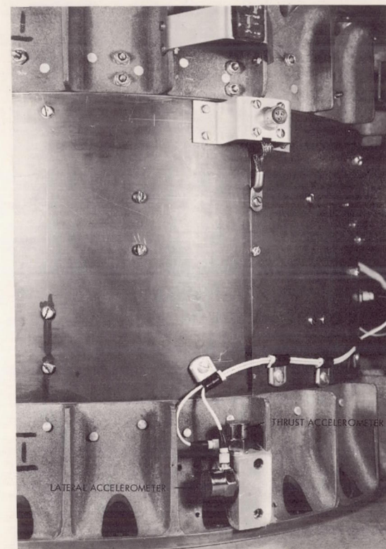
Figure 3—Locations of the thrust and lateral accelerometers on the Dutchman.
