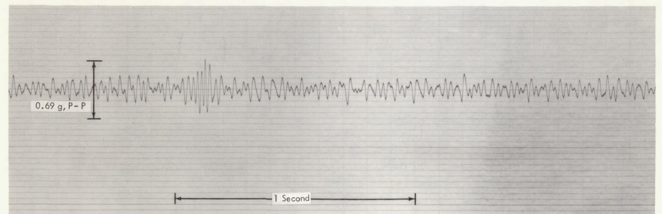
(c) Lateral plus 90-degree axis. Signal of the 60-cps vibration.
