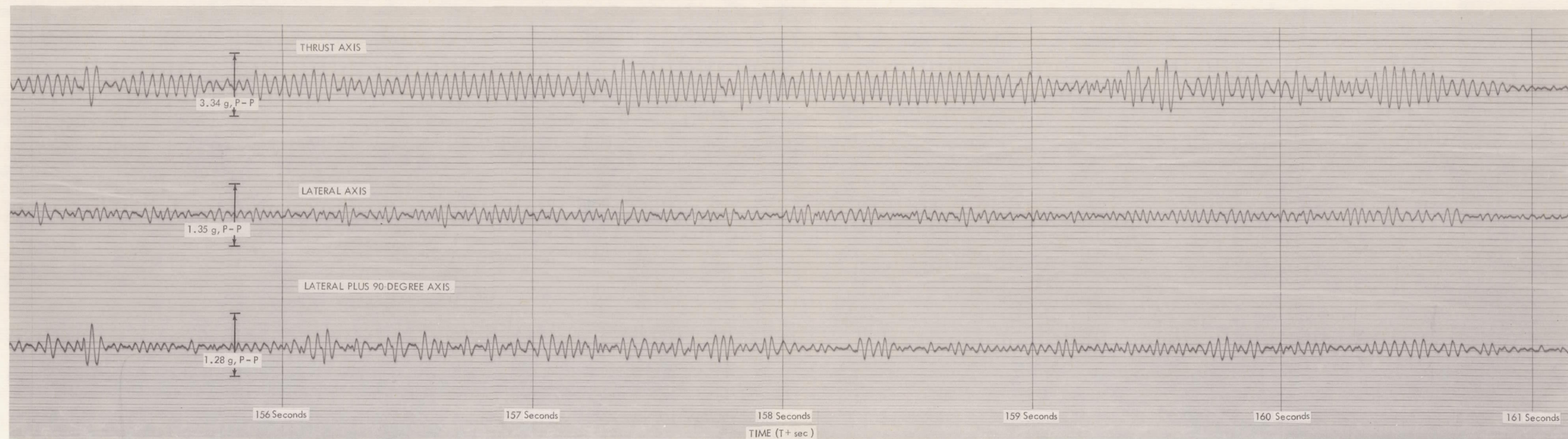
Figure 13—Vibrations at first-stage engine cutoff; instantaneous acceleration versus time; signal filtered with a narrow-band filter. Signal of the 26-cps vibration.
