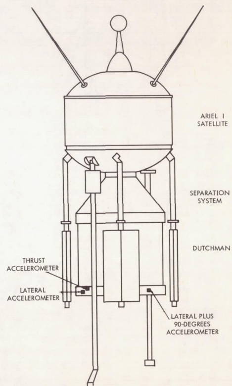
Figure 2—Locations of the accelerometers on the Dutchman.
