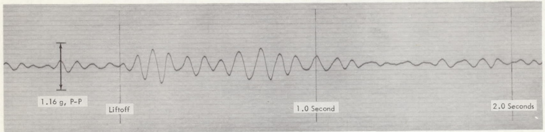
(a) Signal of the 10.5-cps vibration.
