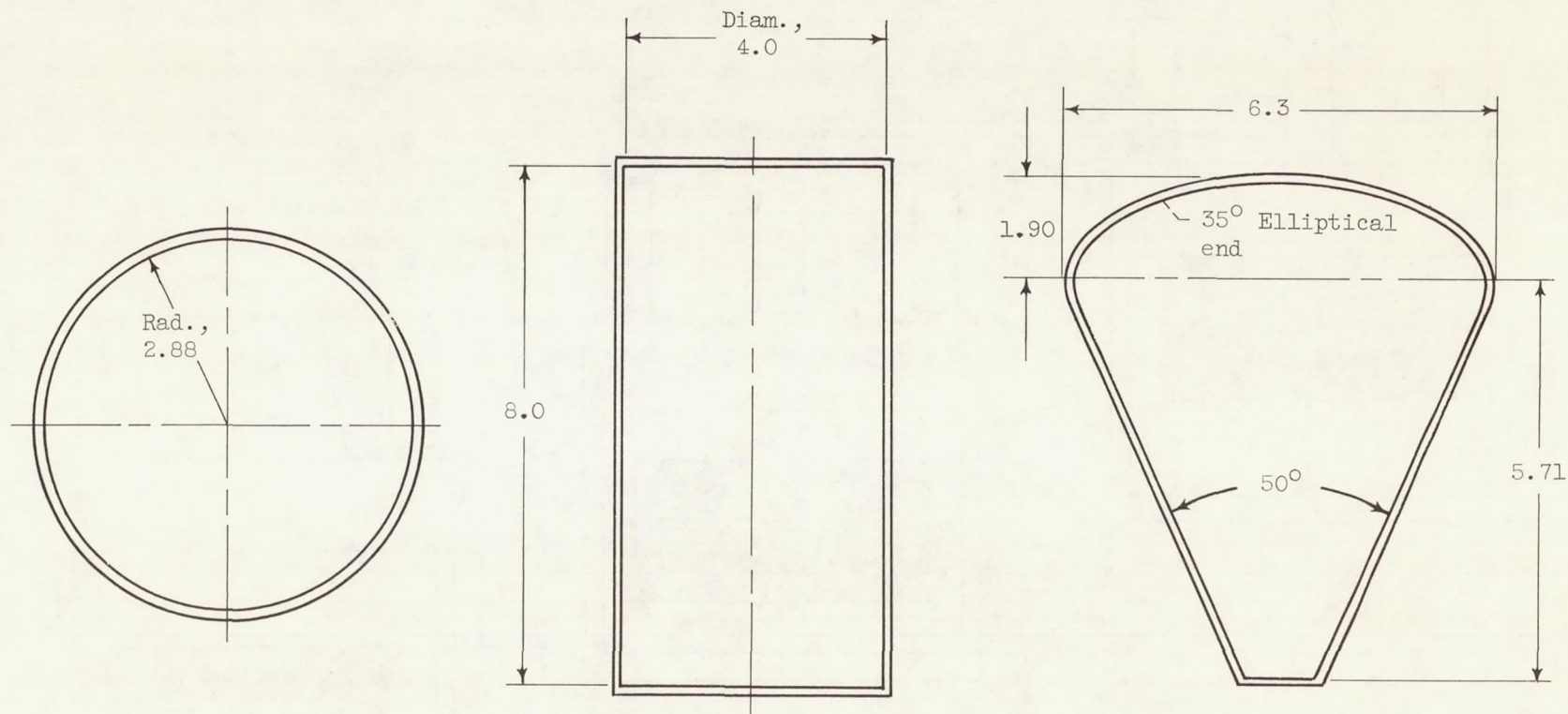
Figure 3. - Schematic diagrams of 100-milliliter glass tanks used in experimental study showing nominal dimensions in centimeters.
