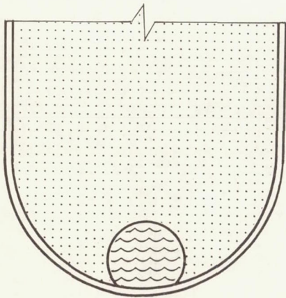
Figure 7. - Typical interface configurations at low fillings in cylindrical tanks with various end shapes.
