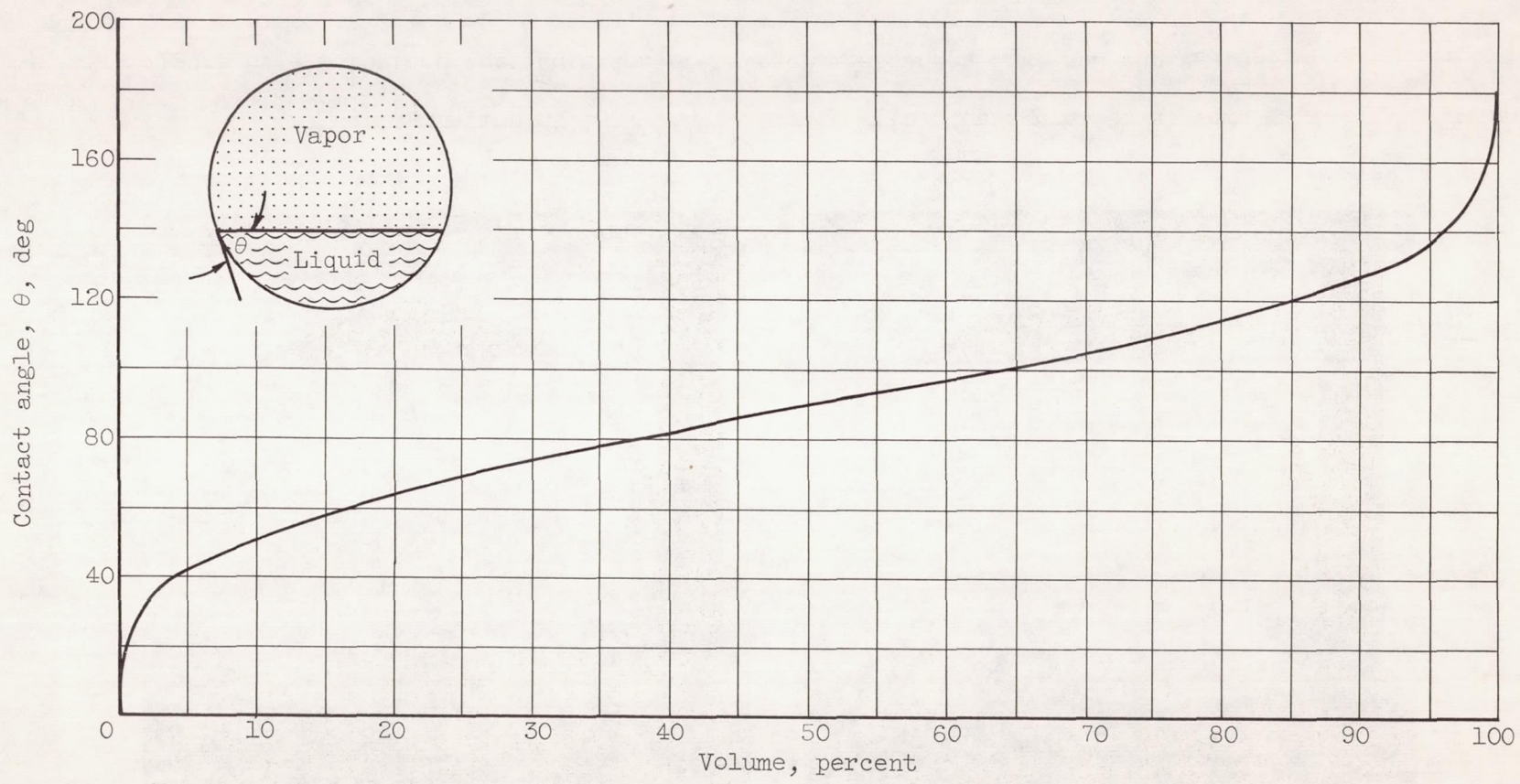
Figure 8. - Contact angle as function of percent of total volume in a sphere.
