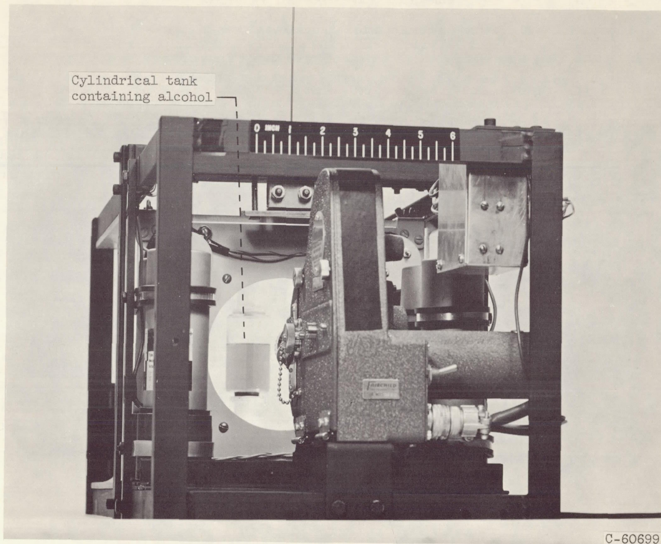
(b) View of experiment tank mounted in light box.
