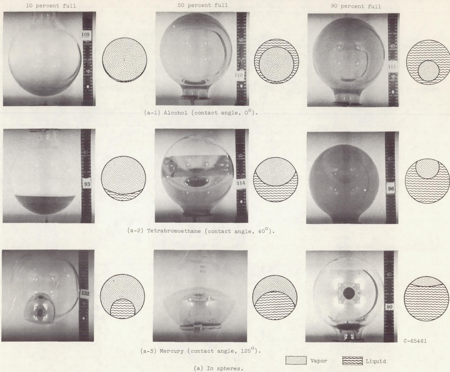
Figure 5. - Configuration of liquid-vapor interface during weightlessness.
