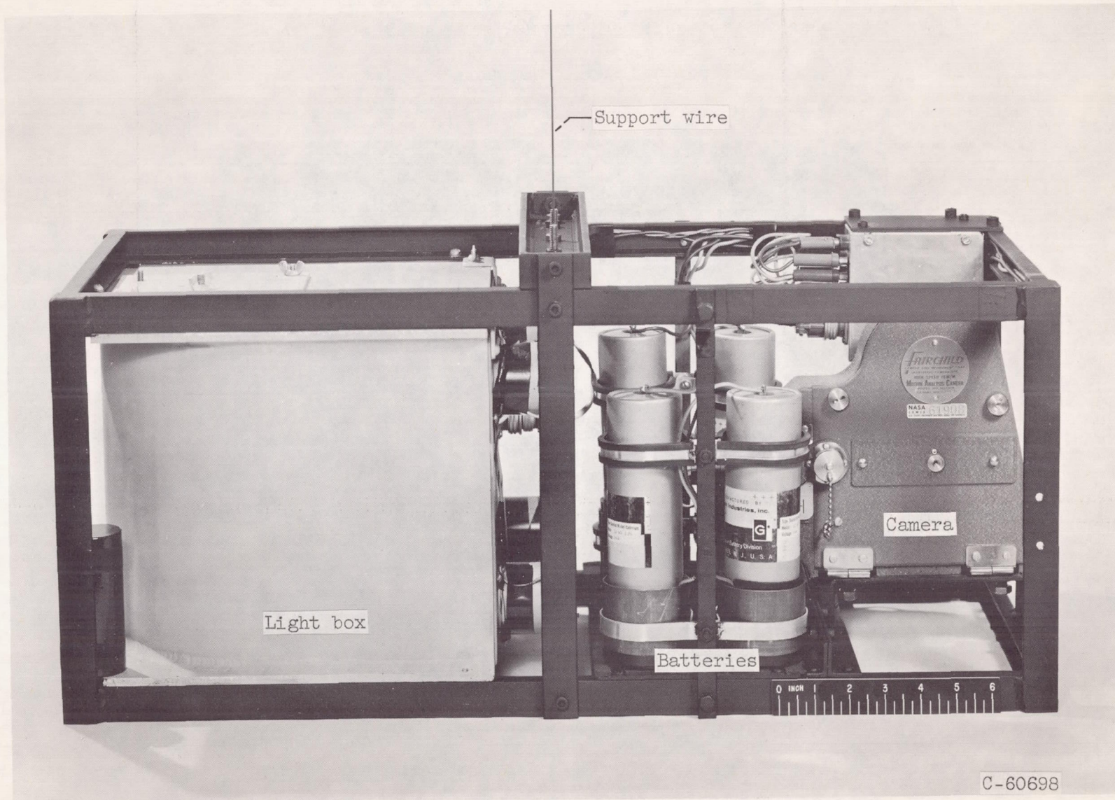
(a) View showing components.
