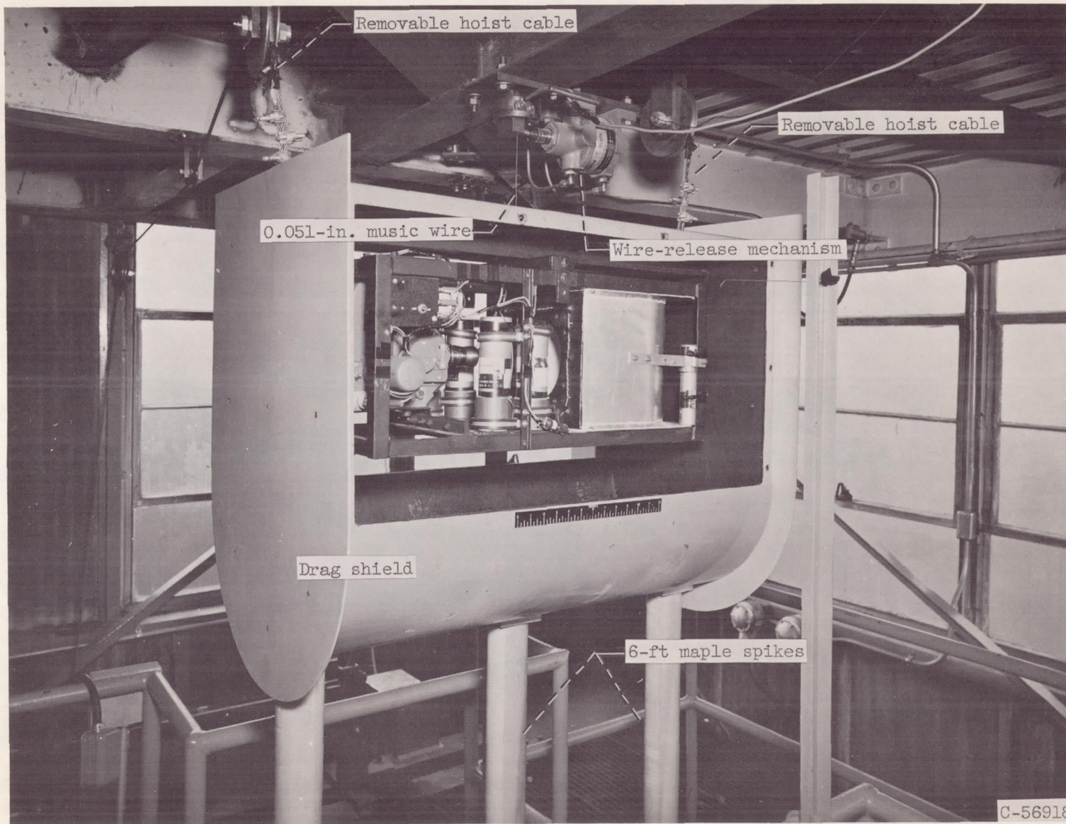
(c) Experiment inside drag shield prior to test drop.
