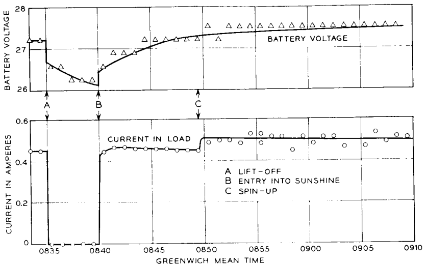
Fig. 10 — Ni-Cd battery voltage and current delivered to canister during launch.
