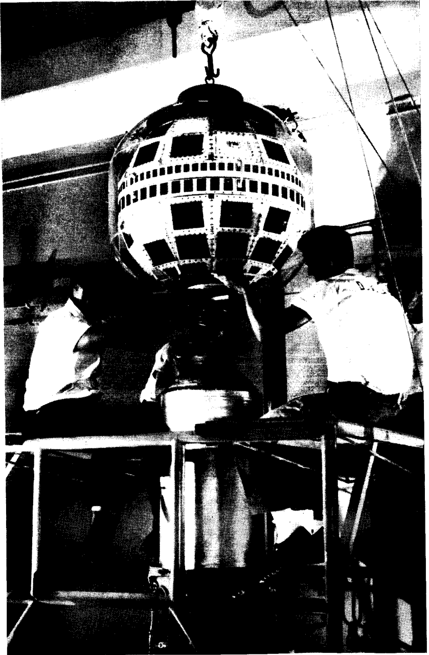
Fig. 1 — Mating the spacecraft to the Delta third stage.
