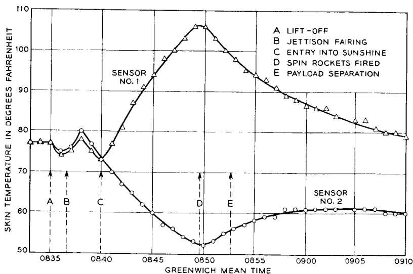
Fig. 9 — Skin temperature variation after lift-off
