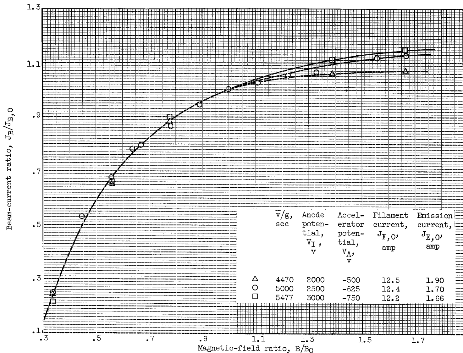
(a) Beam-current ratio as function of magnetic-field ratio.
