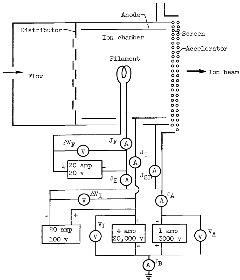
Figure 2. - Wiring diagram of ion thruster.
