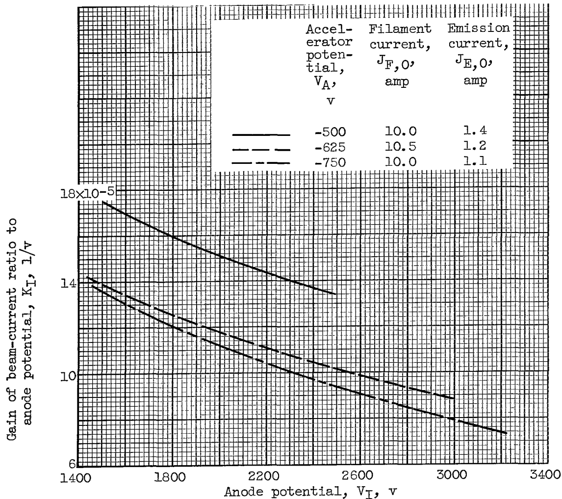
(c) Gain of beam-current ratio to anode potential as function of anode potential.
