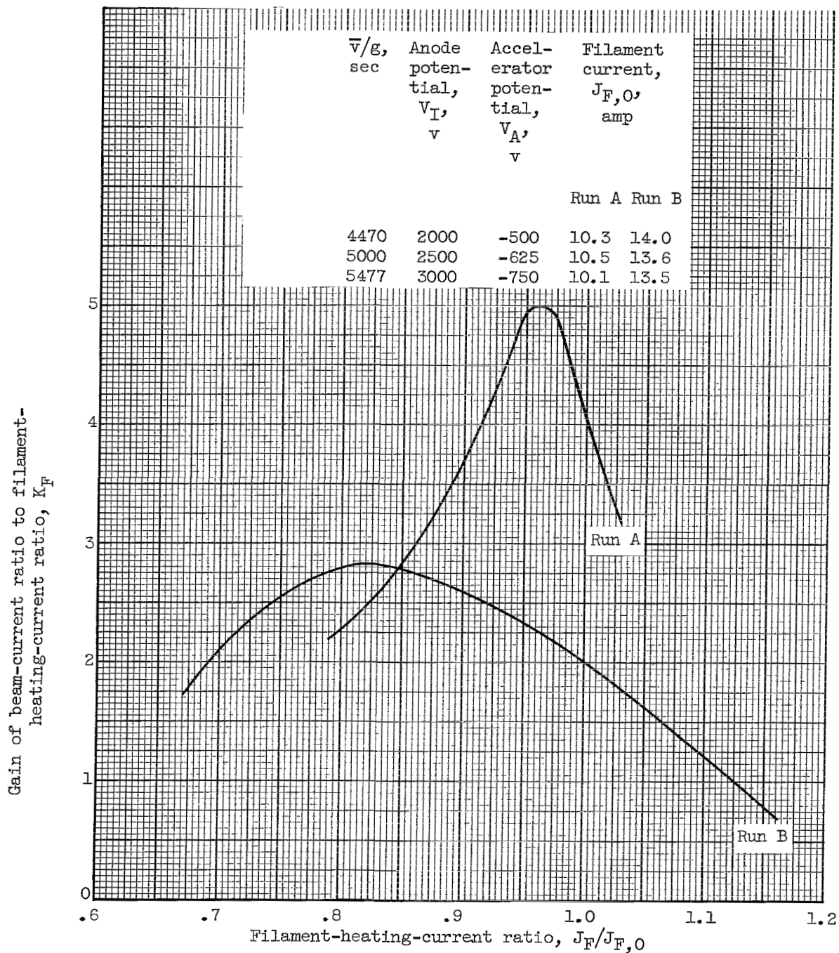
(d) Gain of beam-current ratio to filament-heating-current ratio as function of filament-heating-current ratio for two different filaments.
