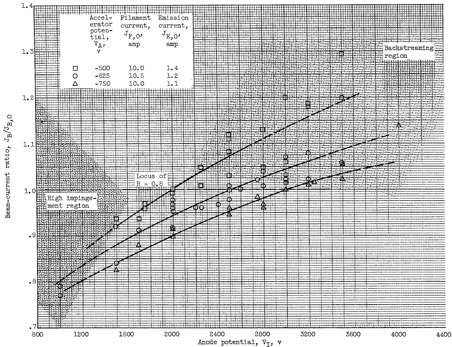
(a) Beam-current ratio as function of anode potential.
