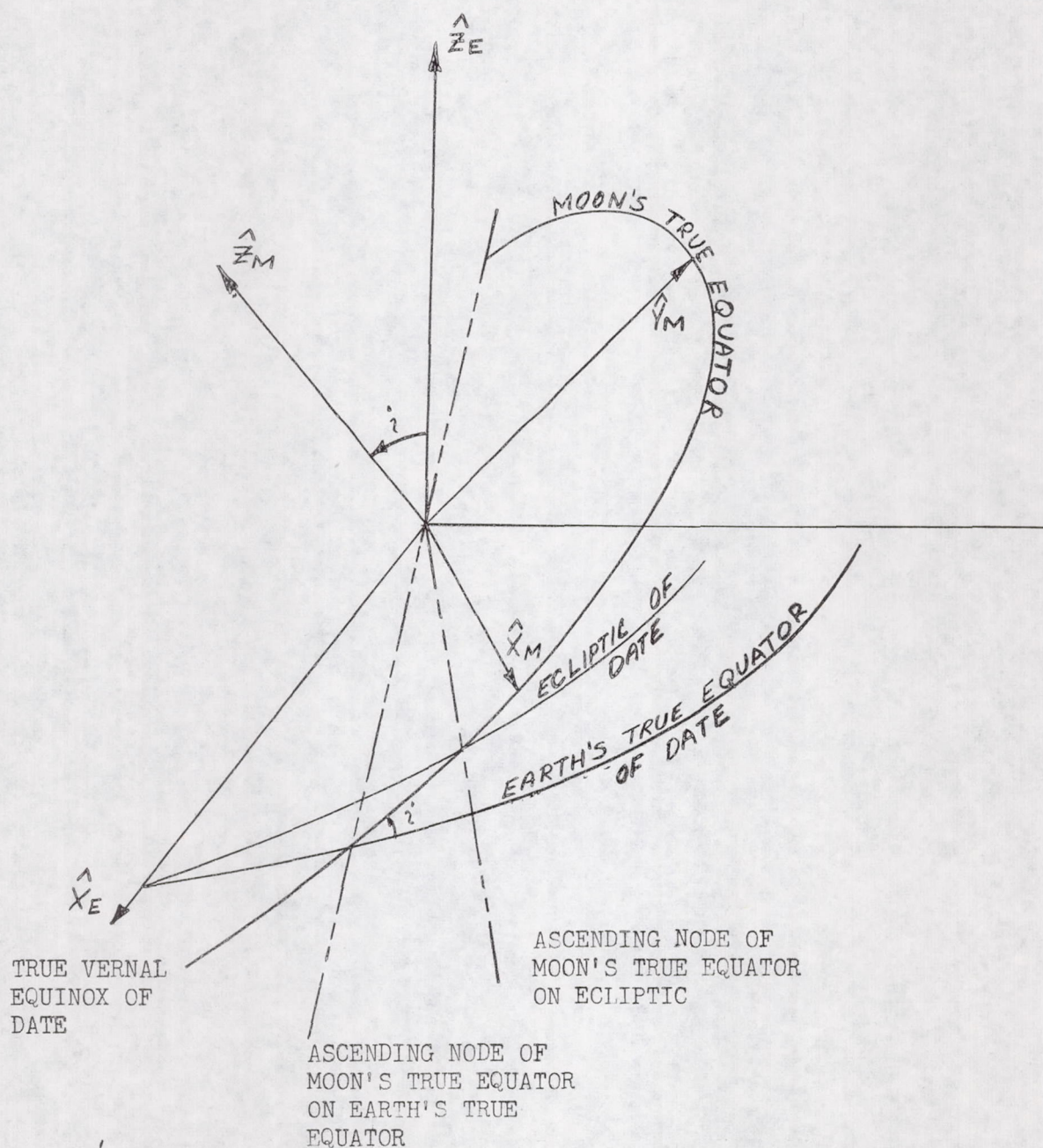
FIGURE VII LIBRATION ANGLES
