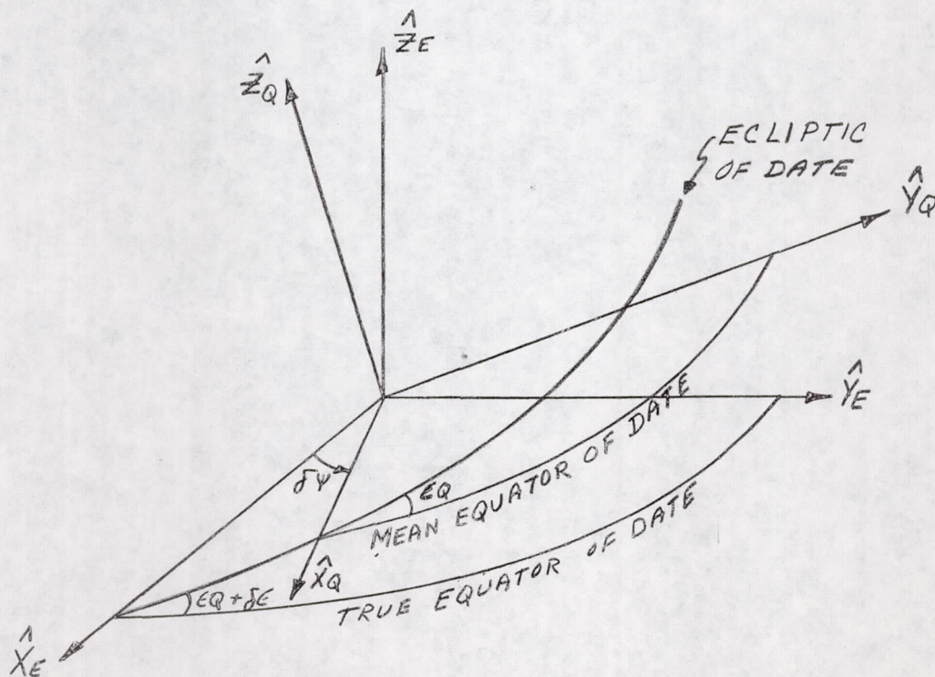
FIGURE VI NUTATION ANGLES
