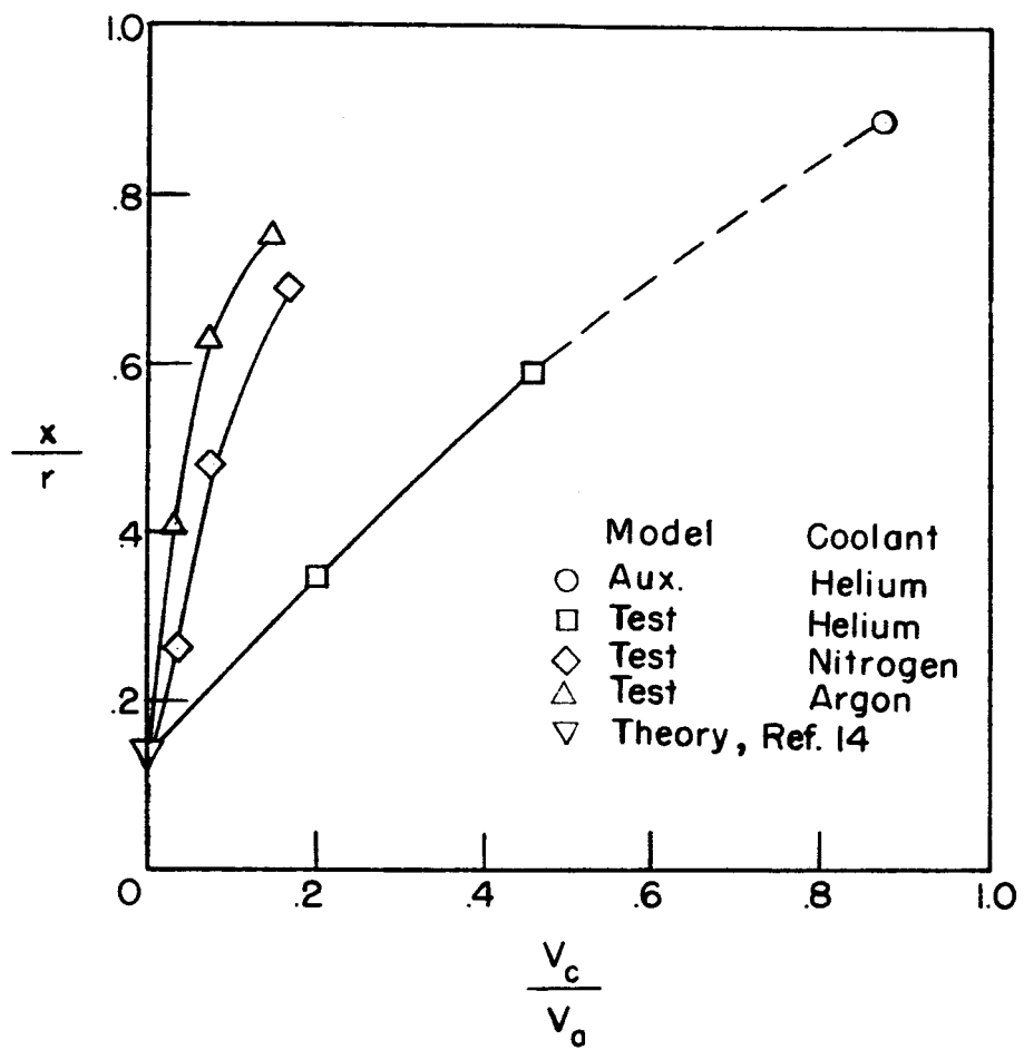
Figure 6.- Shock standoff as a function of volumetric flow.
