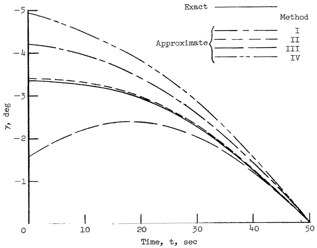
(b) V_d = 20,000 ft/sec.
