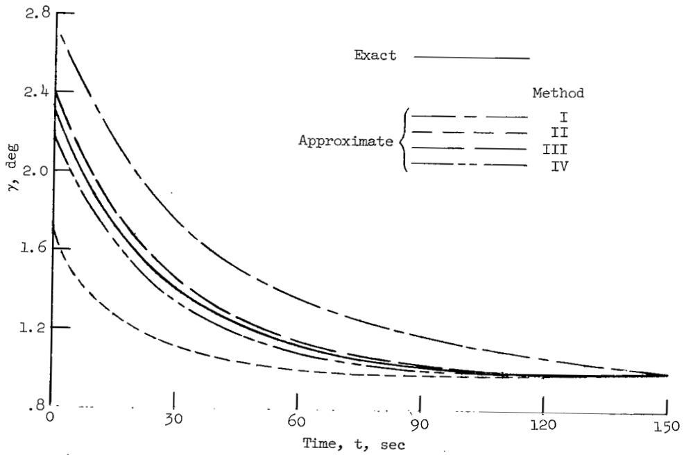
(b) V_d = 26,000 \text{ ft/sec} ; \gamma_d = 1^\circ ; C_L = -0.5 .
