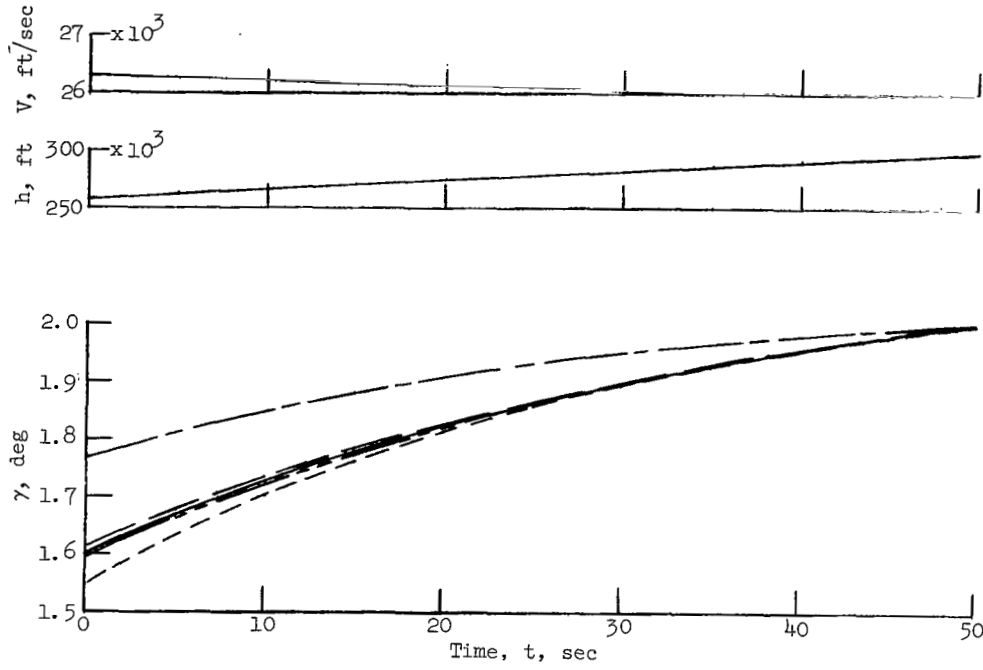
(c) V_d = 26,000 ft/sec; \gamma_d = 2^\circ ; C_L = 0.5 .
