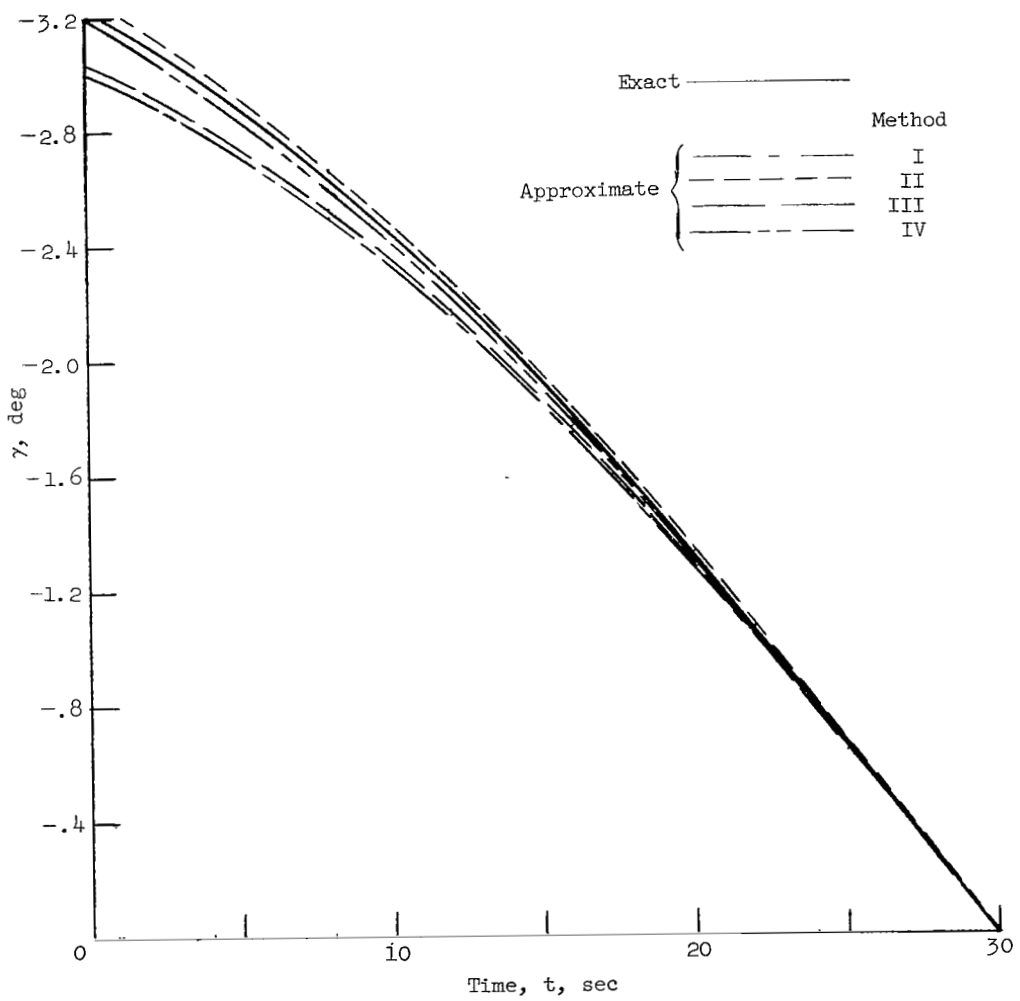
(c) V_d = 26,000 ft/sec; C_L = 0.5 .
