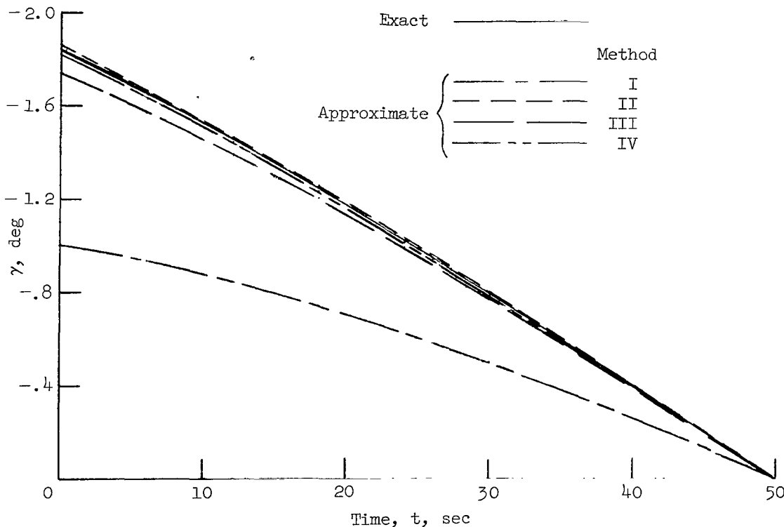
(a) V_d = 30,000 ft/sec; \gamma_d = 0^\circ ; C_L = 0.5 .
