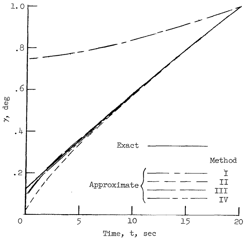
(e) V_d = 30,000 \text{ ft/sec} ; \gamma_d = 1^\circ ; C_L = 0.5 .
