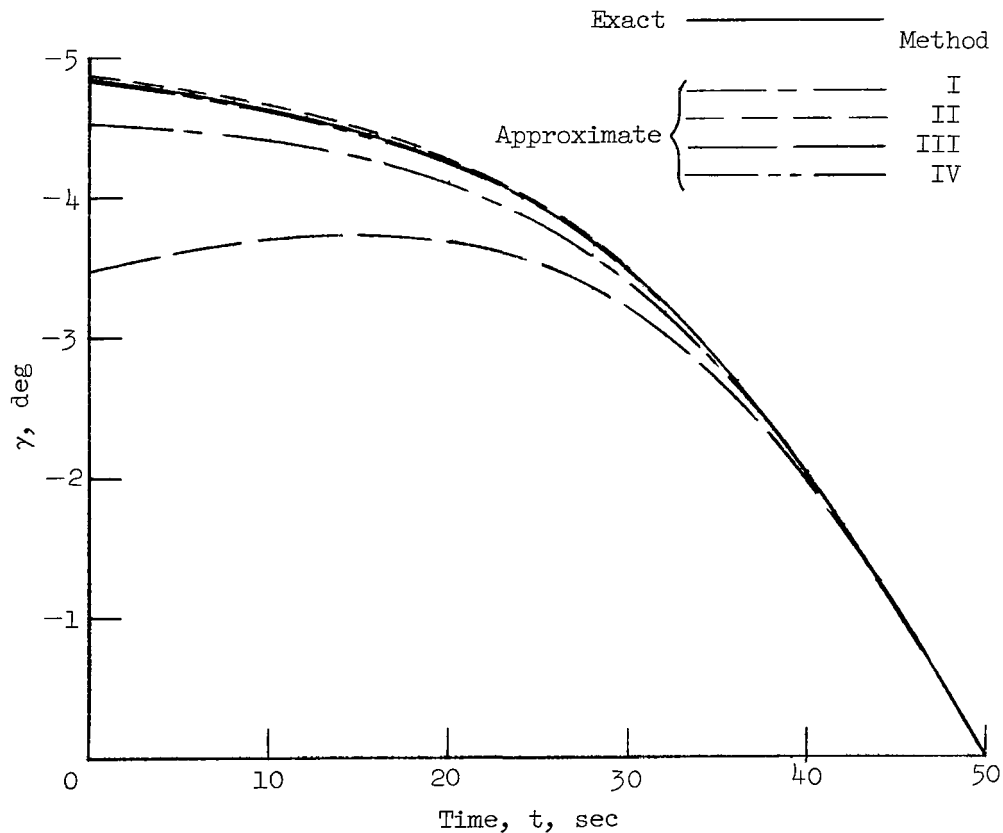
(a) V_d = 26,000 ft/sec.
