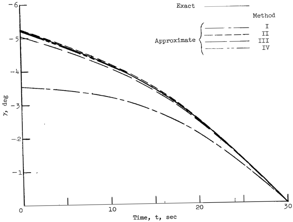
(a) V_d = 40,000 ft/sec; C_L = 0.5 .
