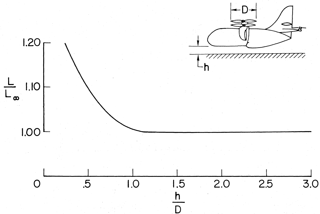
Figure 3.- Effect of ground proximity on lift of the XC-142A model.
