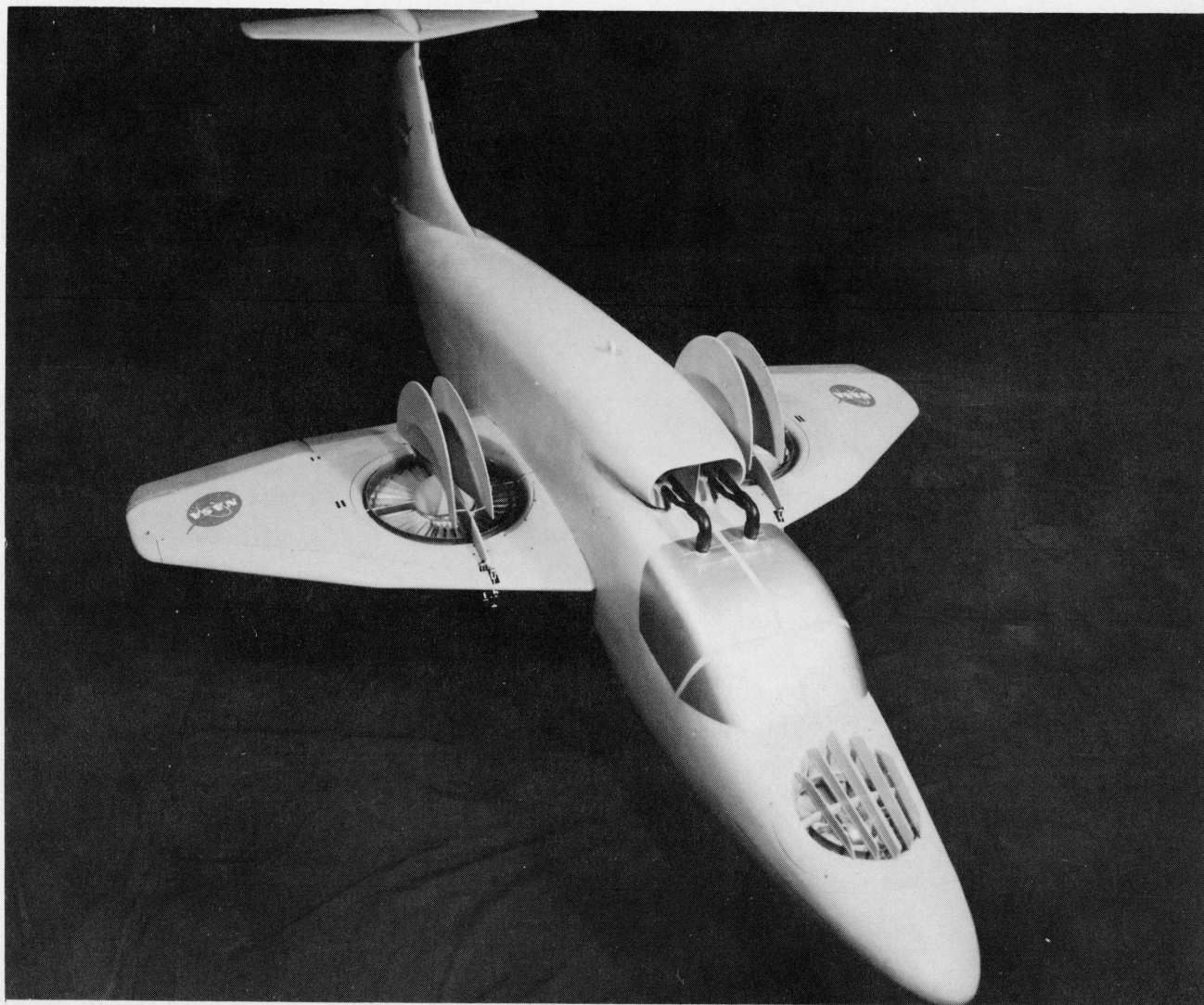
(a) View of model showing fan inlets.
