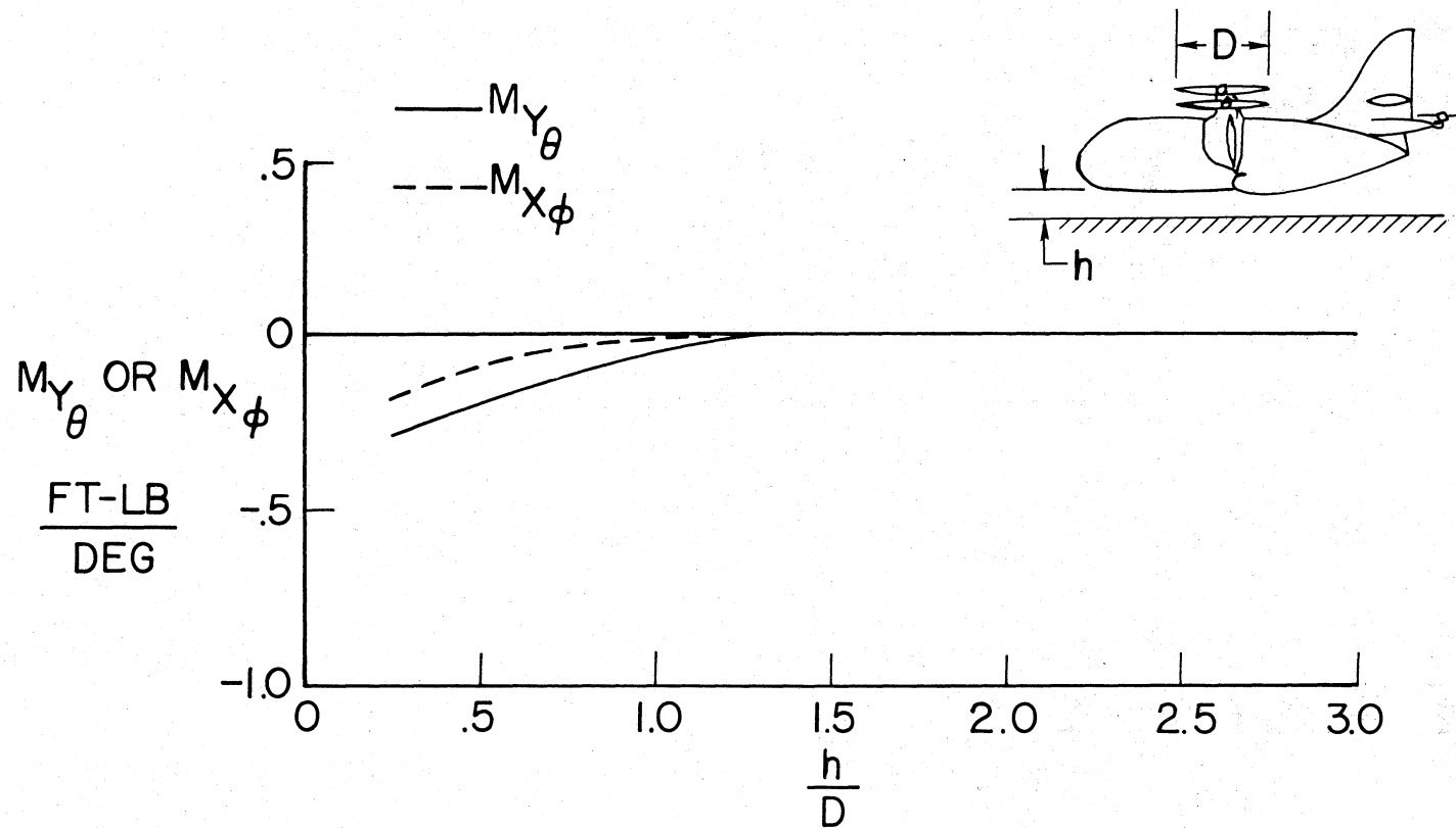
Figure 4.- Effect of ground proximity on static stability of the XC-142A model in hovering flight.
