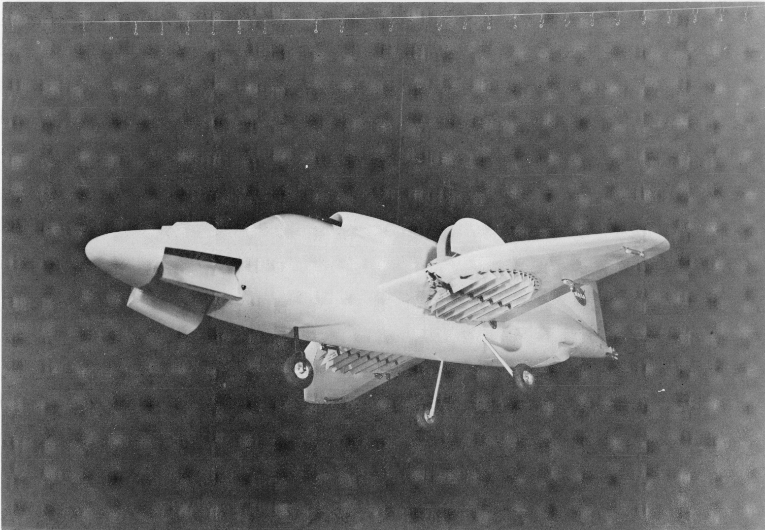
(b) View of model showing fan exit vanes.
