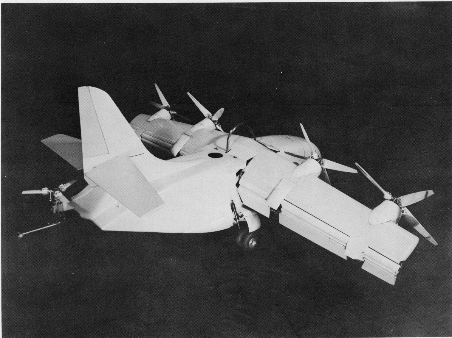
Figure 1.- Photograph of the 1/9-scale XC-142A flying model.
