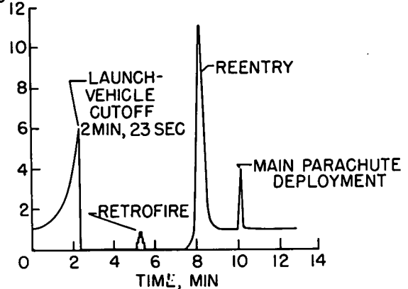
FIGURE 2-6. Acceleration time history for MR-4 flight.
