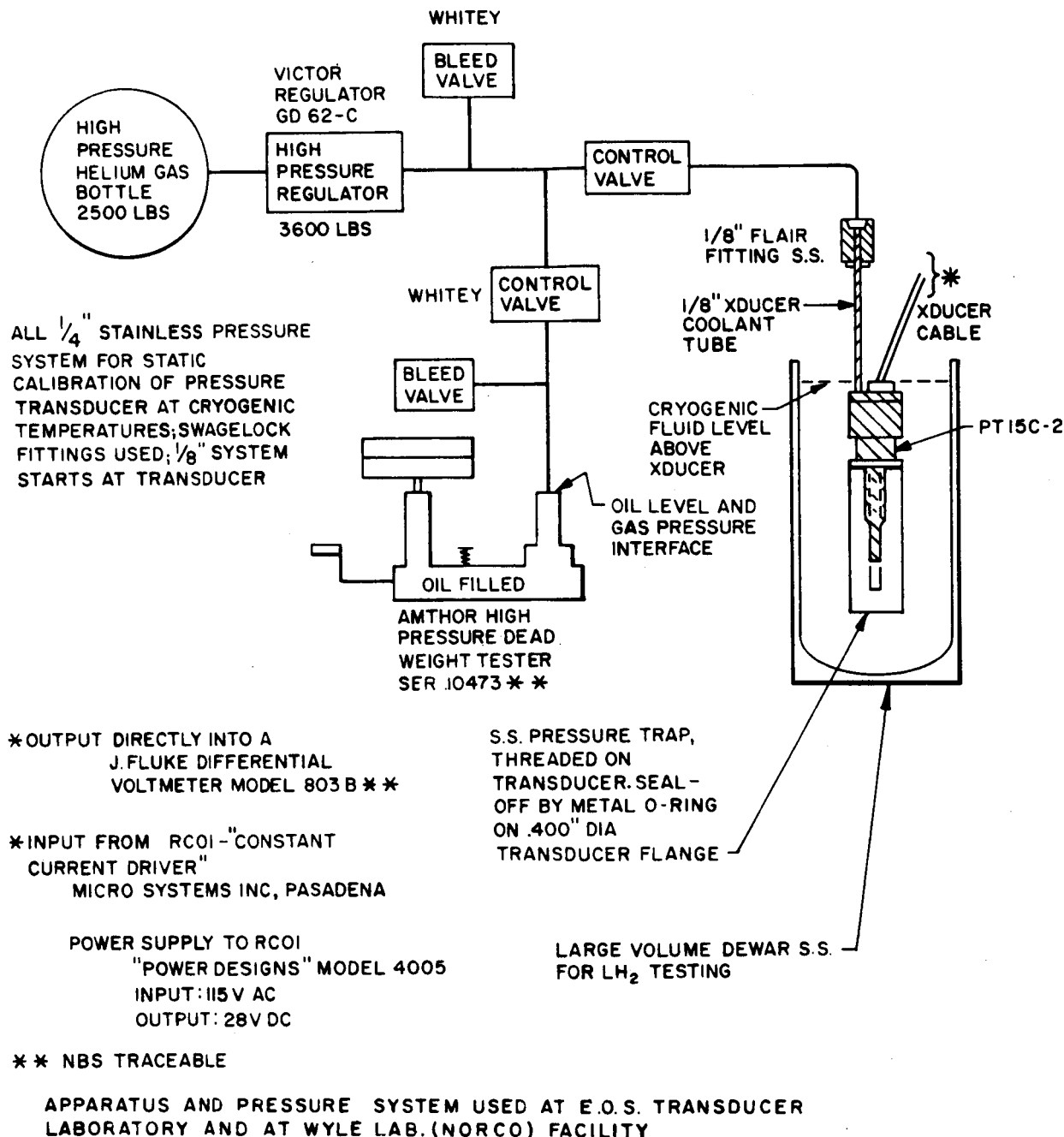
FIG. 10 LABORATORY AND FIELD TEST APPARATUS AND PRESSURE SYSTEM
