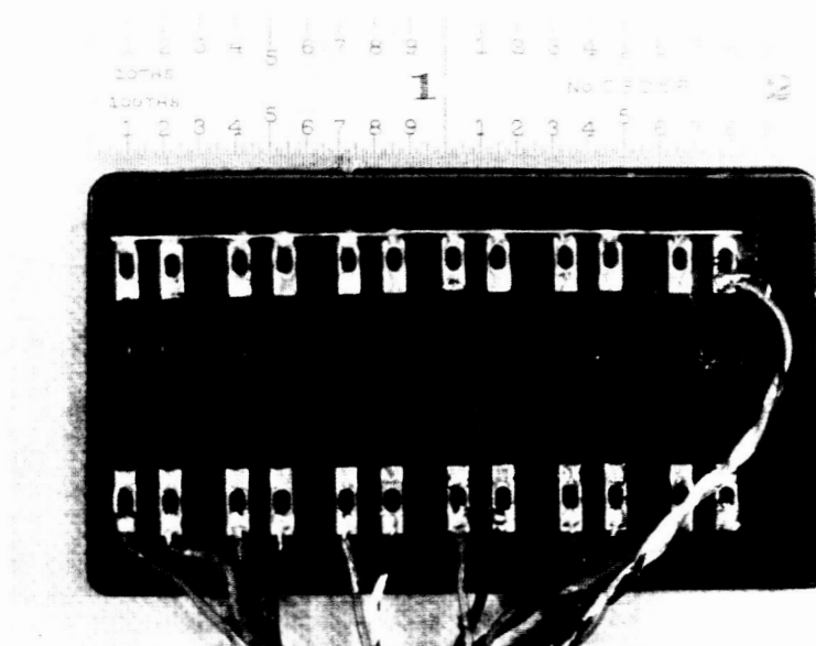
FIG. 4 FOUR-ACTIVE ARM SILICON CHIPS ON 304 SS, SOME SILICON CHIPS BONDED, SOME SUSPENDED OFF THE METAL BAR
