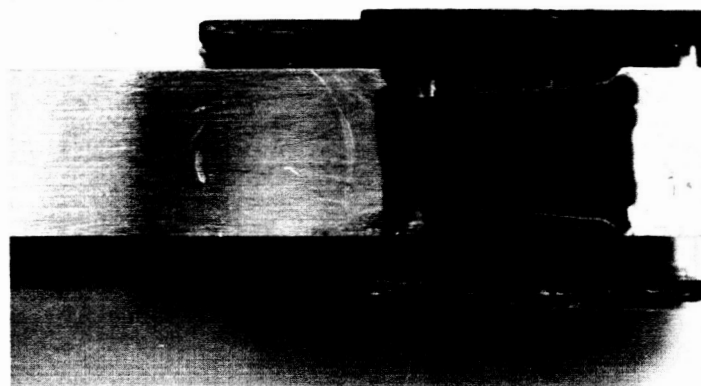
FIG. 5 MULTIPLE ELEMENT SILICON CHIP MOUNTED ON INVAR CONSTANT STRESS BEAM
