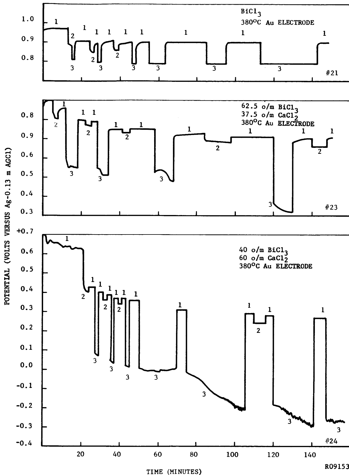
FIGURE 9. \text{BiCl}_3 REDUCTION. EFFECT OF DILUENTS
