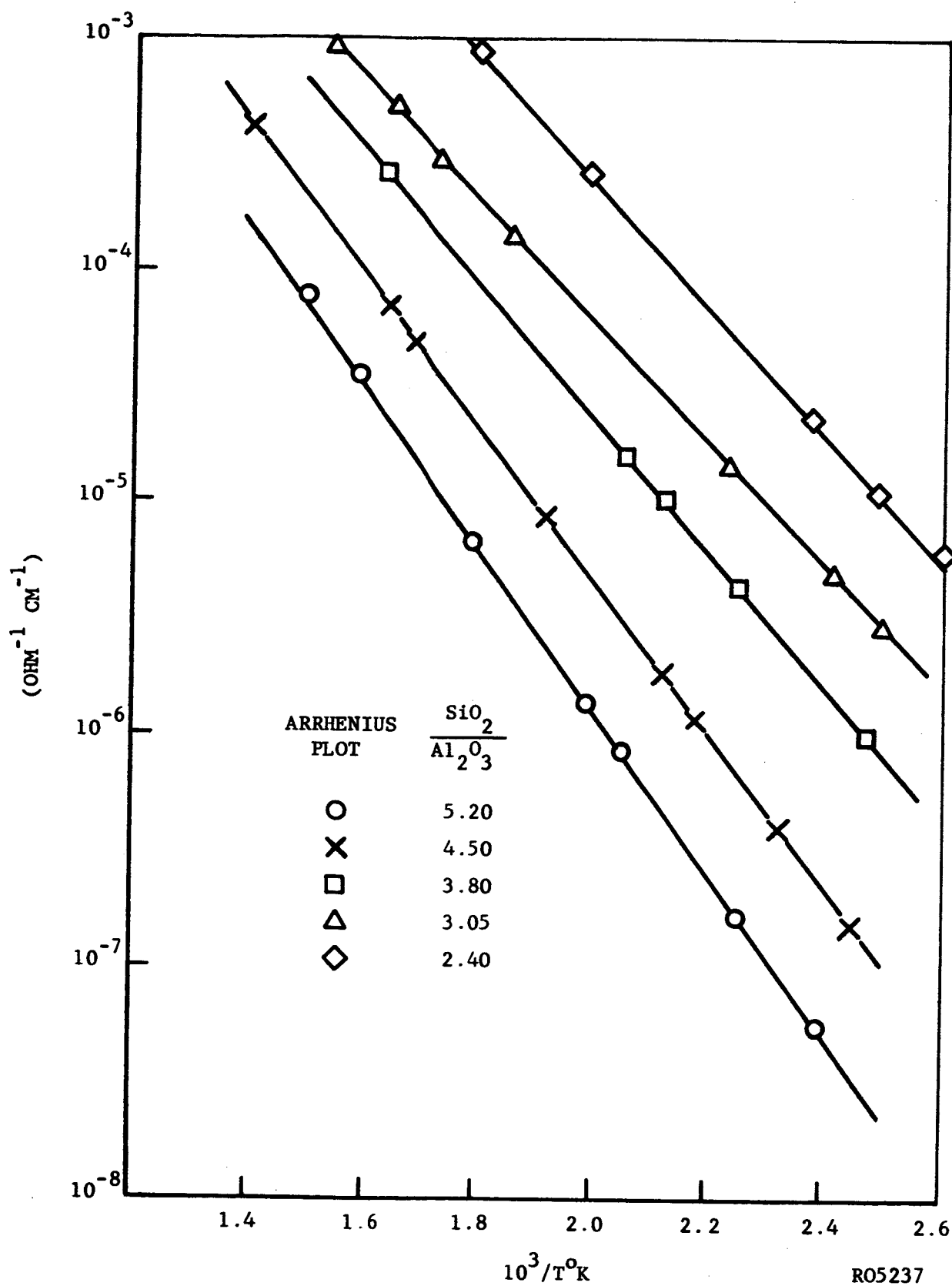
FIGURE 2. CONDUCTIVITY OF THE X-Y ZEOLITE SERIES
