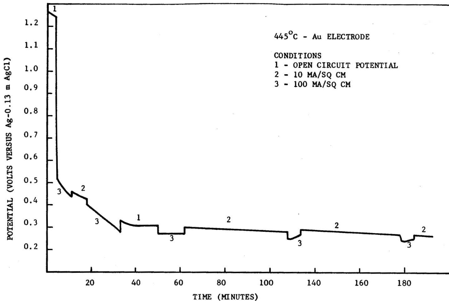
FIGURE 12. CuCl REDUCTION
