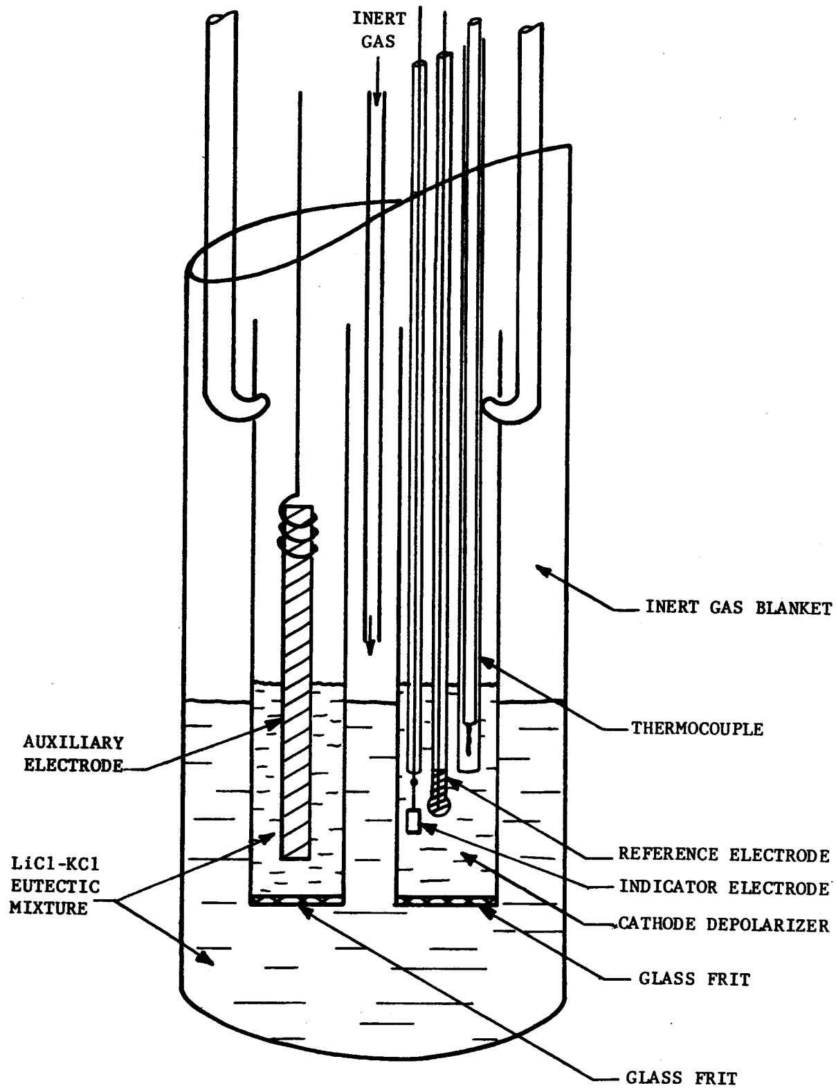
FIGURE 6. ELECTROLYSIS CELL
