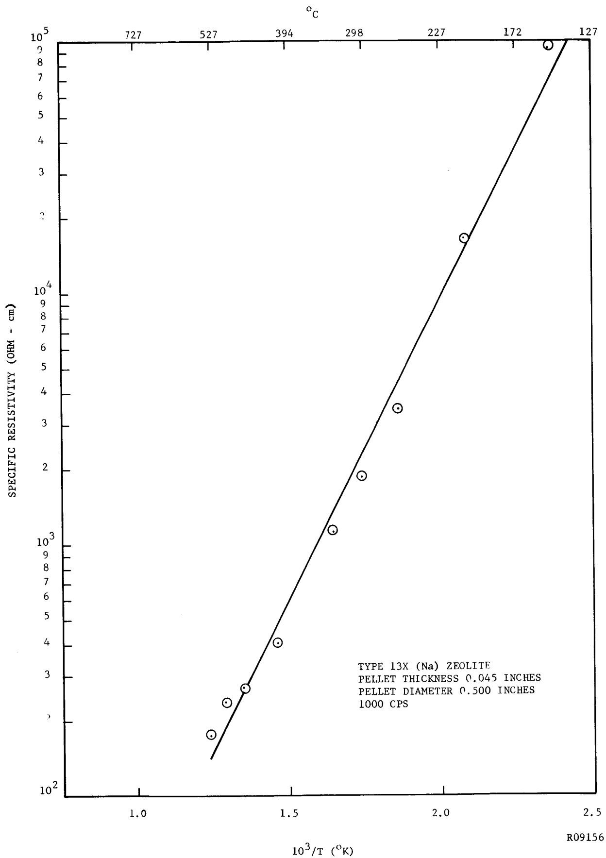
FIGURE 19. ARRHENIOUS PLOT
