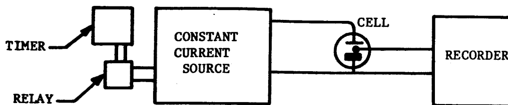
FIGURE 4. BLOCK DIAGRAM OF APPARATUS FOR POLARIZATION STUDIES
