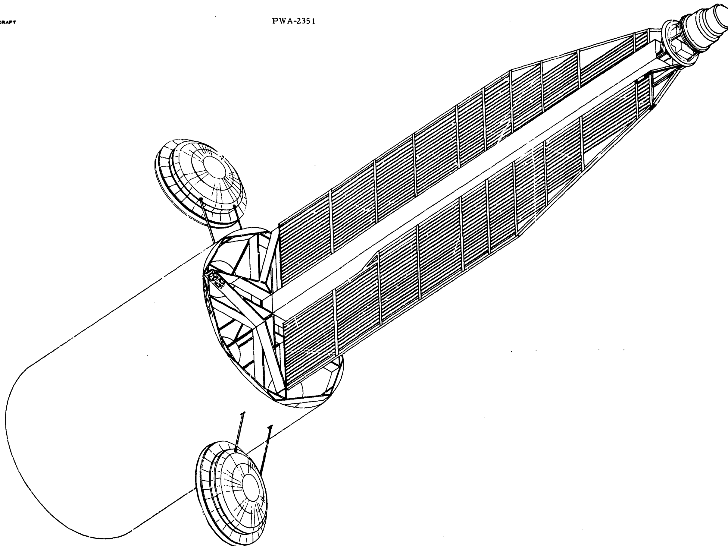
Figure 1 Inflight Powerplant Configuration
