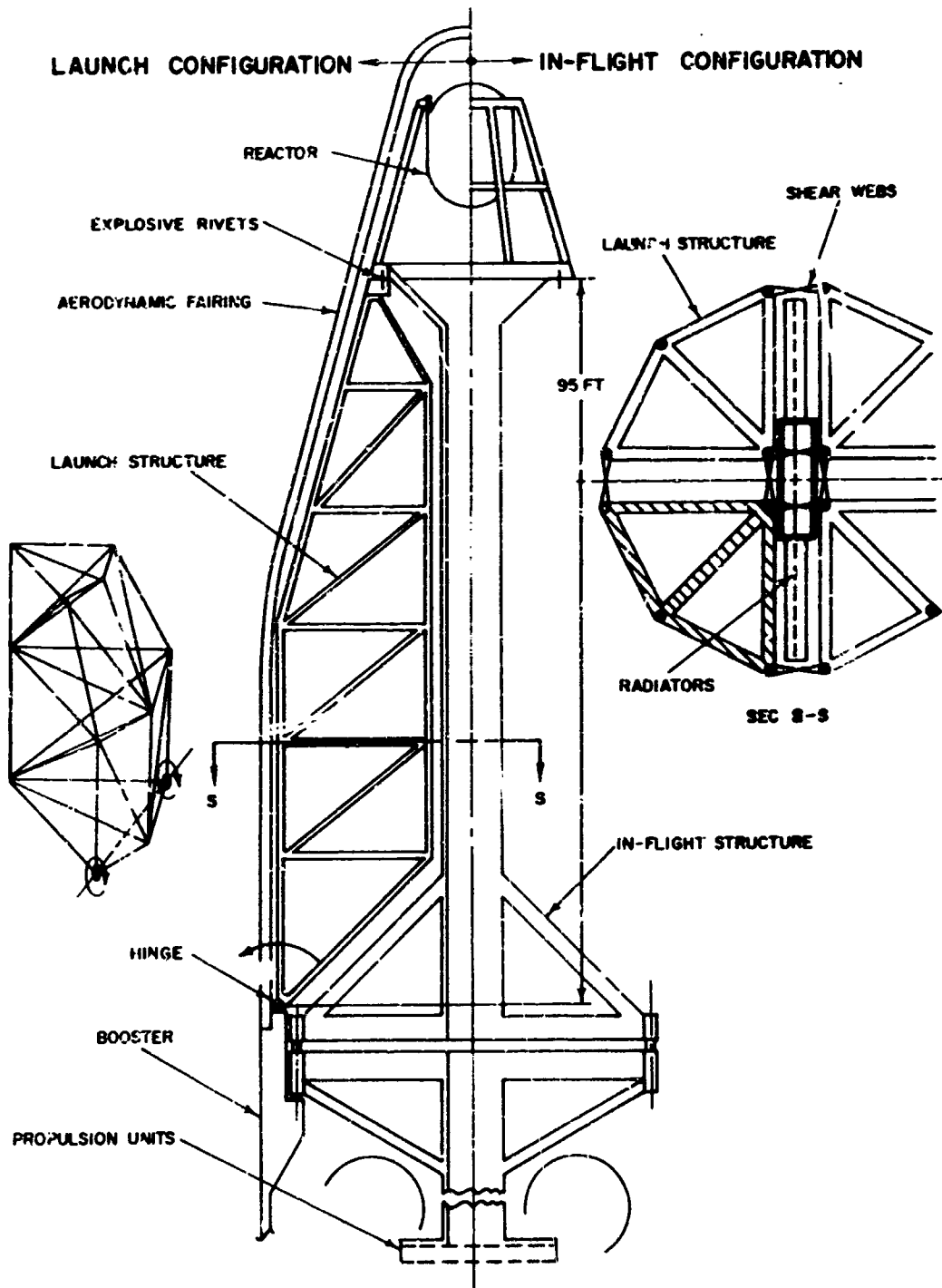
Figure 1-8 Structural Schematic
