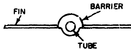
Figure 4-1 Fin-Tube Radiator Design
