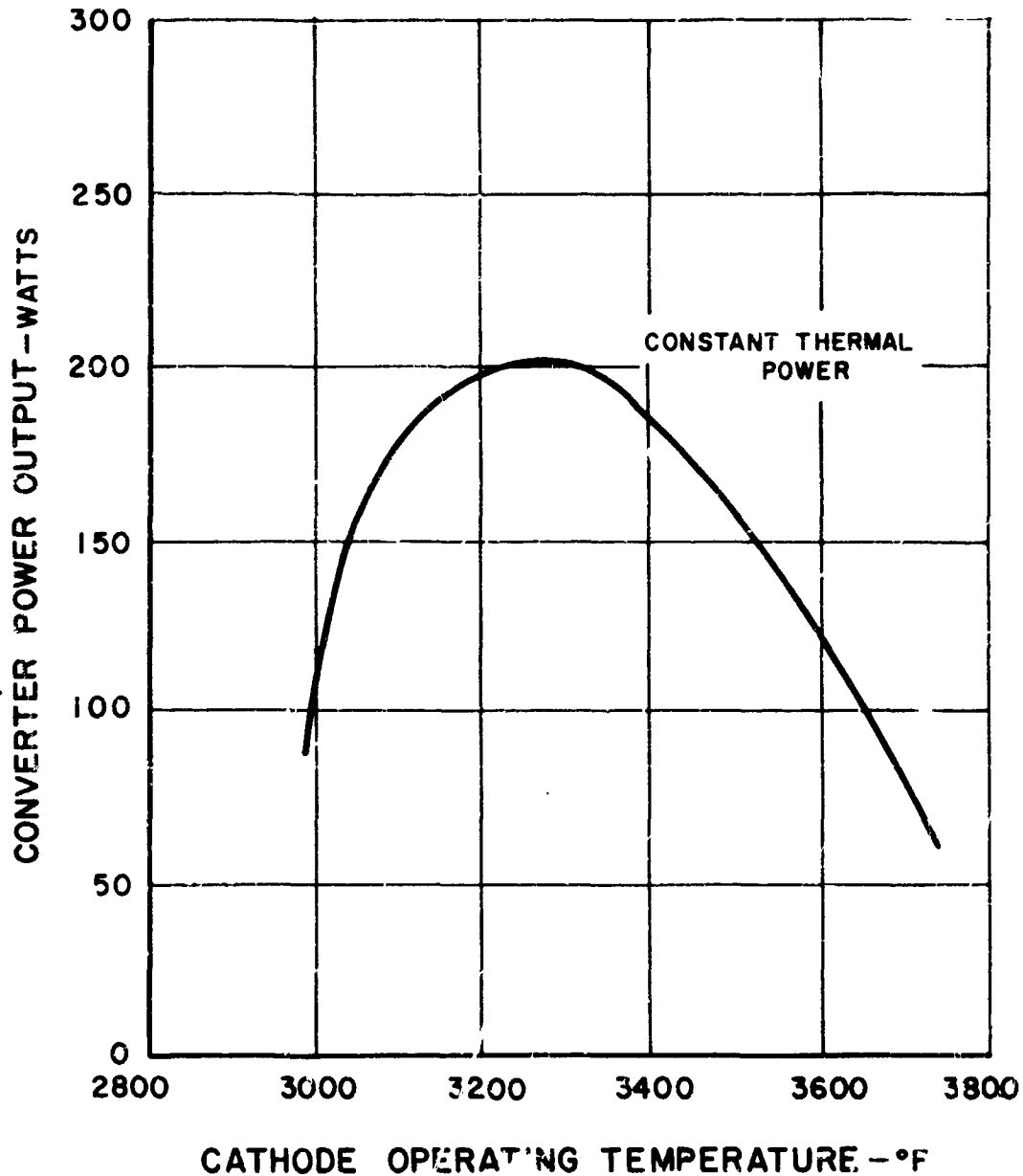
Figure 11 Converter Power vs Cathode Temperature
