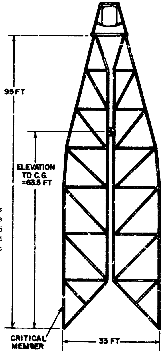
Typical Cross-Section
