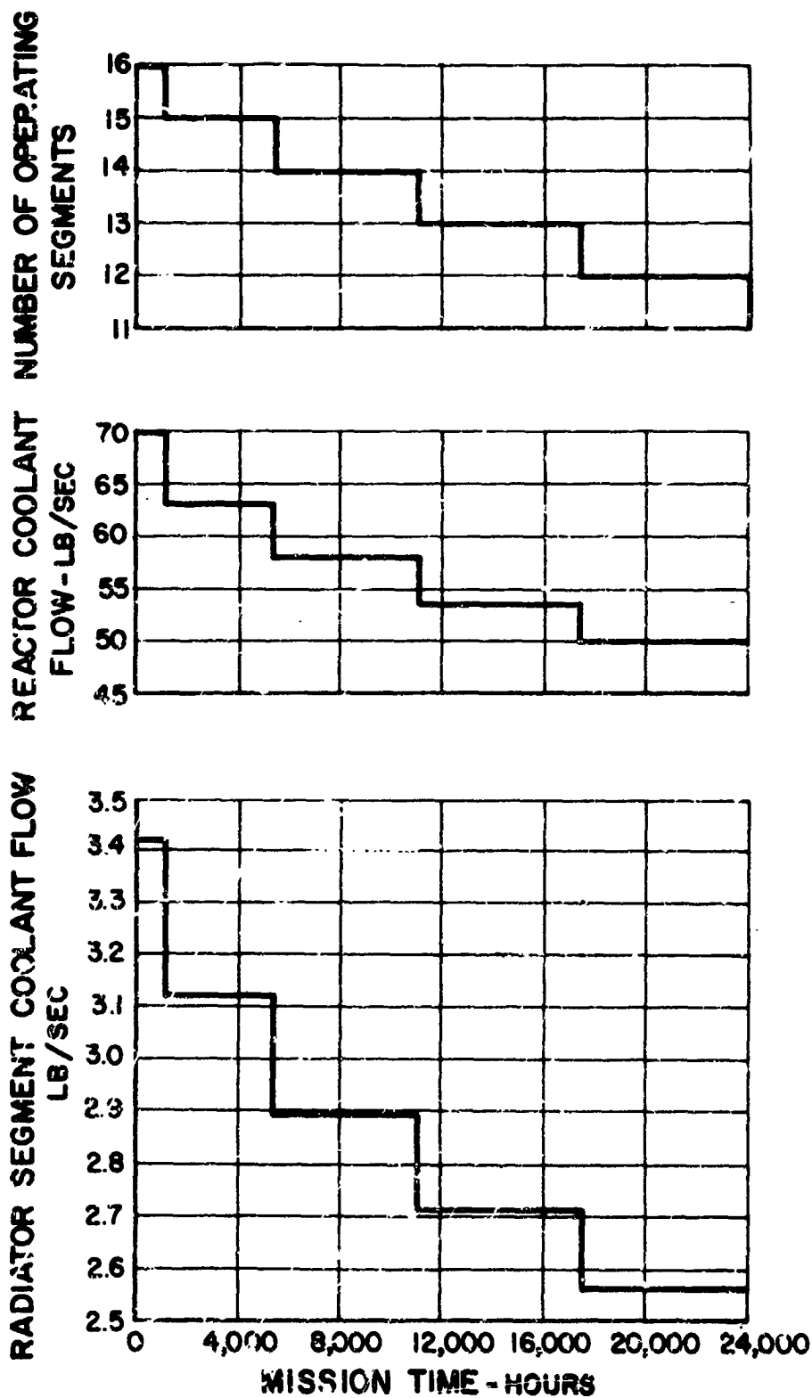
Figure 33 Powerplant Performance during Mission. System Operating Characteristics
