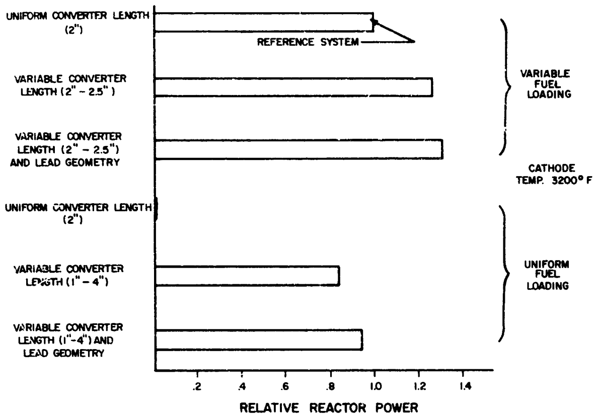
Figure 6-12. Reactor Performance
