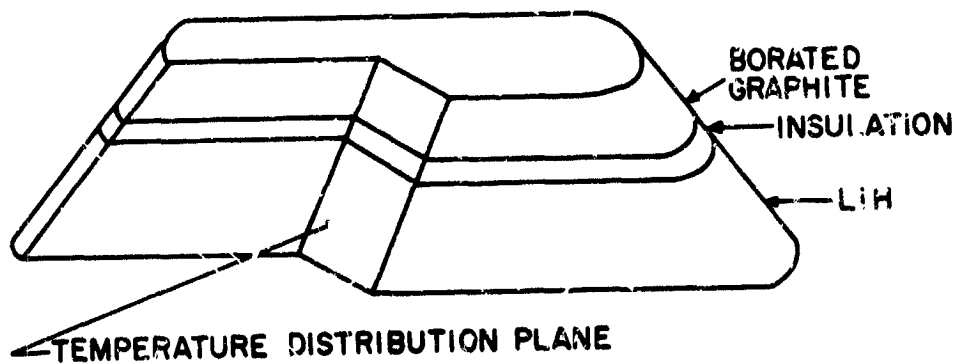
Figure 3-15 Shield Temperature Distribution
