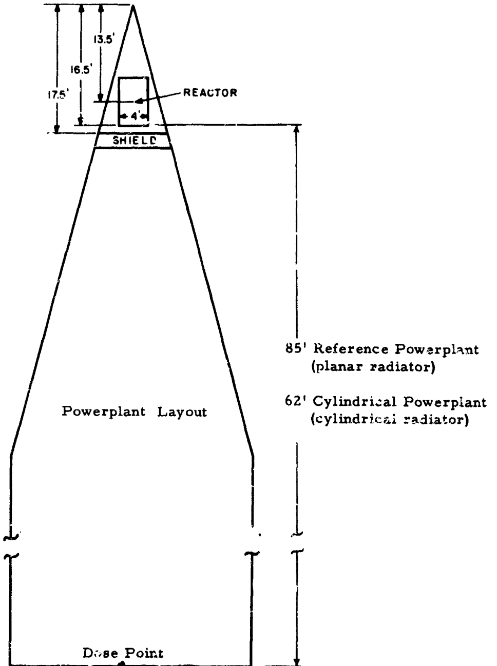
Figure 3-3 Vehicle Layout
