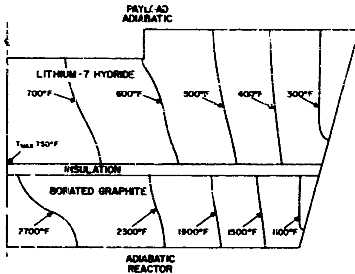
Figure 2-16 Cylindrical Powerplant Shield Temperature Distribution
