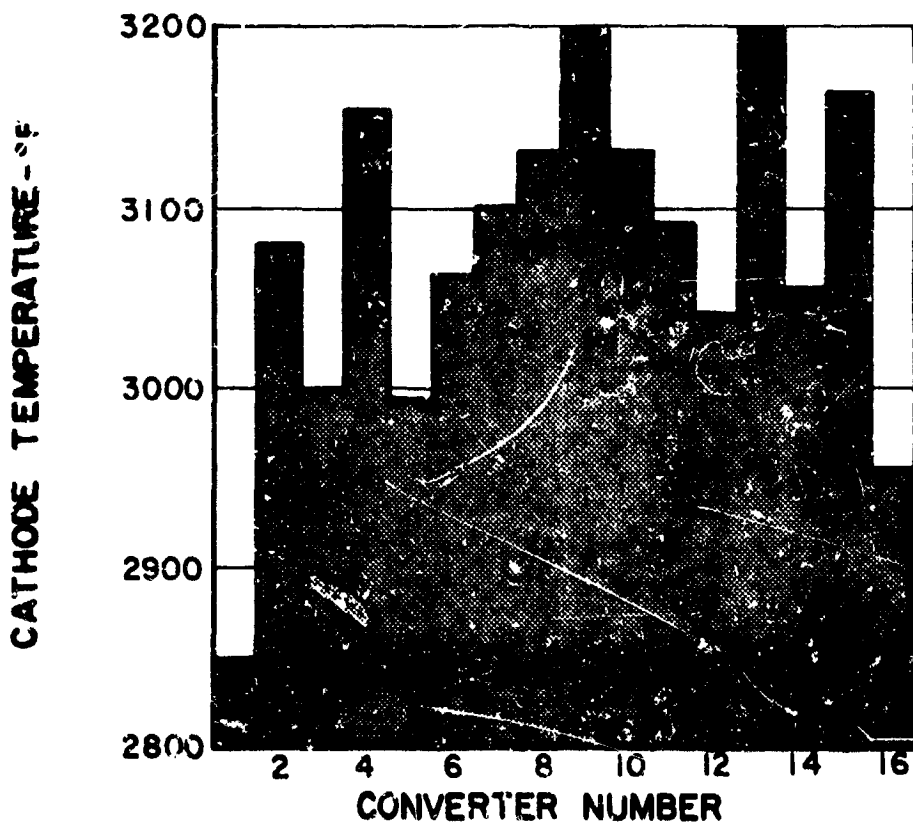
Figure 18 Cathode Temperature
