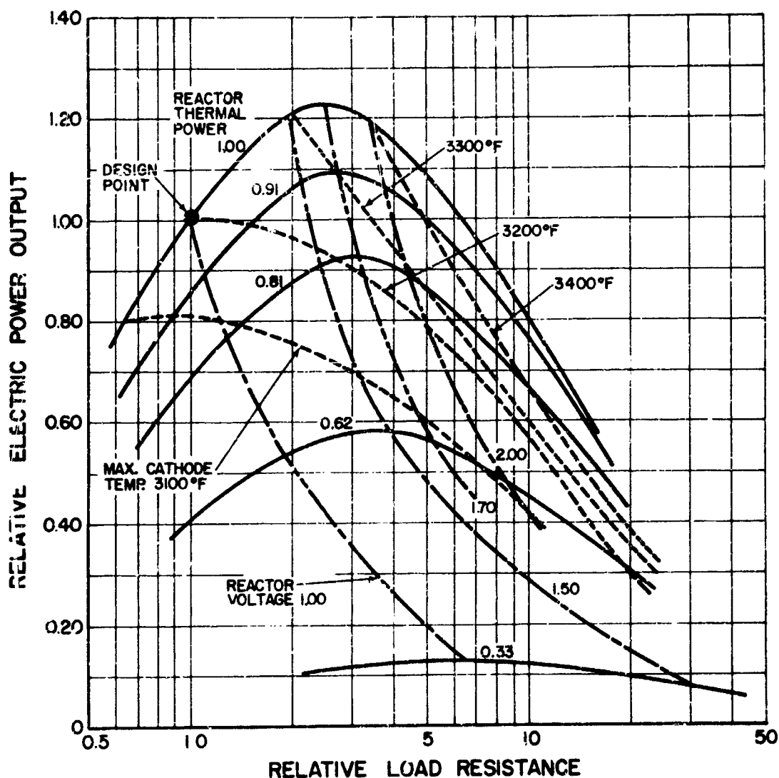
Figure 23 Reactor Performance
