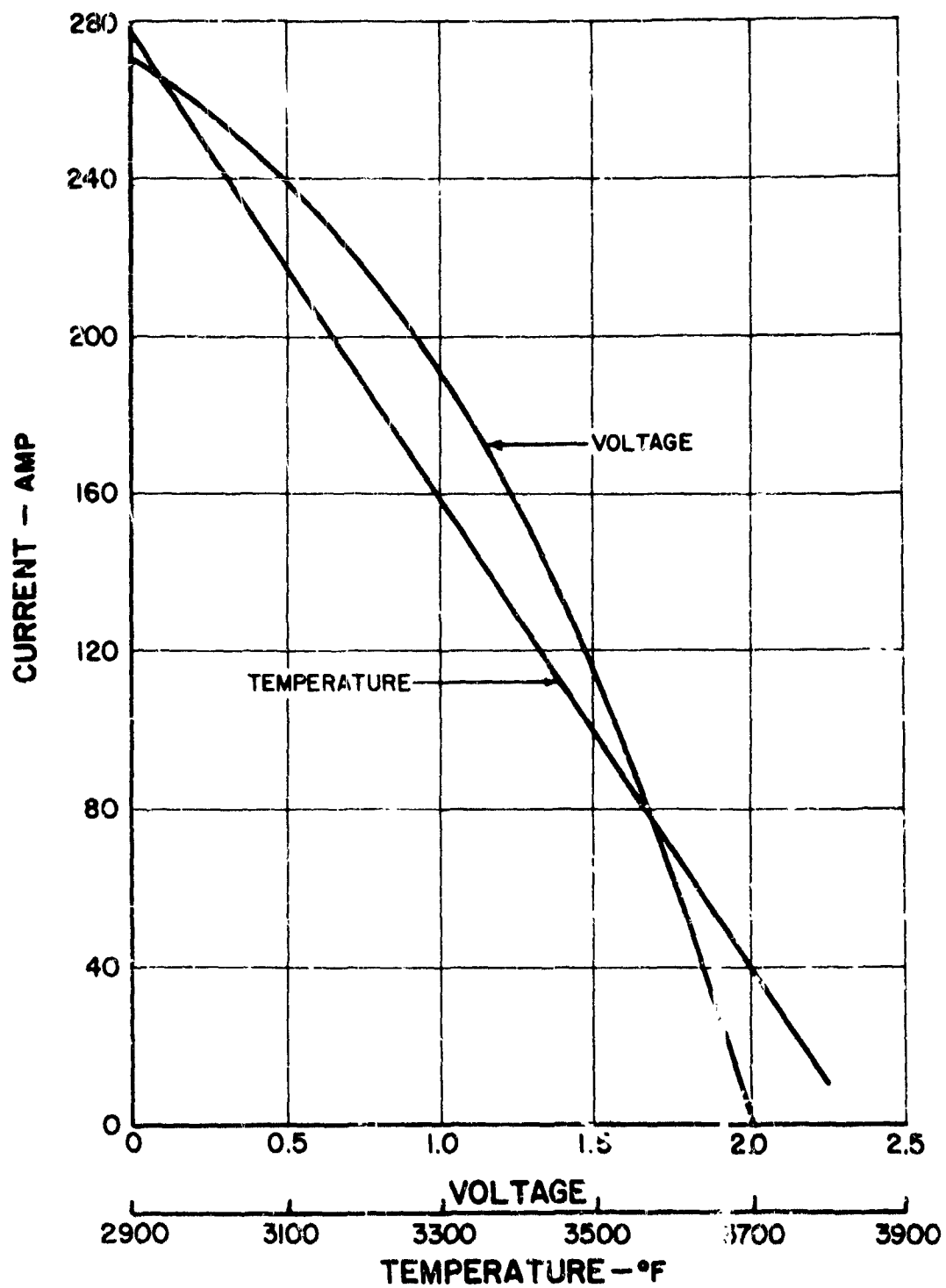
Figure 13 Current-Voltage Characteristics
