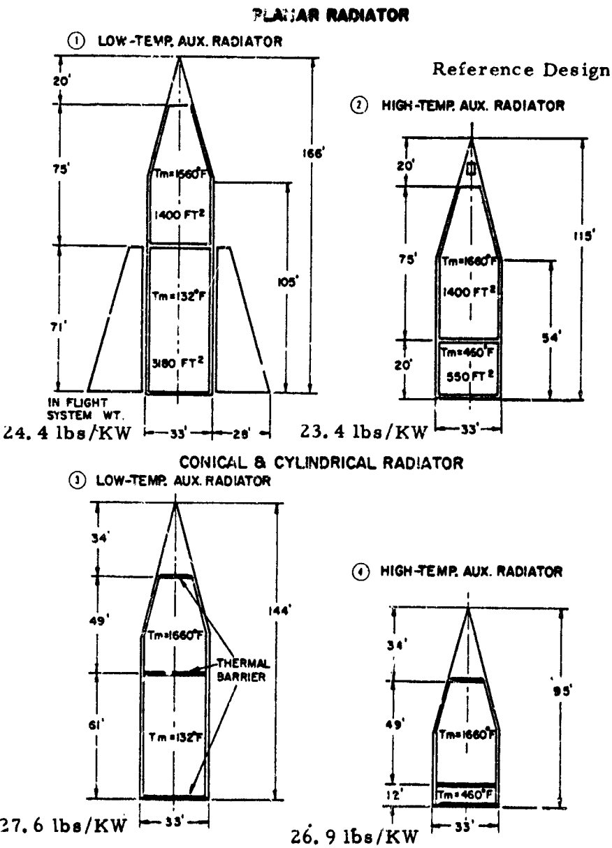
Figure 2-1 Radiators for 3.25-MW Thermionic Powerplant
