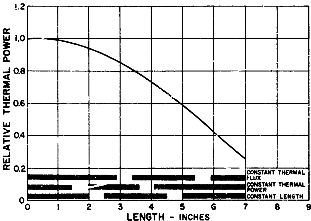
Figure 6-1 Thermal Power Distribution. Converter Length Criterion
