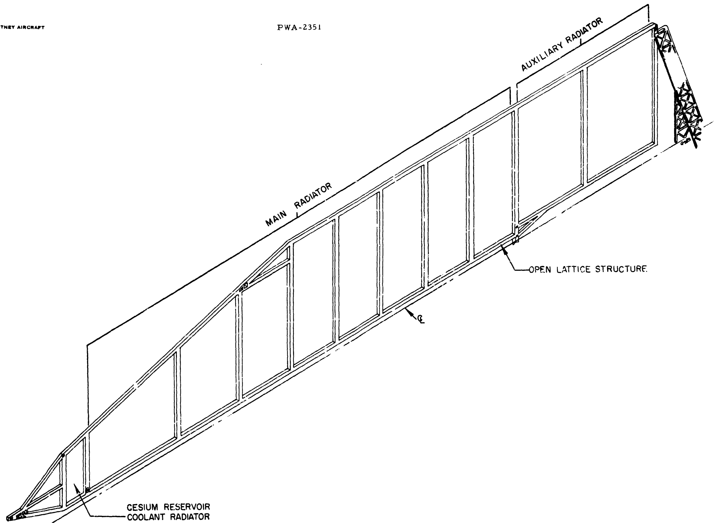
Figure 1-6 Radiator Support Framework
