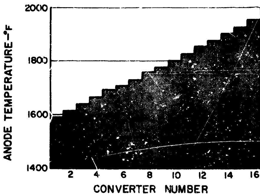
Figure 17 Anode Temperature
