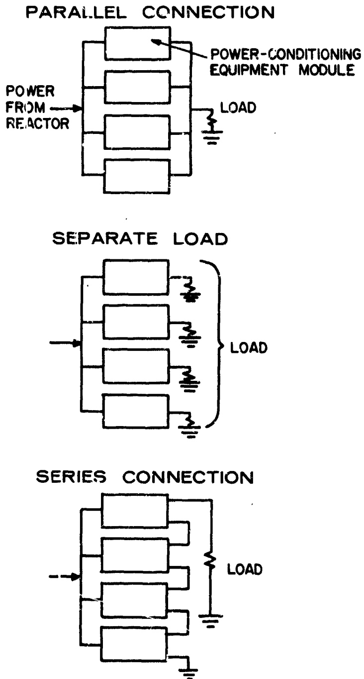
Figure 37 Load Circuit Diagrams
