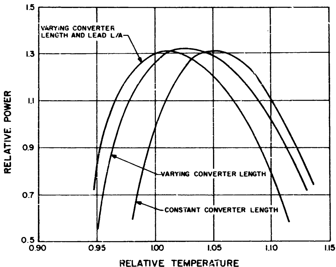
Figure 6-7 Fuel Element Performance. Variable Fuel Loading
