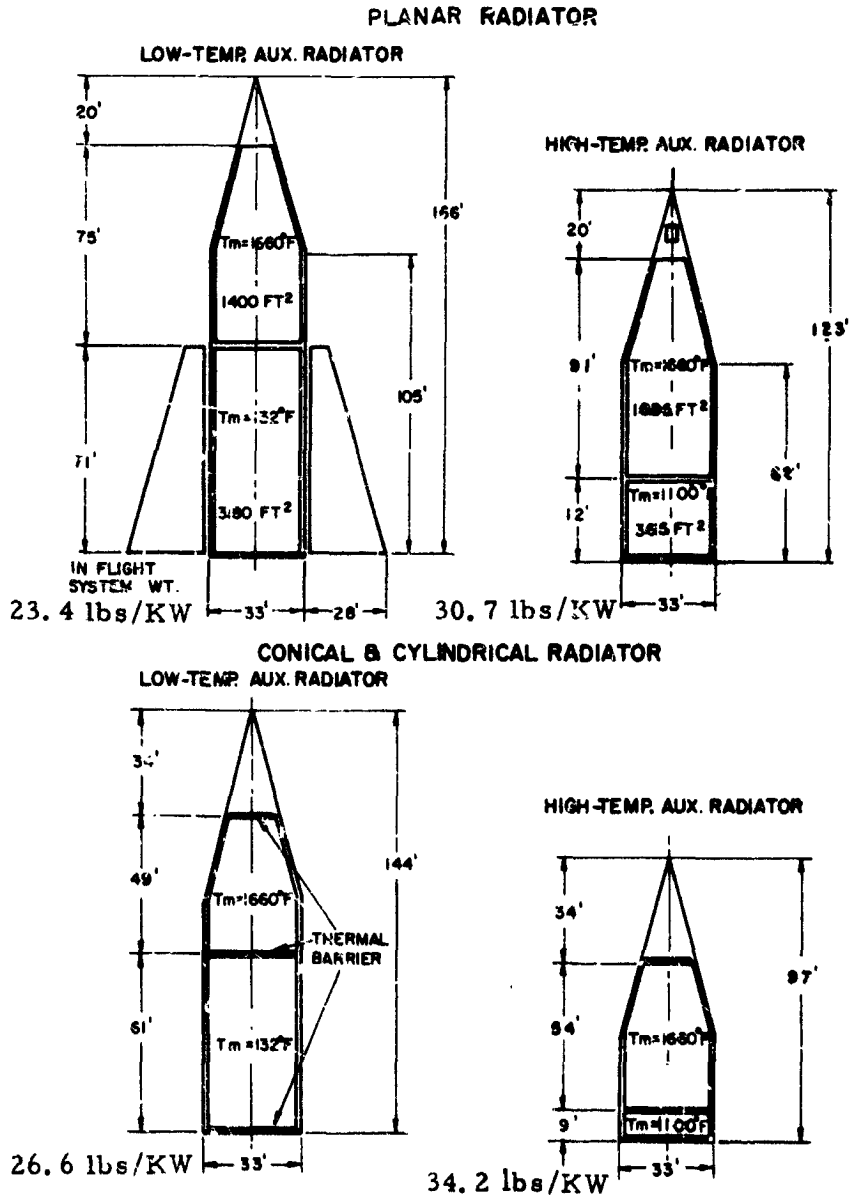
Figure 2-2 Revised Estimates Based on New Power-Conditioning Information
