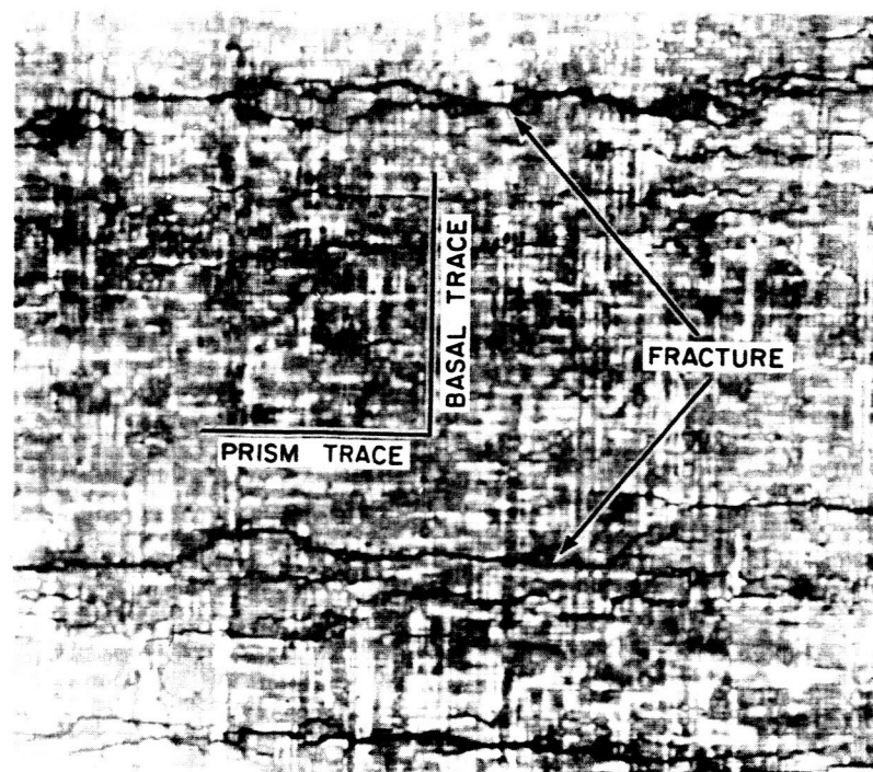
Fig. 1 - Bend Surface of Crystal Oriented for Prism Slip.
