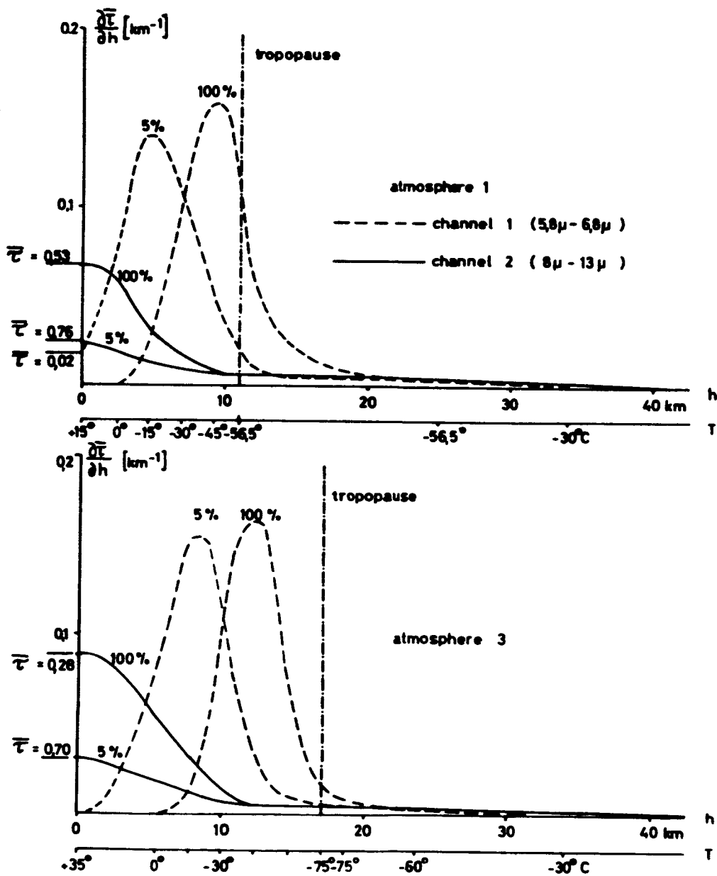
Fig. 3.3 : Curves of \frac{\partial F}{\partial h} vs. the height h for the outgoing radiation flux which are defined in Eqs. 3.4
