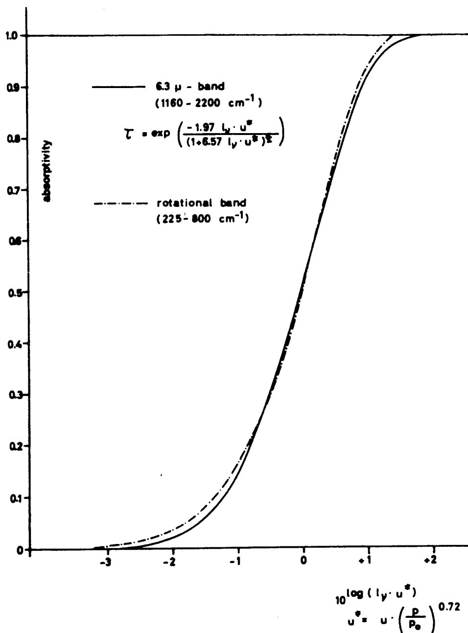
Fig. 4.3 : Spectral absorptance of the 6.3μ - band and rotation band of water vapor
