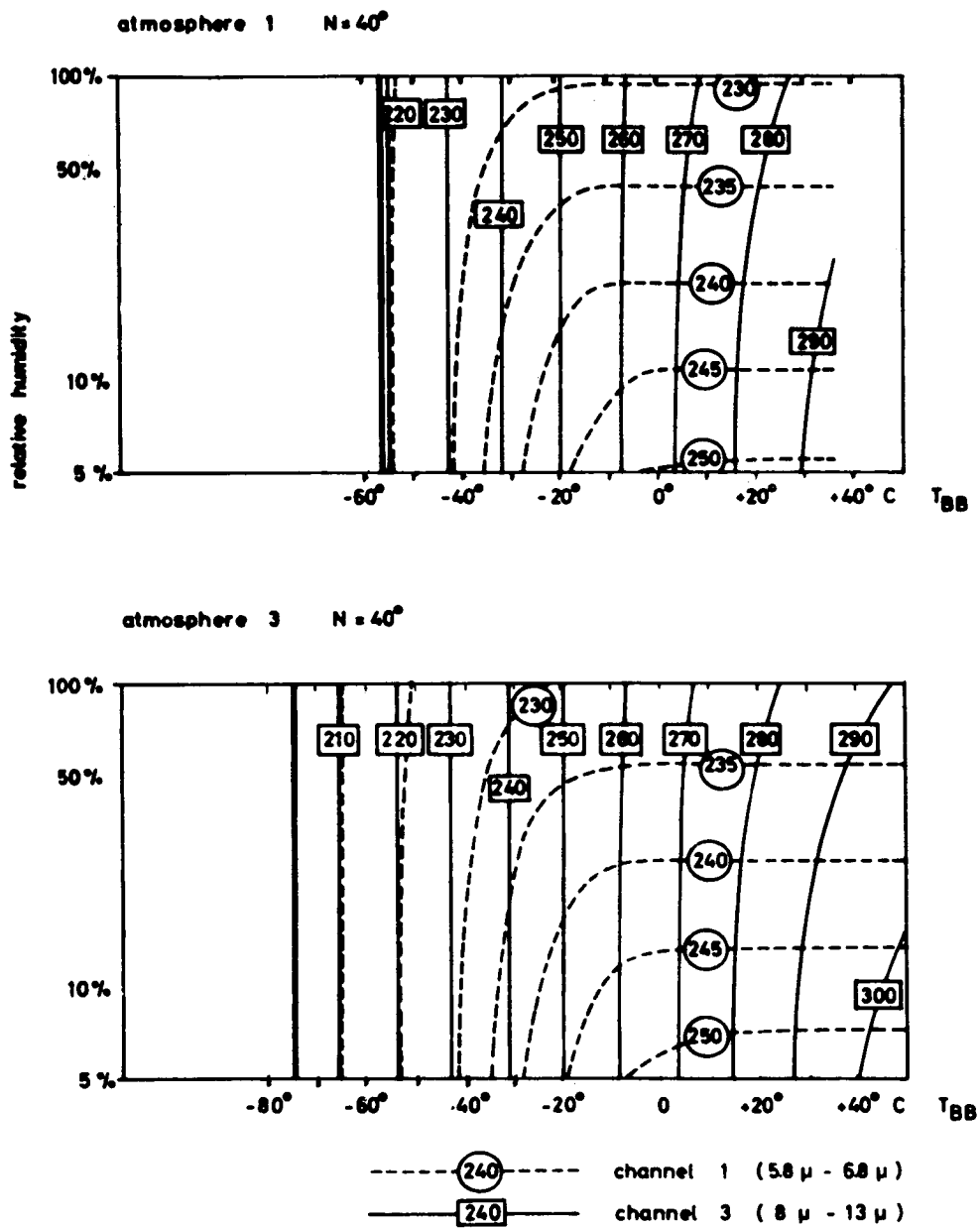
Fig. 3.9 : Evaluation diagrams for the nadir angle N = 40^\circ
