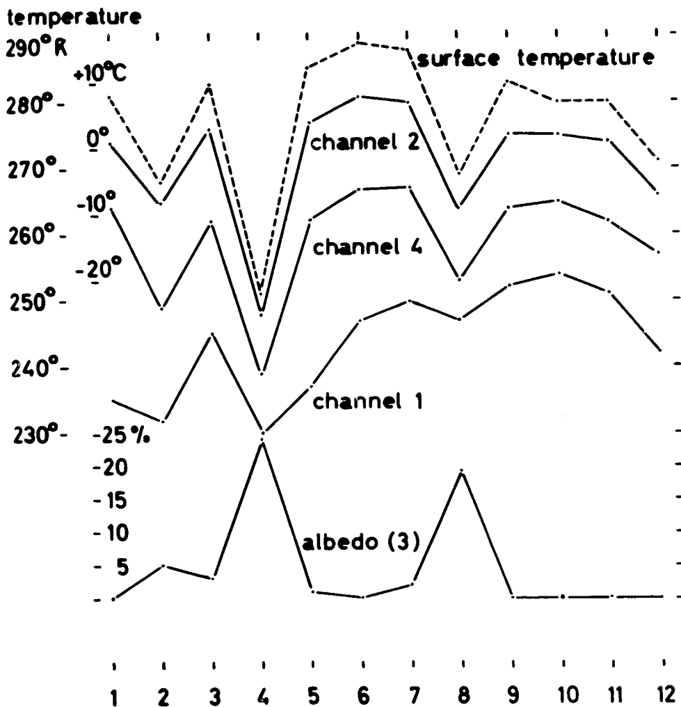
Fig. 4.9 : Comparison of radiation data from 12 points which were viewed with constant nadir angle ( 30^{\circ} - 40^{\circ} ) during orbit 61.
