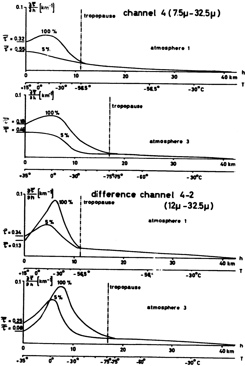
Fig. 3.4 : Curves of \frac{\partial F}{\partial h} vs. the height h for the outgoing radiation flux which are defined in Equ. 3.4
