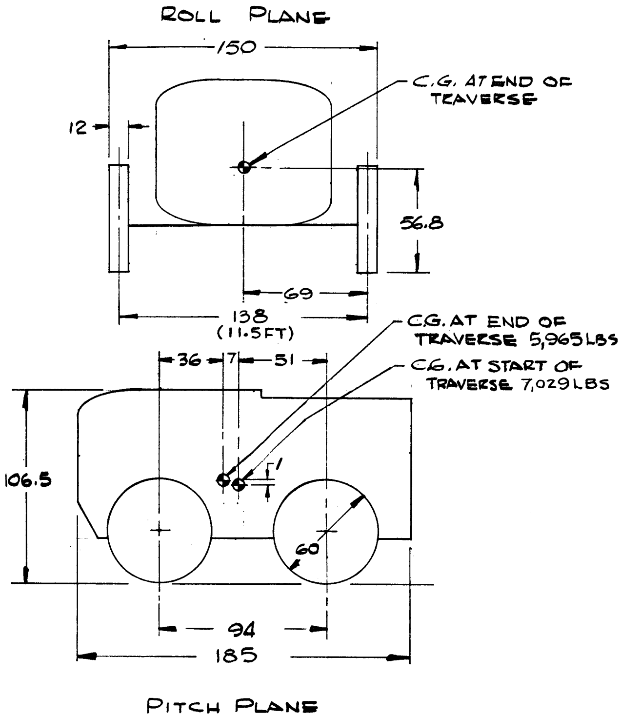
FIGURE 1. MOLAB VII CHARACTERISTICS
