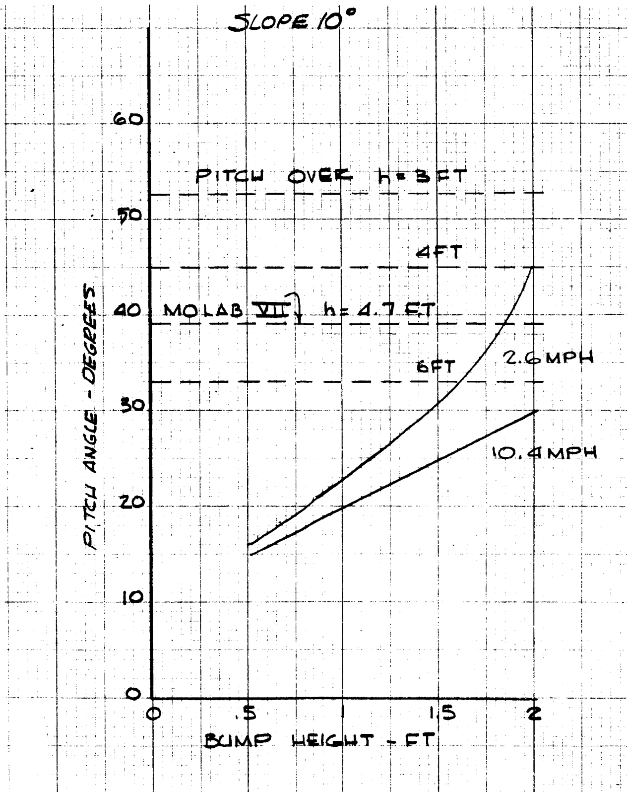
FIGURE 3B. PITCH PLANE STABILITY, SLOPE 10^\circ
