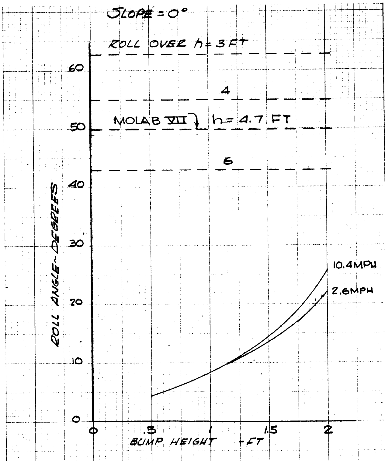
FIGURE 4A. ROLL PLANE STABILITY, SLOPE = 0^\circ
