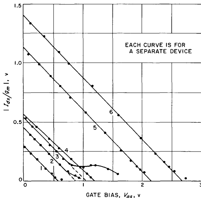
Fig. 8. Measured FET characteristics
