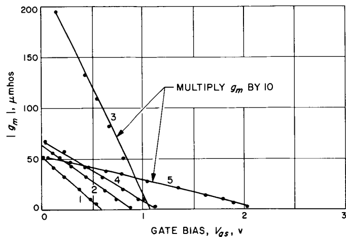
Fig. 9. Measured transconductance
