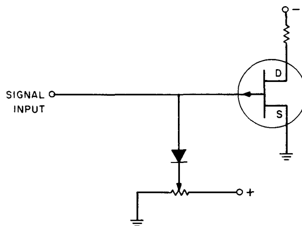
Fig. 5. Leakage current cancellation
