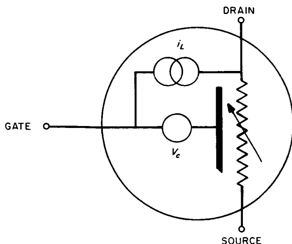
Fig. 2. Drift equivalent circuit of FET
