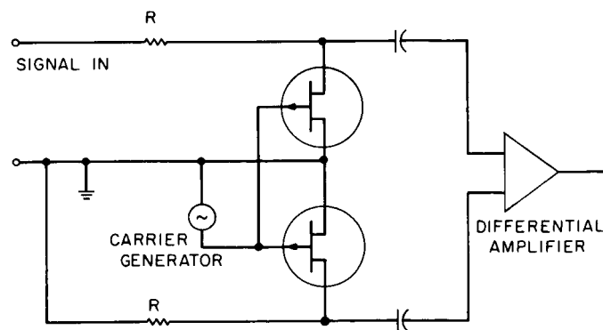
Fig. 6. Balanced chopper
