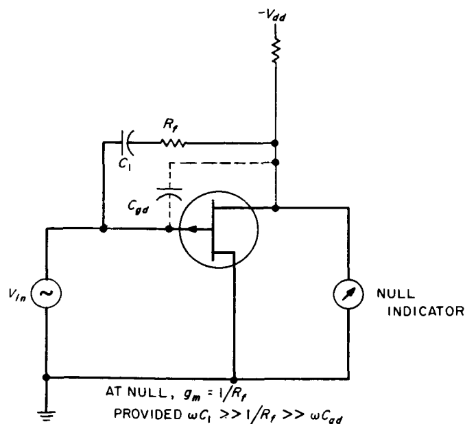
Fig. 7. Transconductance measurement
