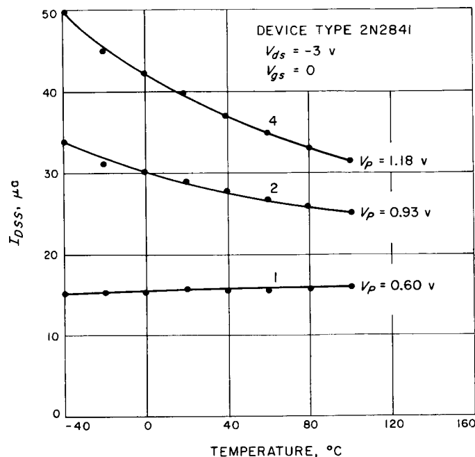
Fig. 10. Drain current vs. temperature
