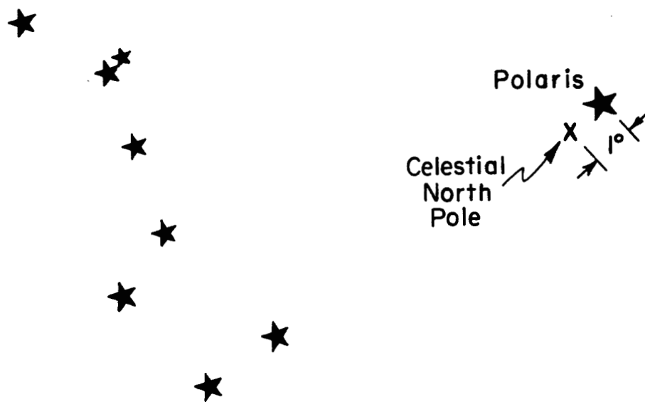
Fig. 3. Position of Polaris relative to the Celestial North Pole and the constellation Ursa Major.
