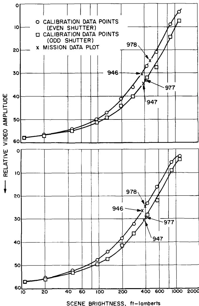
Fig. 41. Light-transfer characteristics, camera P_3
