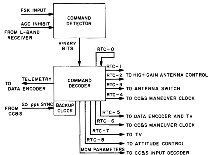
Fig. 11. Command Subsystem
