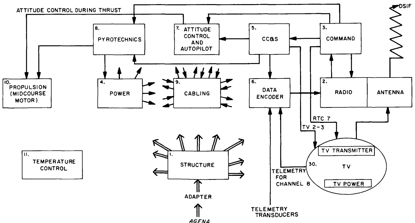
Fig. 5. Ranger Block III spacecraft Subsystems
