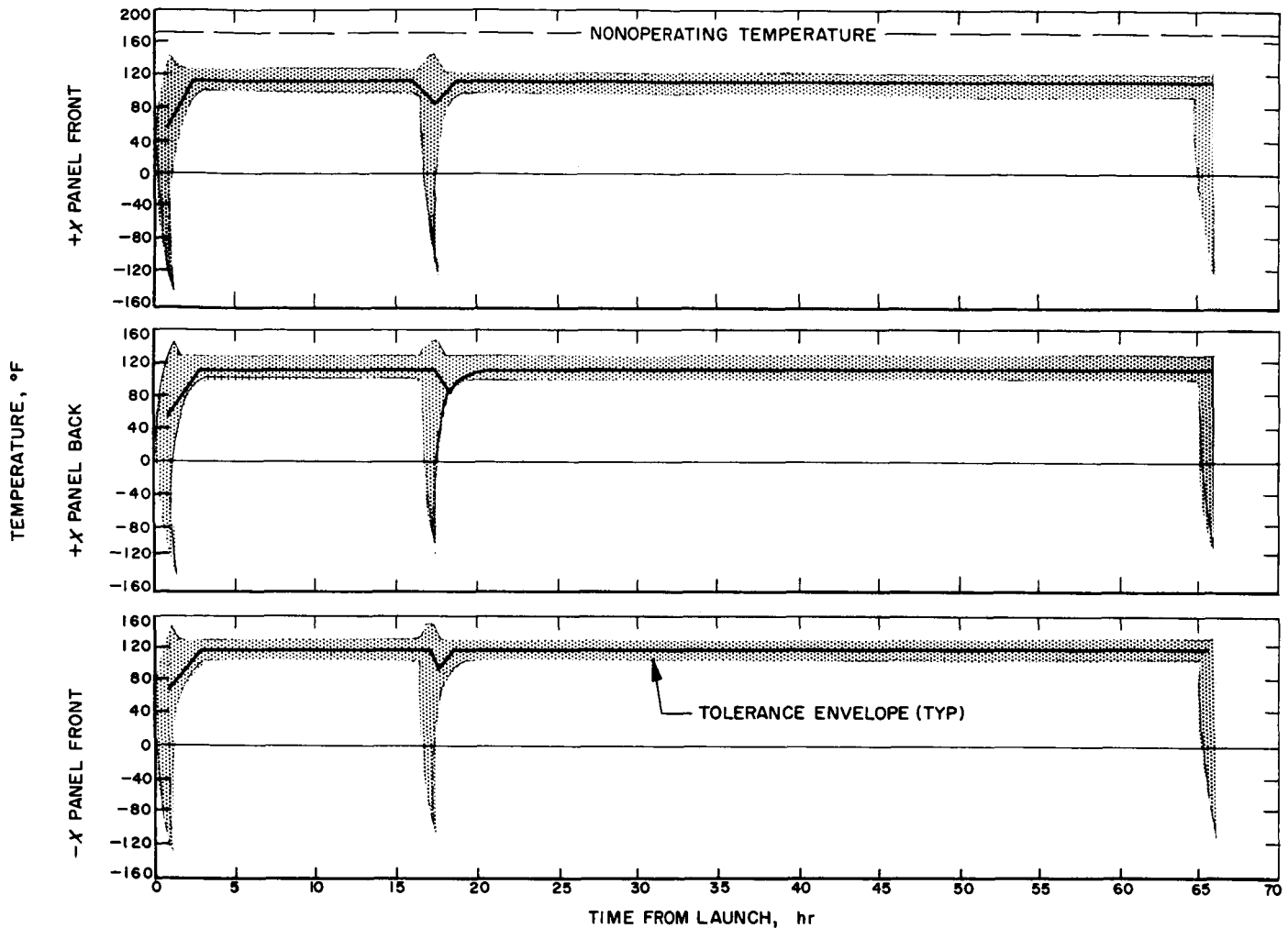
Fig. 15. Solar-panel temperatures
