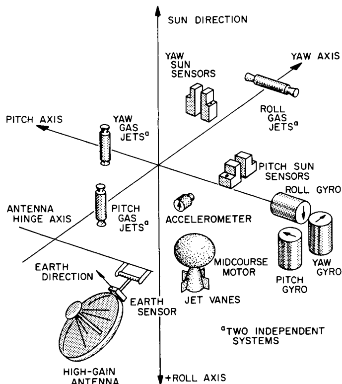
Fig. 23. Attitude Control elements
