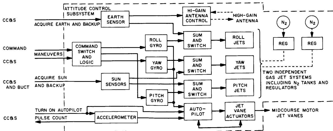
Fig. 24. Attitude Control Subsystem
