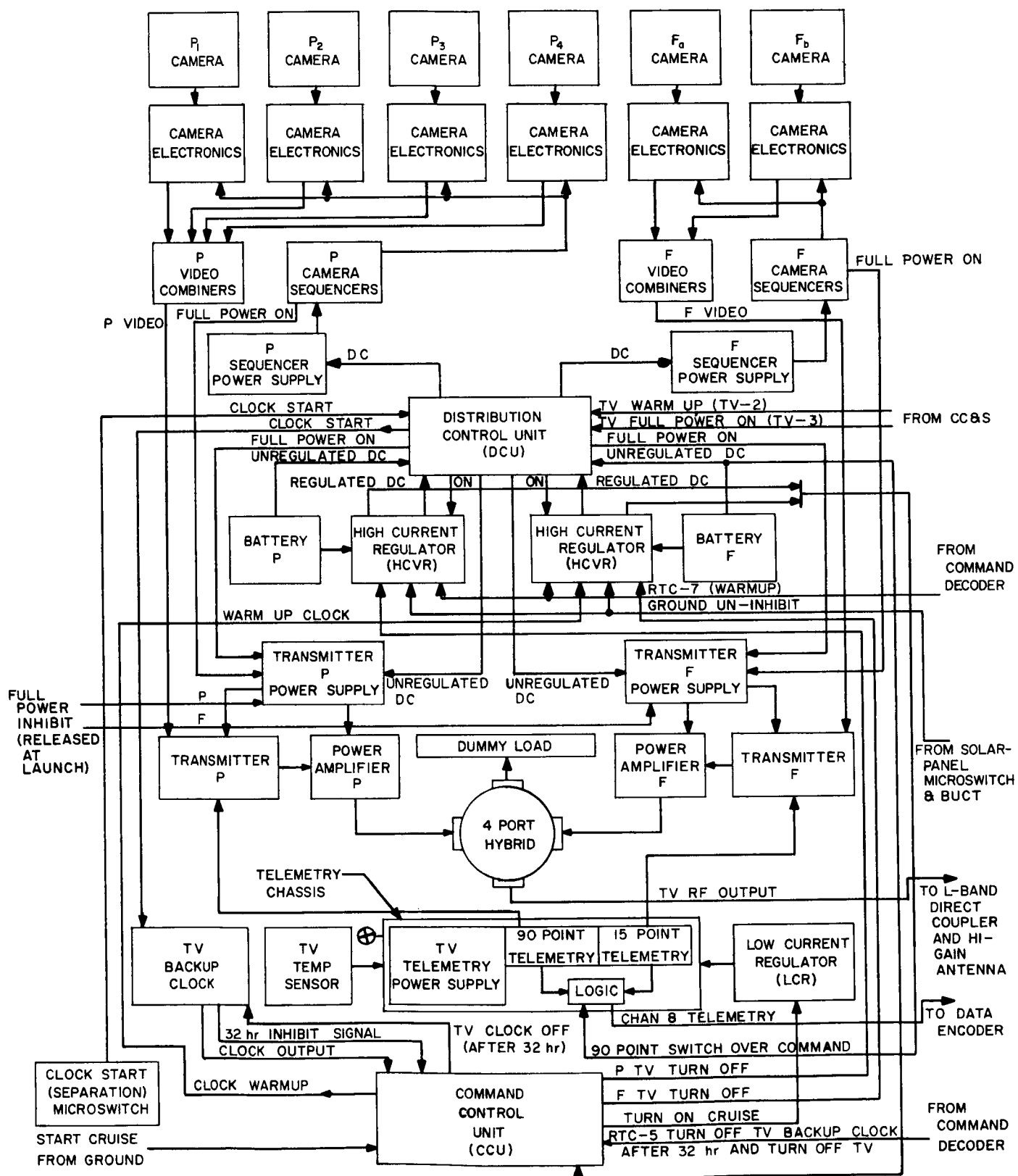
Fig. 29. Television Subsystem
