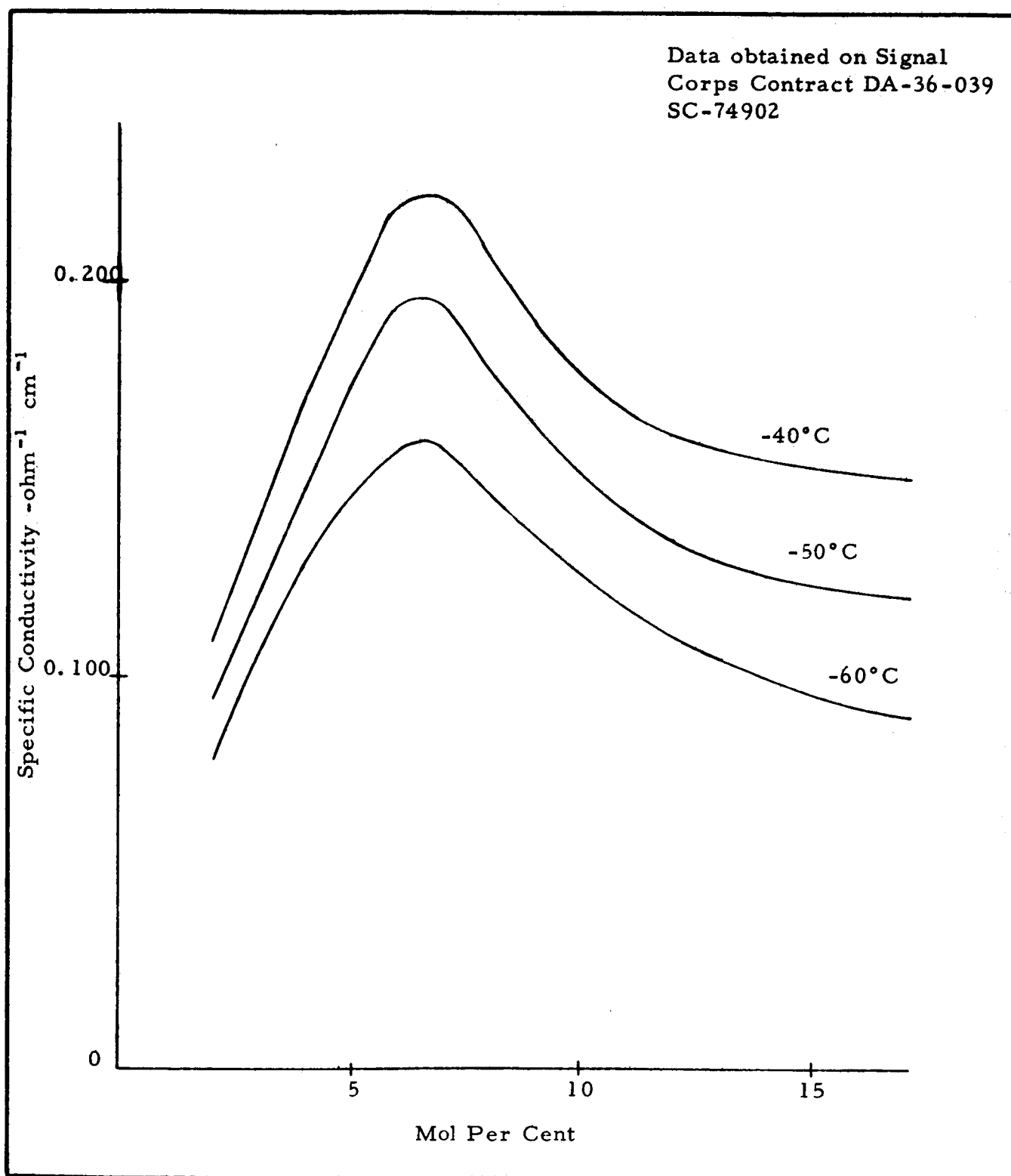
SPECIFIC ELECTRICAL CONDUCTIVITY OF THE SYSTEM \text{NH}_3(\text{l}):\text{KSCN}
