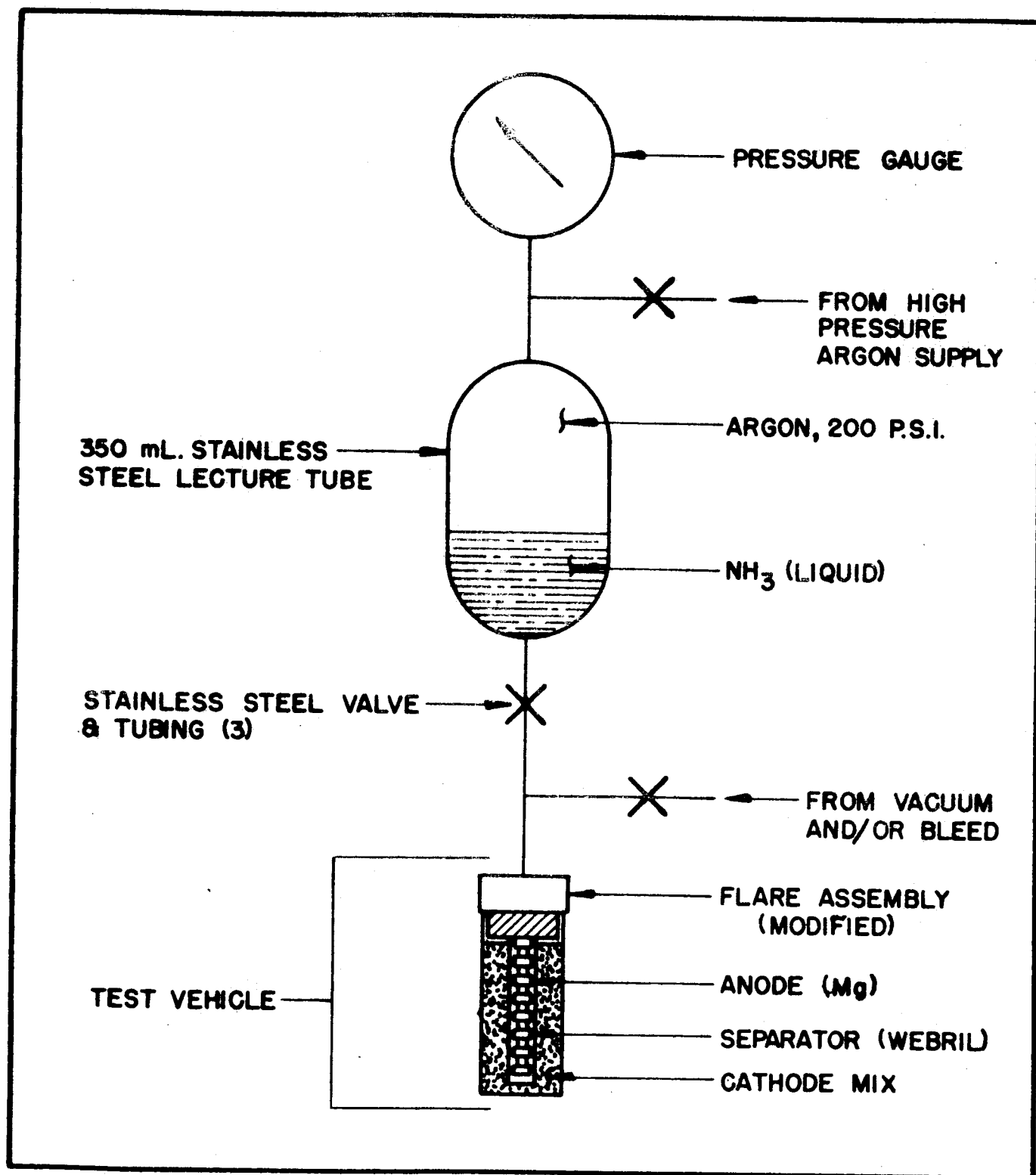
SCHEMATIC OF THE MANIFOLDING OF THE A-601 TEST VEHICLE
