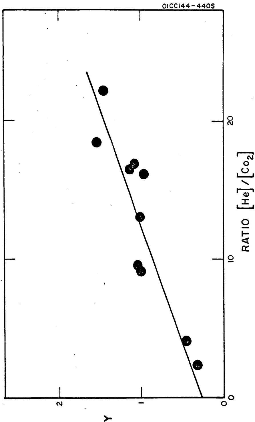
Figure 4. Plot of Y (see test) versus (\text{He})/(\text{CO}_2) making use of the data shown in Figure 3.
