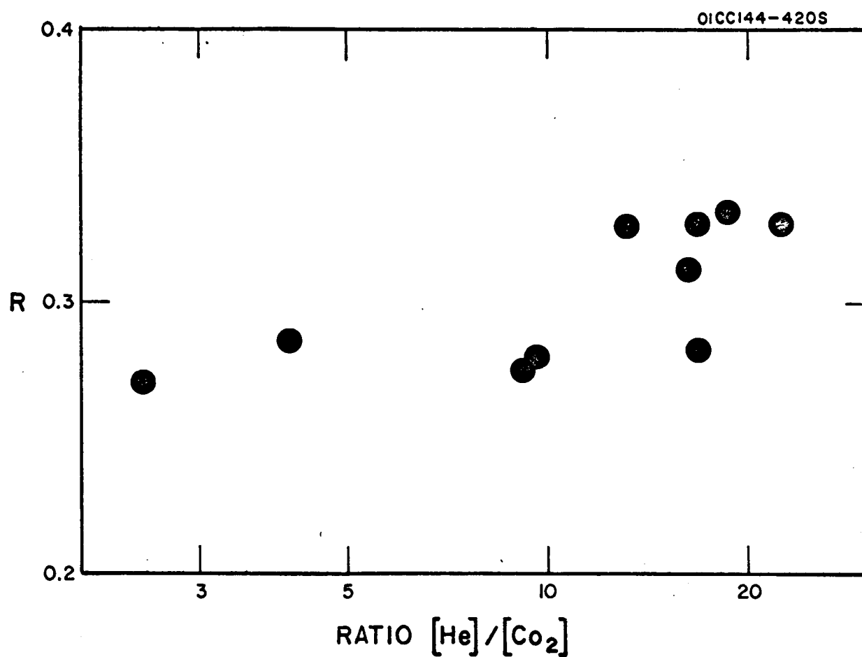
Figure 3. Dependence of R = (O_2)/CO on the ratio of admixed helium to carbon dioxide concentration. Carbon dioxide pressure 22 mm Hg. Effective light intensity about 1 \times 10^{15} quanta/sec.
