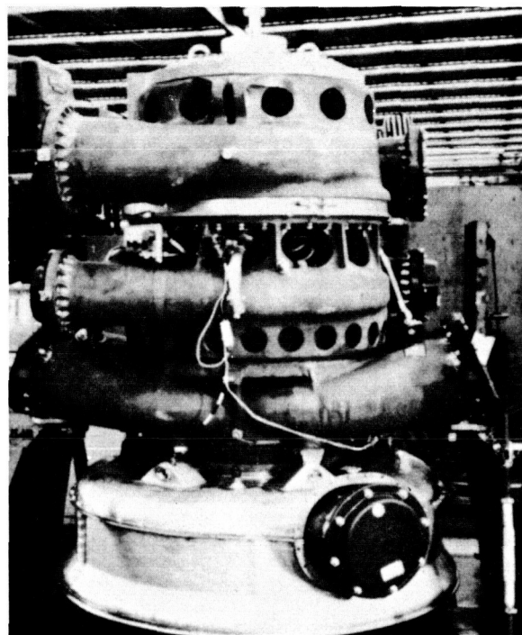
FIGURE IV-14.—Turbopump for 1500K-thrust engine.
