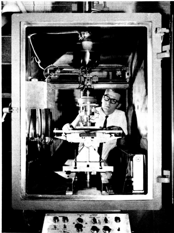
FIGURE II-10.—Electron-beam welder.
