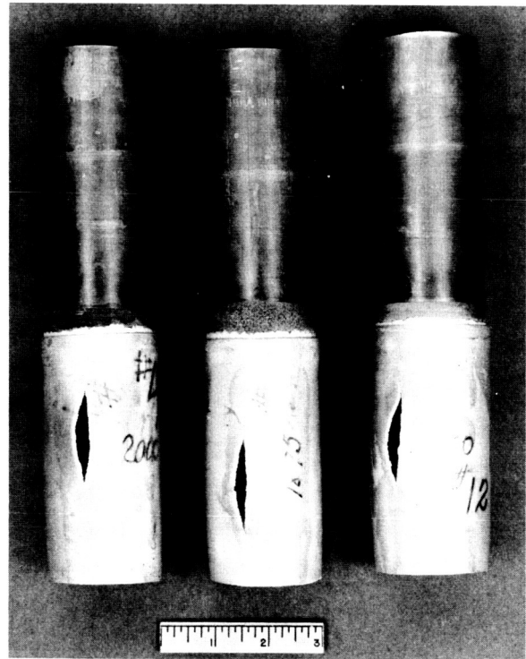
FIGURE II-2.—Two-inch-diameter brazed joints of 321 stainless steel to 6061 aluminum after burst test.
