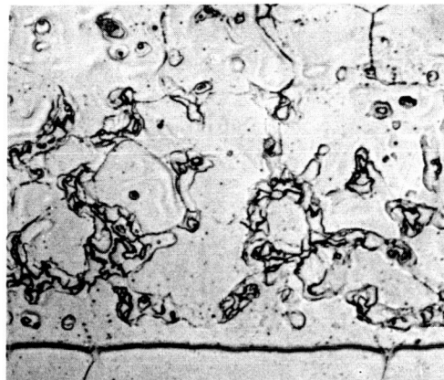
FIGURE II-4.—Inconel-X braze alloy, 304L stainless-steel interface, showing solution of Inconel-X by the braze alloy and extension of grain boundaries. \times 150 .
