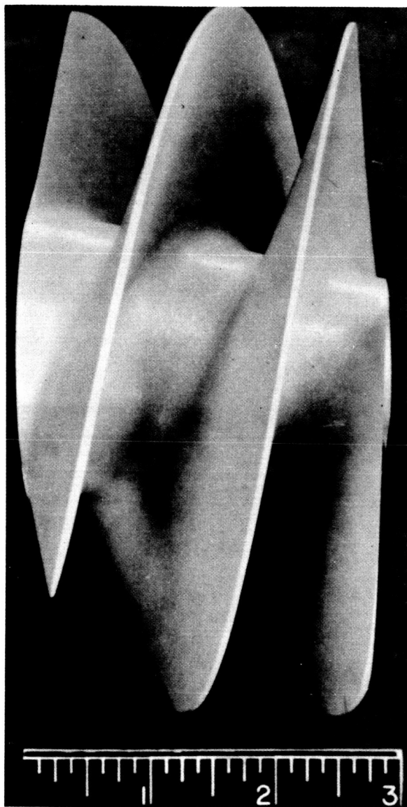
FIGURE IV-7.—Typical turbopump inducer.
