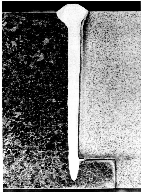
FIGURE II-11.—Electron-beam butt weld of udimet 500 to 4340 steel .675-inch thick.
