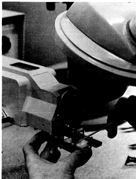
FIGURE II-9.—Resistance-welding apparatus.
