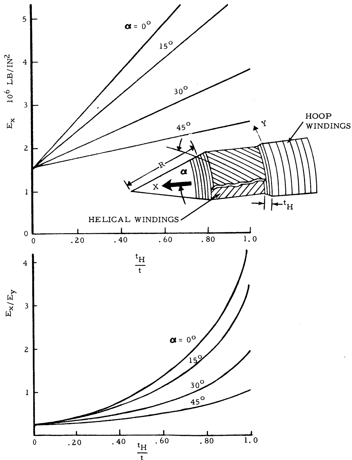
FIGURE IX-8.—Filament-wound composite-wall directional-stiffness control.
