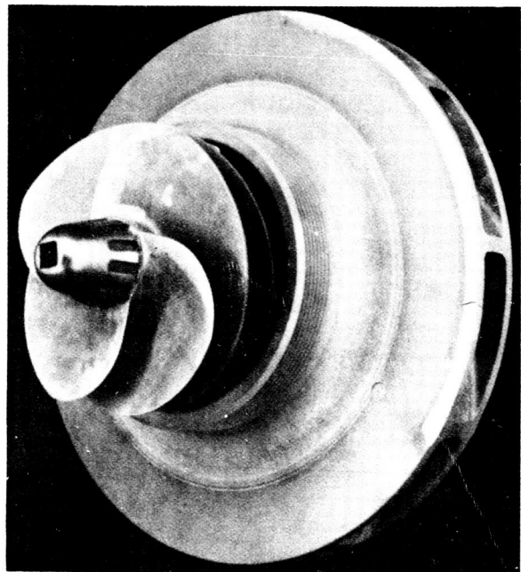
FIGURE IV-16.—Cavitating inducer and impeller.
