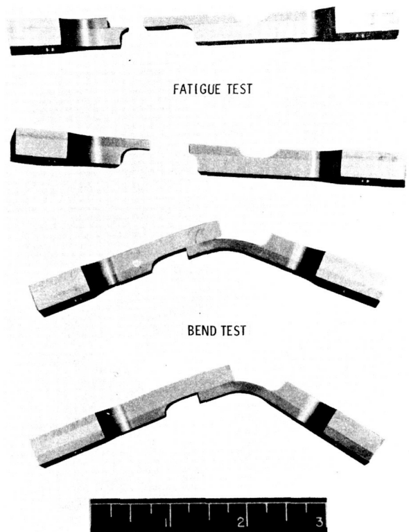
FIGURE II-13.—Bar specimens of roll-bond aluminum to stainless steel after fatigue and bend tests.
