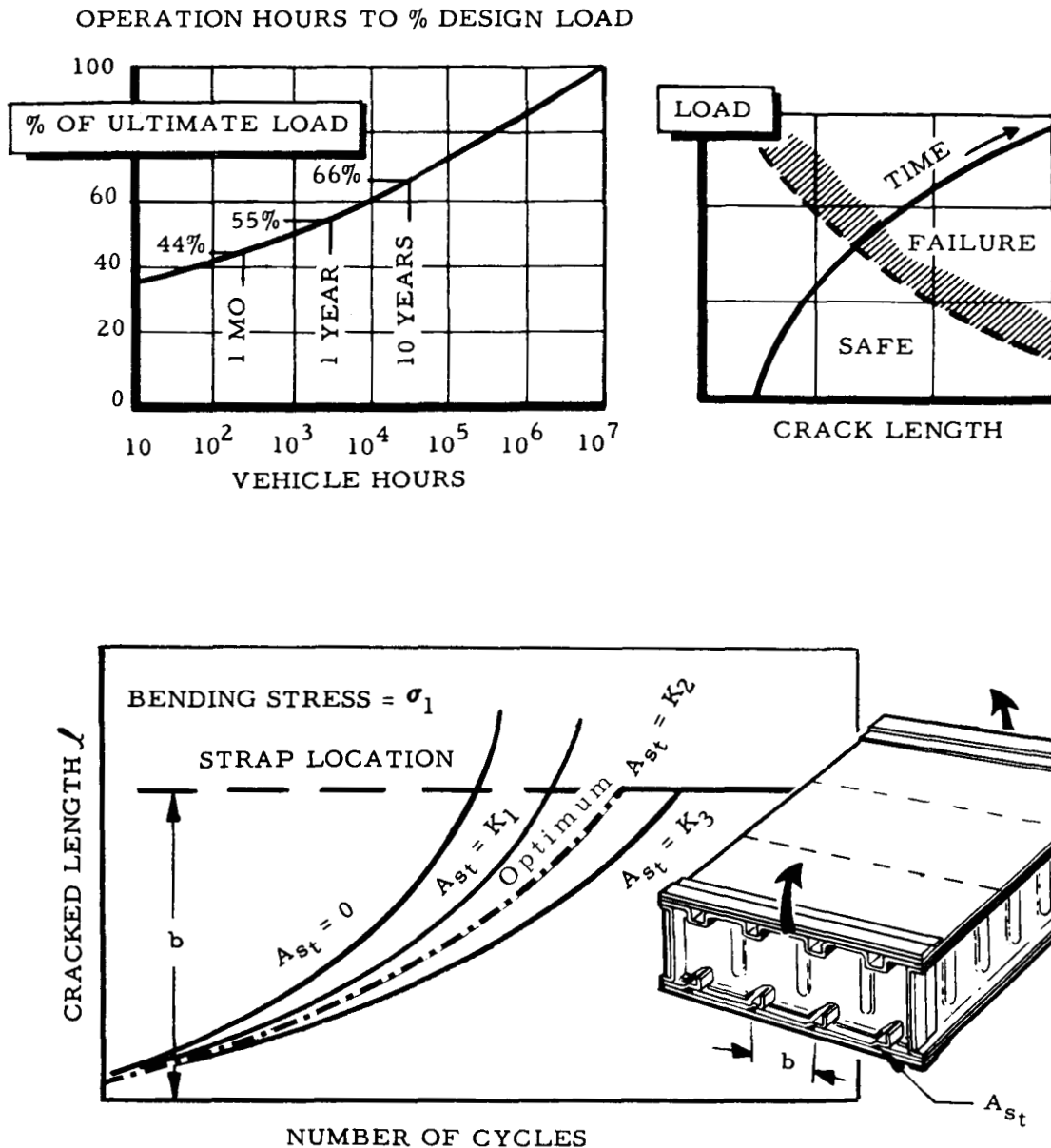
FIGURE IX-15.—Operational considerations for crack growth and detection relationships and determining optimum wing-box strap area for operational-cycles requirements.
