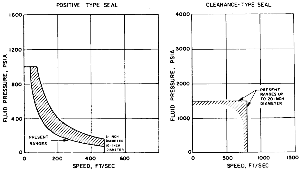
FIGURE IV-9.—Positive and clearance seal operating requirements.
