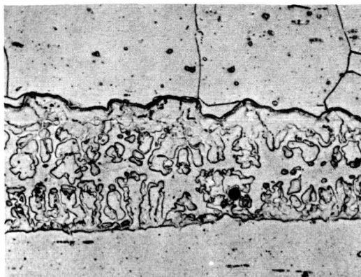
FIGURE II-3.—Inconel-X braze alloy, 304L stainless-steel interface, showing normal joint. \times 150 .
