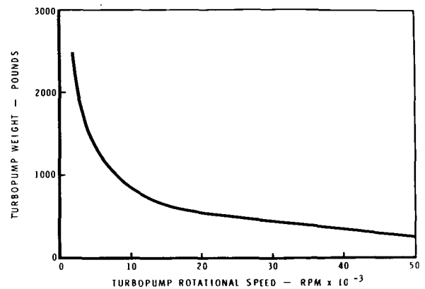
FIGURE IV-6.—Turbopump weight versus rotational speed. The pump pressure rise is 2,000 psi and the pump flow rate is 10,000 gpm.
