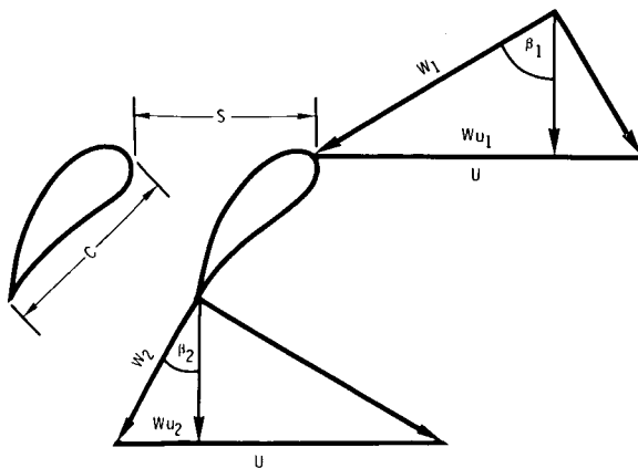
FIGURE IV-10.—Blade velocity diagram.
