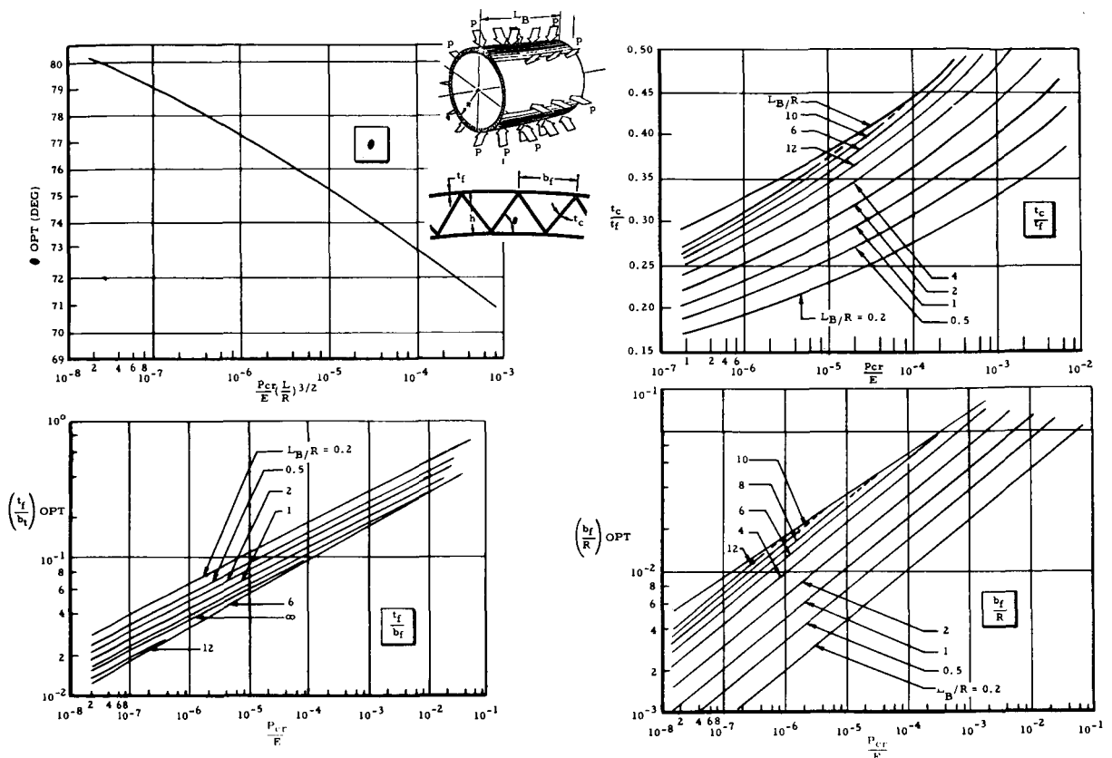
FIGURE IX-18.—Optimum-geometry values of truss angle \theta , t_c/t_f/b_f , and b_f/R for truss-core sandwich cylinders under hydrostatic collapse pressure.
