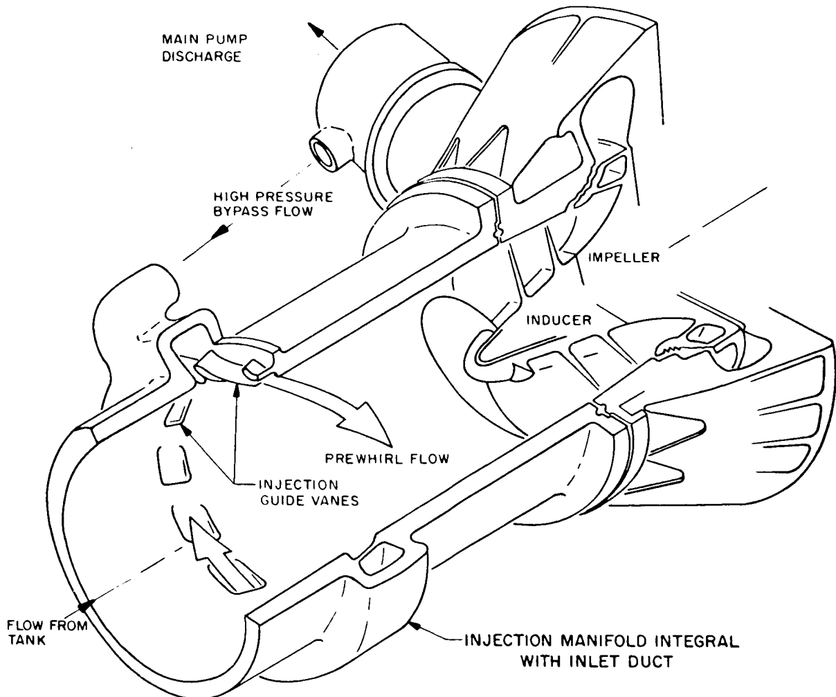
FIGURE IV-19.—Turbopump inlet fluid injection schematic.
