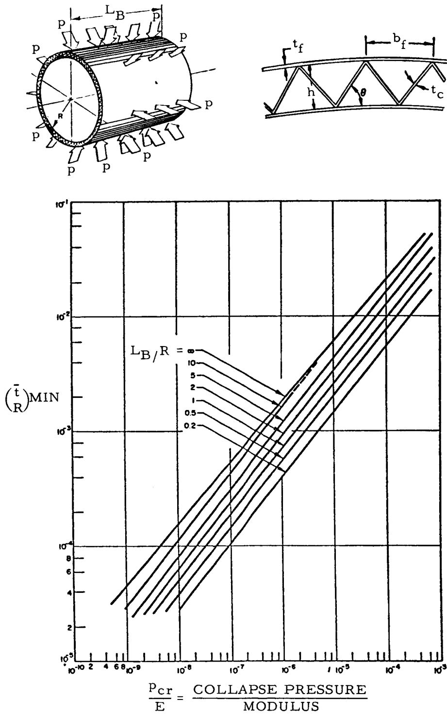
FIGURE IX-17.—Optimum-design chart with various bulkhead spacings for truss-core sandwich cylinders under hydrostatic collapse pressure.
