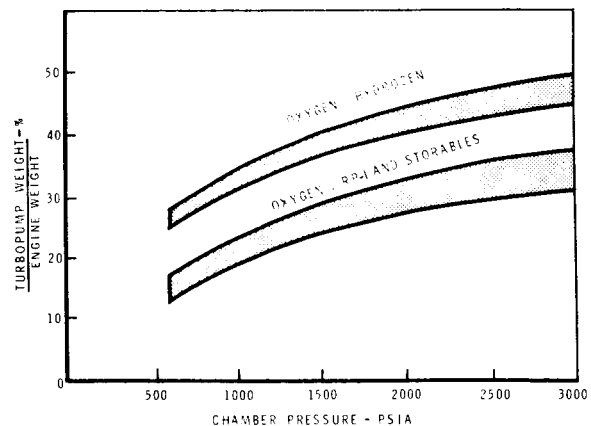
FIGURE IV-4.—Effect of chamber pressure on relative turbopump weights.
