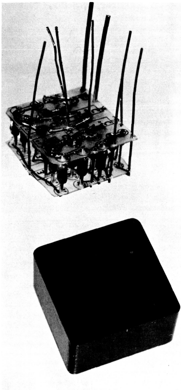
FIGURE II-8.—Resistance-welded high-density electronic modules.
