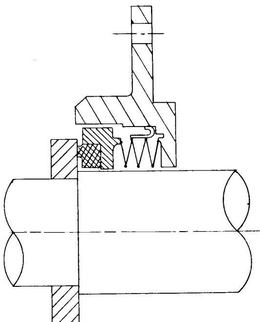
FIGURE IV-23.—Bellows seal.
