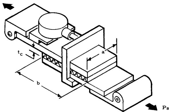
FIGURE IX-12.—Transverse-shear element tests.
