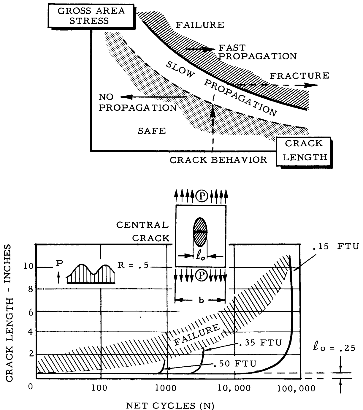
FIGURE IX-13.—Static- and cyclic-loading crack-propagation characteristics.
