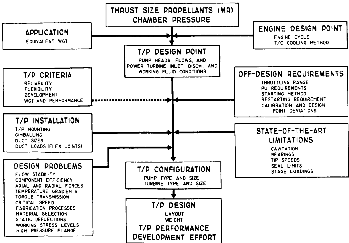
FIGURE IV-5.—Turbomachinery design process.
