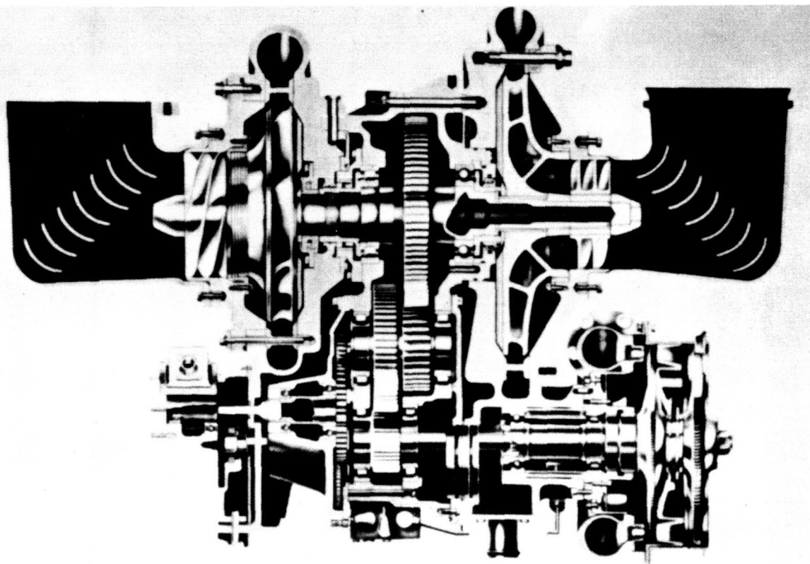
FIGURE IV-12.—Geared turbopump.
