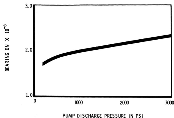
FIGURE IV-8.—Bearing speed versus pump-discharge pressure. The propellant is \text{LH}_2 and the flow rate is 10,000 gpm.
