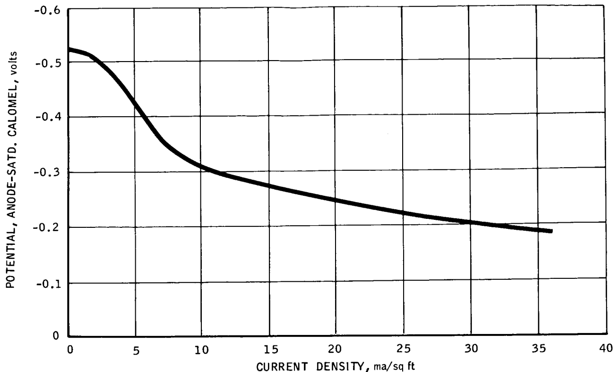
FIGURE VI-5.—A typical anodic-polarization curve. The cell is continuous flow, plastic; the pH is 8.3; and the temperature is 23° C. (System is described in table I.)
