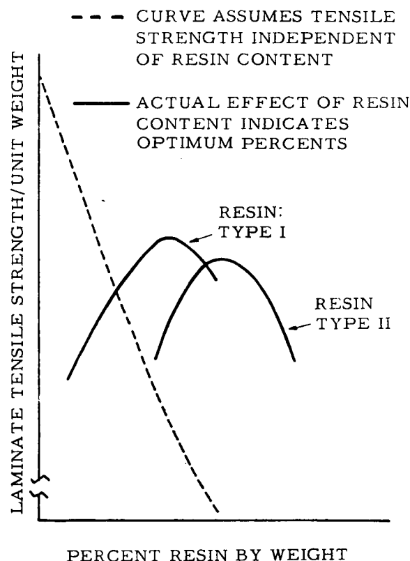
FIGURE IX-5.—Tensile strength/unit weight versus percent resin content by weight.
