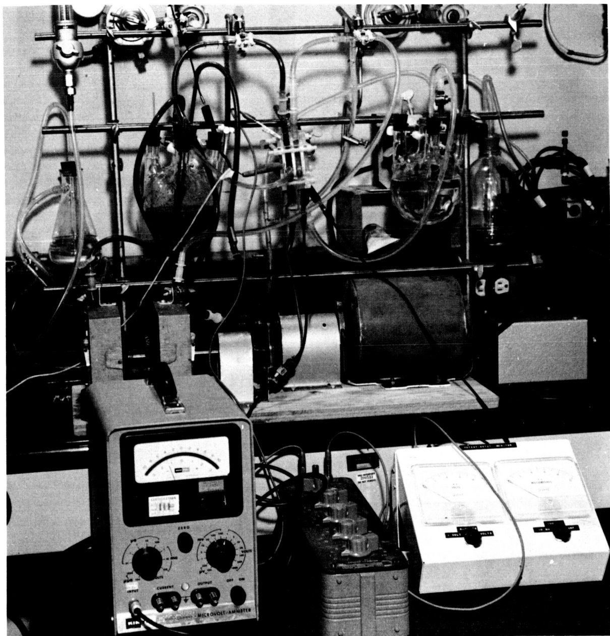
FIGURE VI-3.—Continuous-flow biofuel-cell system.
