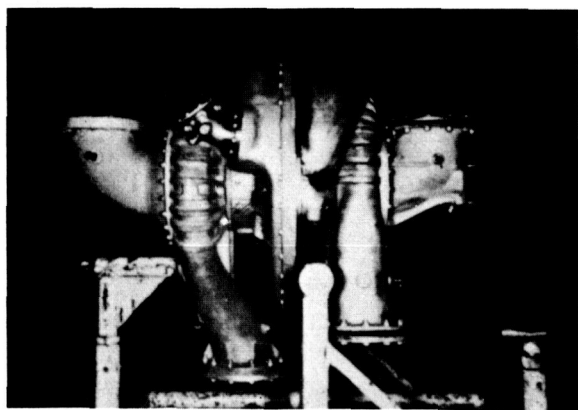
FIGURE IV-13.—Single-shaft turbopump for 700,000-lb.-thrust engine.
