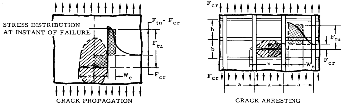
FIGURE IX-14.—Analytical equations for crack-propagation and crack-arresting.
