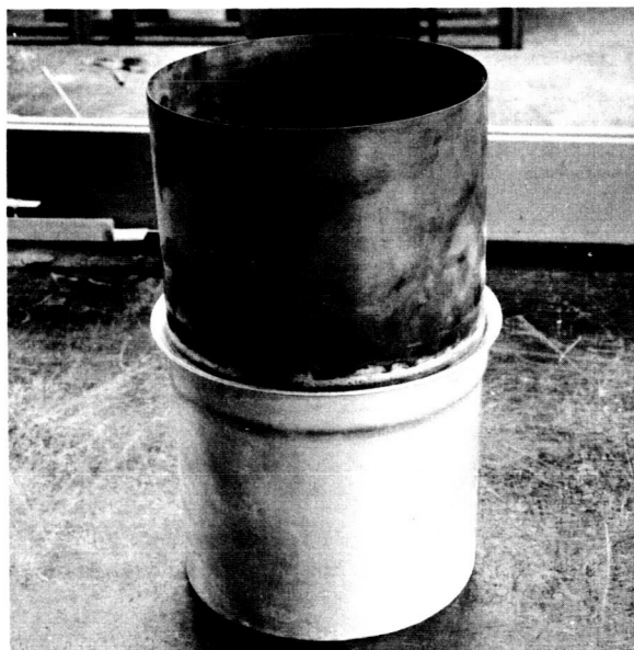
FIGURE II-1.—Eight-inch-diameter brazed joint of 321 stainless steel to 6061 aluminum alloy.
