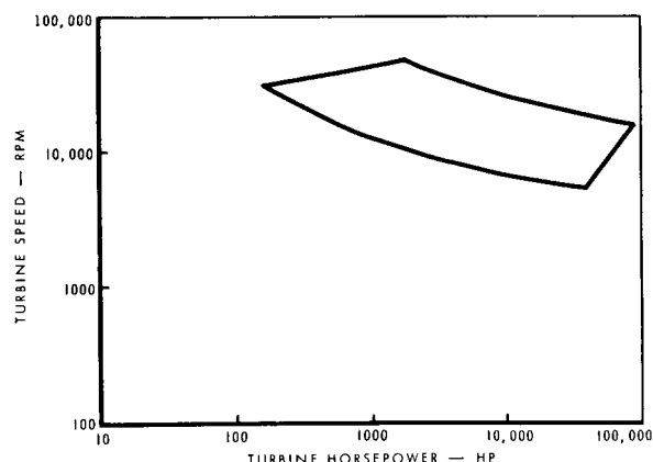
FIGURE IV-2.—Operation envelope of current turbines.
