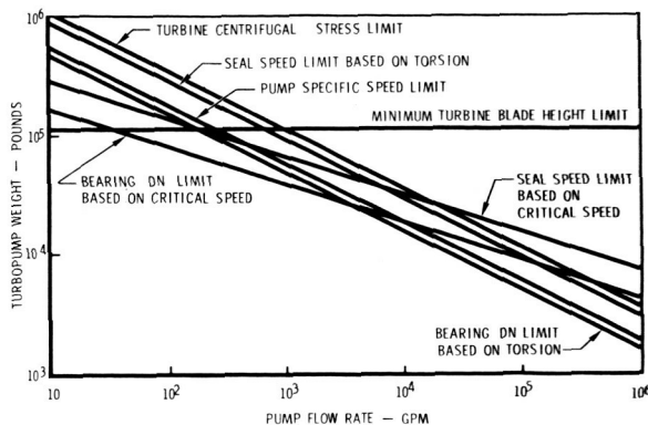
FIGURE IV-11.—Maximum rotational speeds allowed by various limits.
