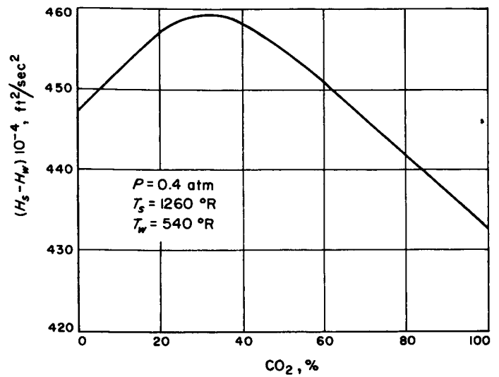
Fig. 7. Enthalpy difference vs % \text{CO}_2
