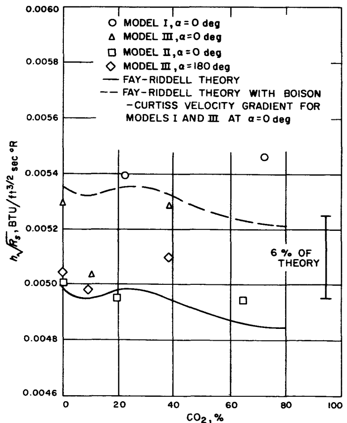
Fig. 10. Stagnation point heat transfer vs % \text{CO}_2
