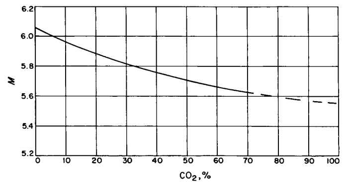
Fig. 8. Mach number vs % \text{CO}_2
