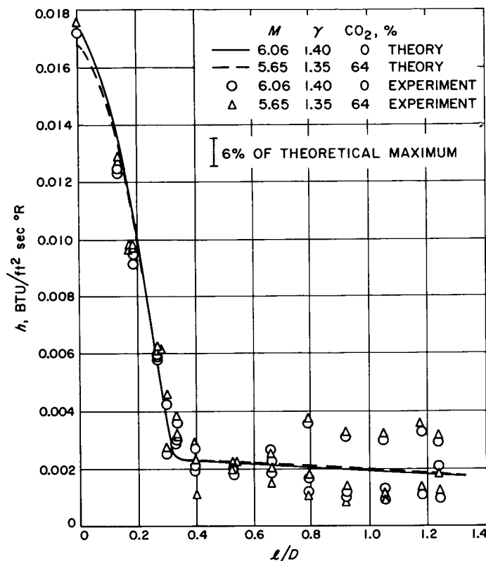
Fig. 12. Heat transfer distributions for Model II at \alpha = 0 deg
