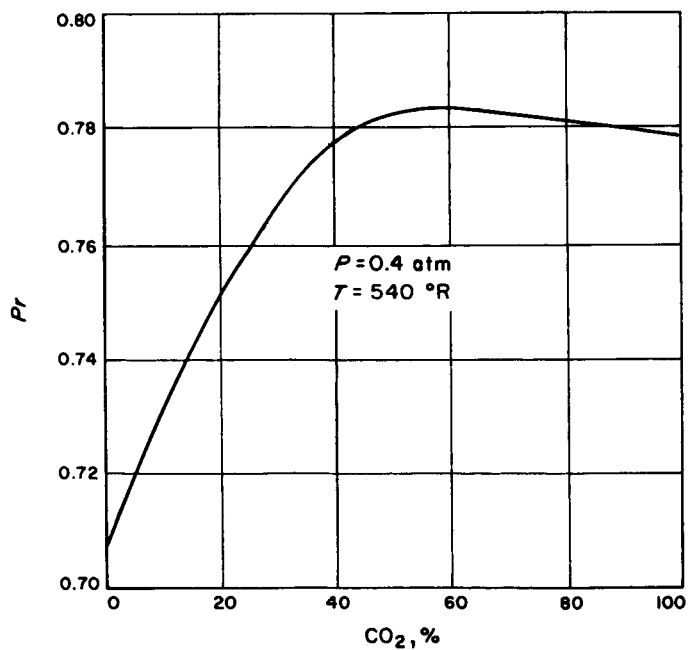
Fig. 6. Prandtl number vs % \text{CO}_2
