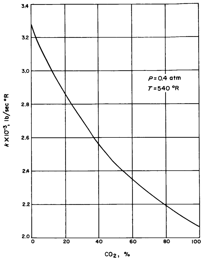
Fig. 5. Thermal conductivity vs % \text{CO}_2
