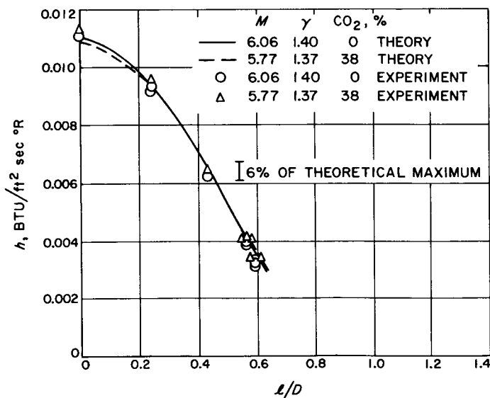
Fig. 13. Heat transfer distributions for Model III at \alpha = 180 deg
