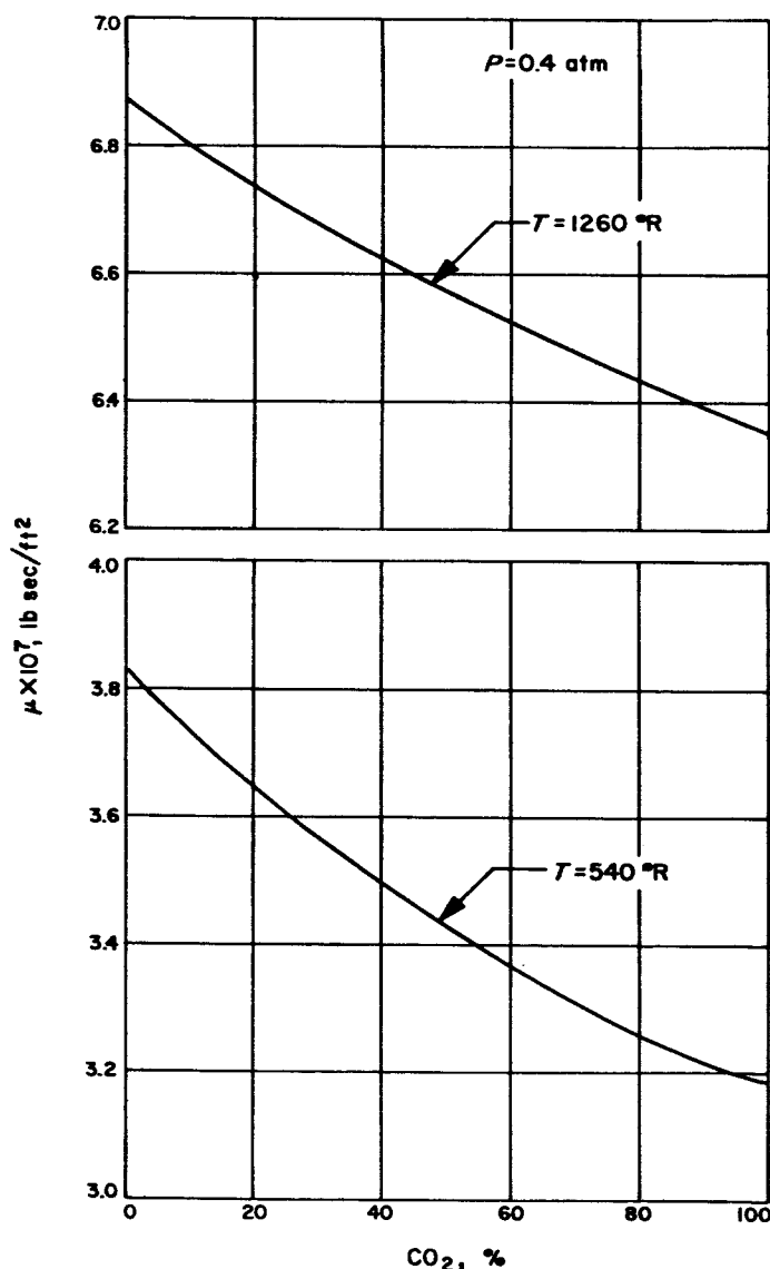
Fig. 4. Viscosity vs % \text{CO}_2
