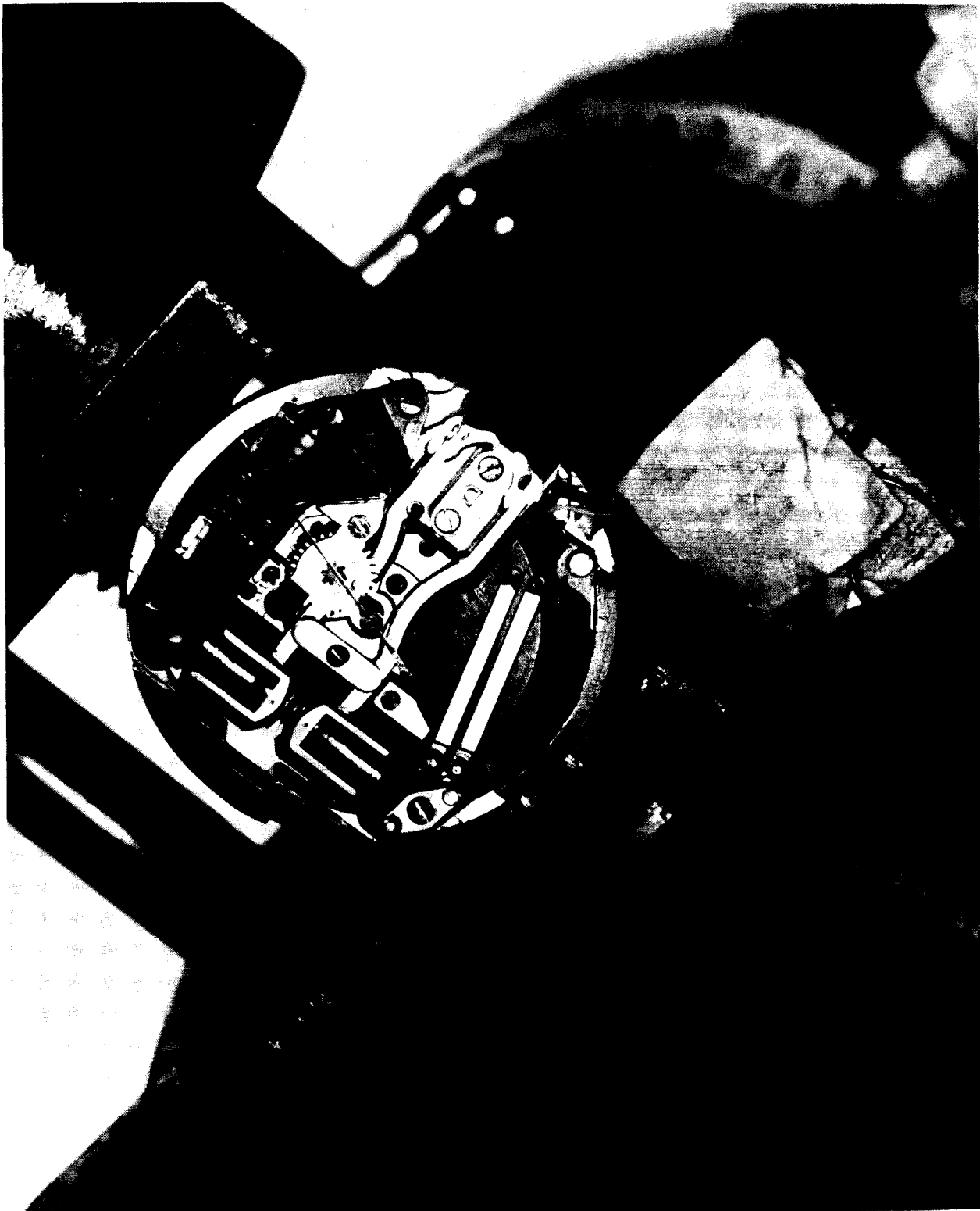
Figure 4-14. Accutron Movement
