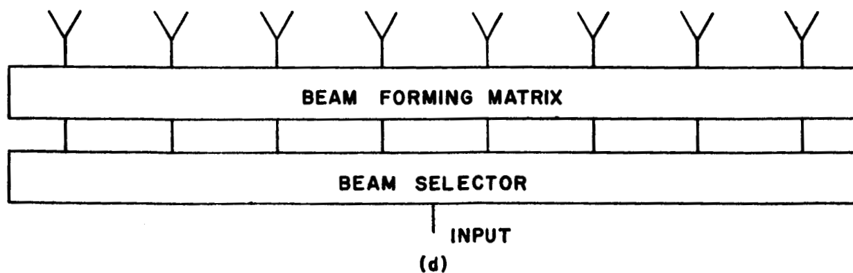
Fig.12. Linear Array Feed Structures.
