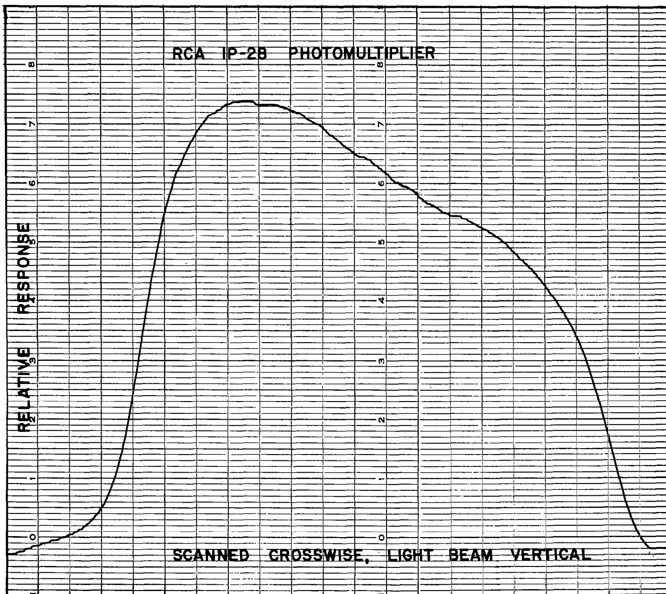
Fig. 11. Variations in sensitivity of an RCA IP-28 photomultiplier for monochromatic light flux as indicated when the cathode is moved across the exit slit of a spectroradiometer.
