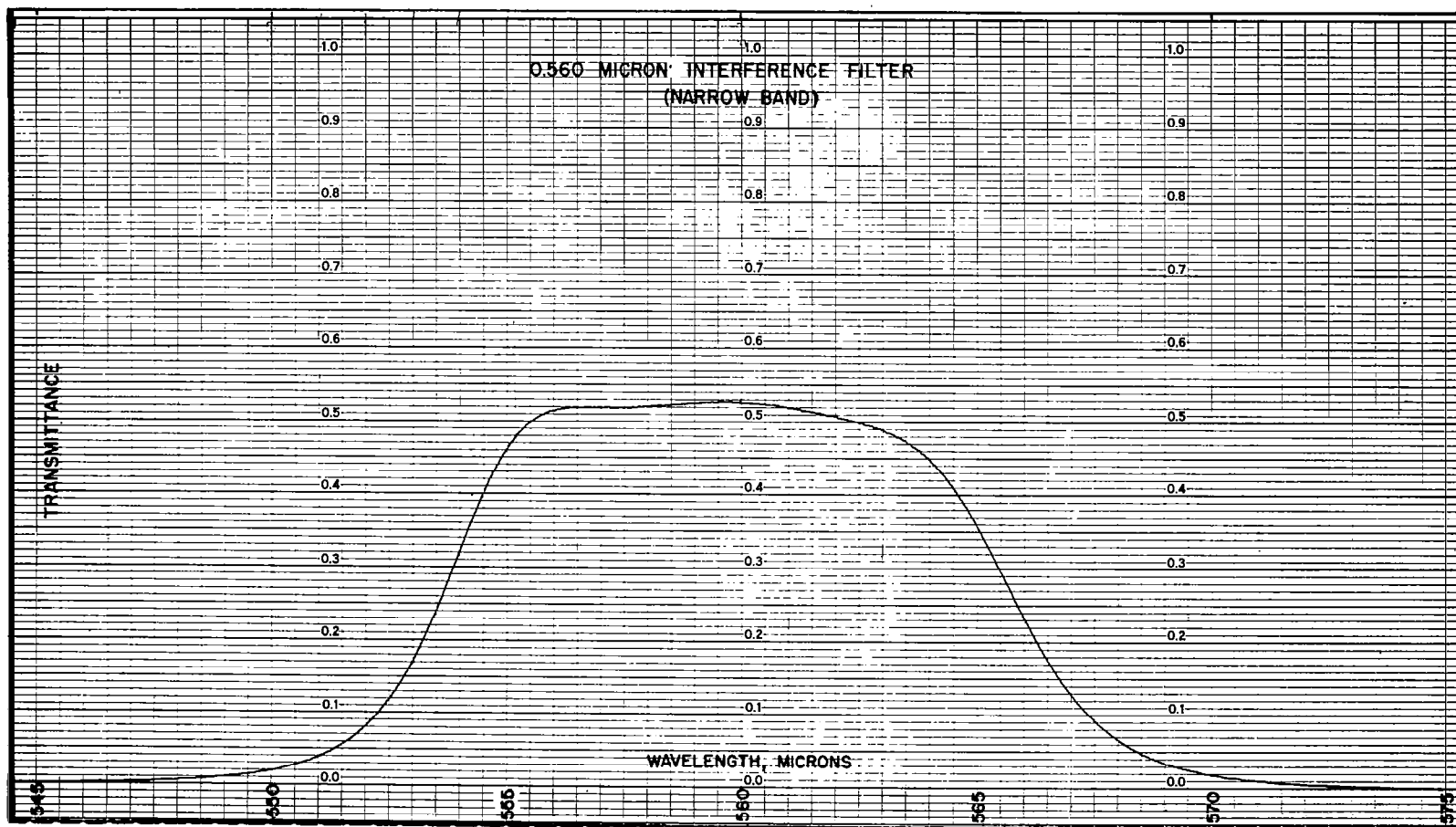
Fig. 27. Spectral transmittance of the 0.560 micron narrow-band interference filter as obtained on a Cary Model 14R spectrophotometer.
