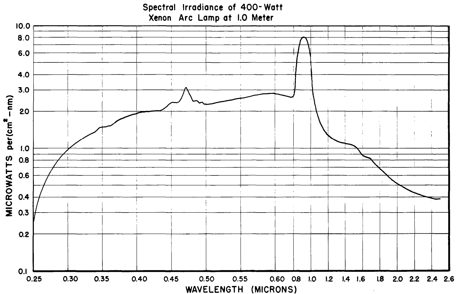
Fig. 30. Spectral irradiance from a 400-watt xenon lamp at a distance of 1 meter in microwatts per (cm 2 -nm).
