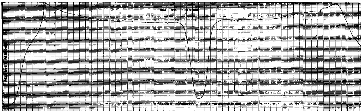
Fig. 15. Variations in sensitivity of an RCA type 935 phototube for monochromatic light flux as indicated when its cathode is moved across the exit slit of a spectroradiometer. The dip near the center of the illustration results from shadowing effects of the anode wire. This tube is employed with the major part of the surface exposed when used in the filter spectroradiometer.
