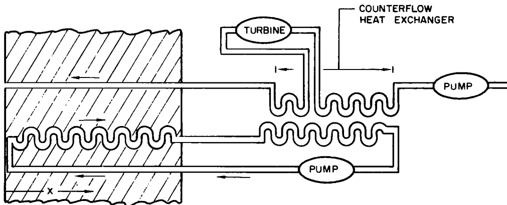
b - FULL COOLING USING AUXILIARY COOLANT LOOP
