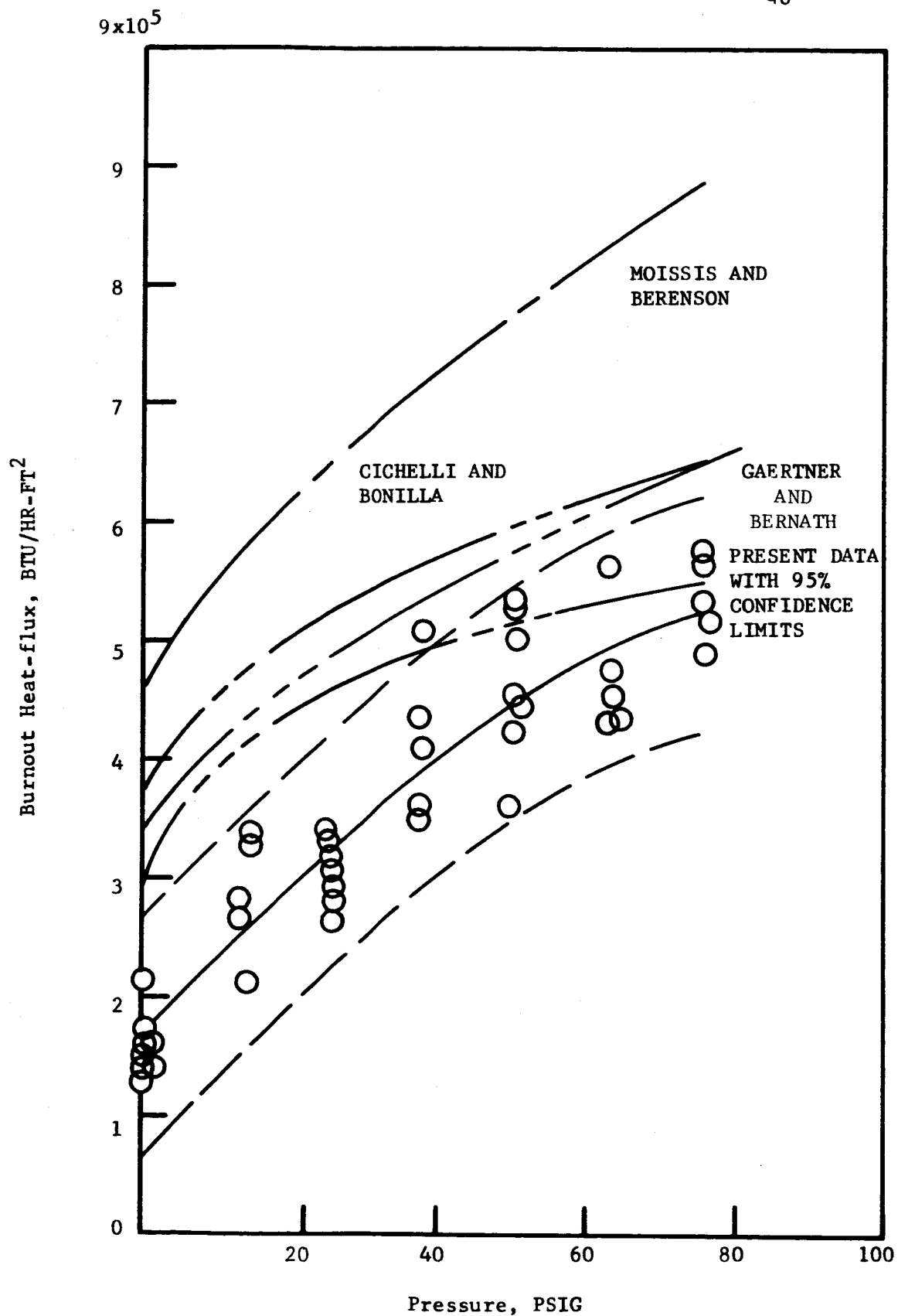
Fig. 12 Steady-state Burnout Heat-flux Versus Pressure (Fig. 2, ref. 4)
