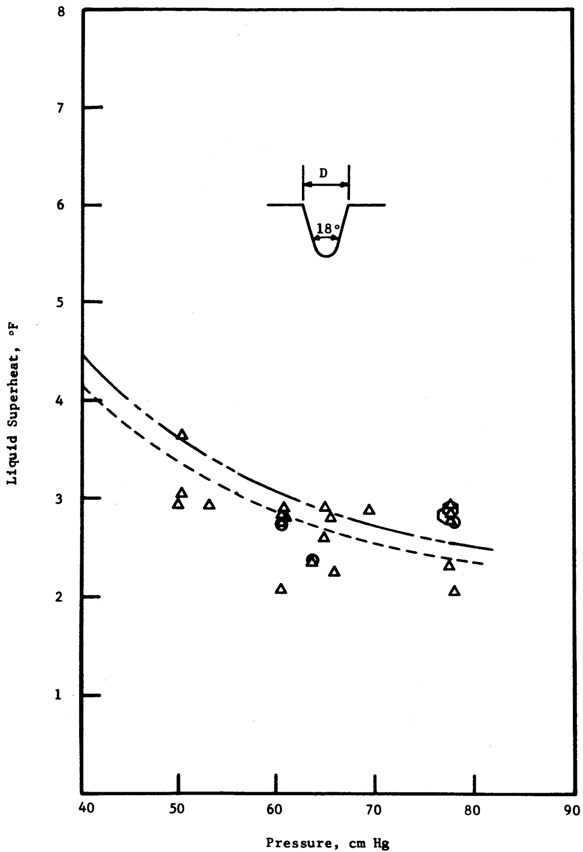
Fig. 2 Superheat Versus Pressure for Cavity of Diameter, D = 0.0018 in. (data from Fig. 7, ref. 7)
