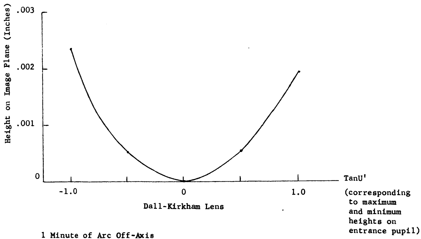
Figure 3-6. Aberration Curves of .020 Inch Decentered Secondary Mirror System
