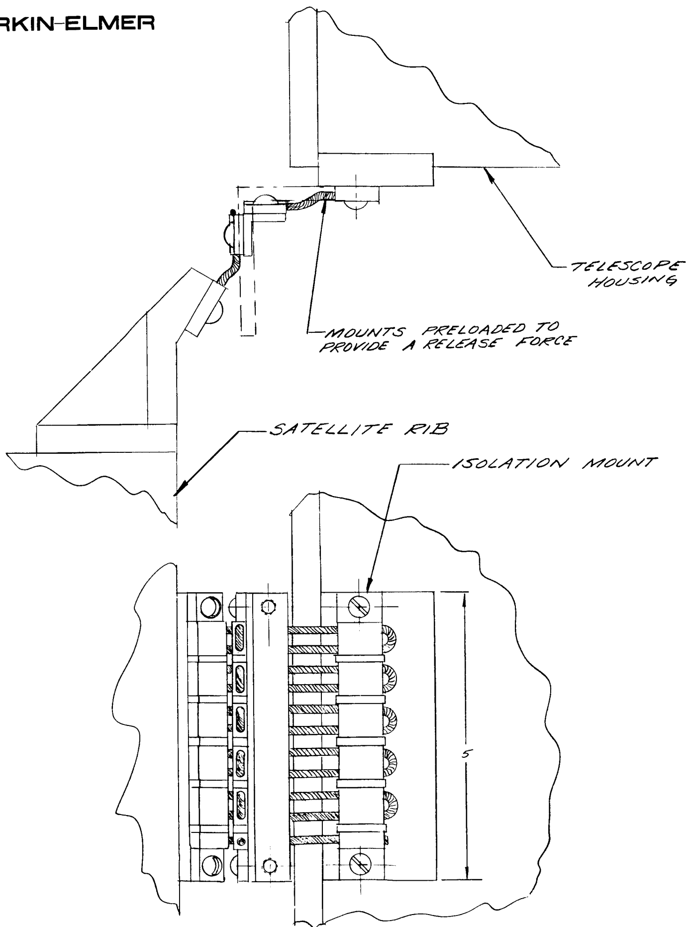
Figure 3-9. Isolation Arrangement
