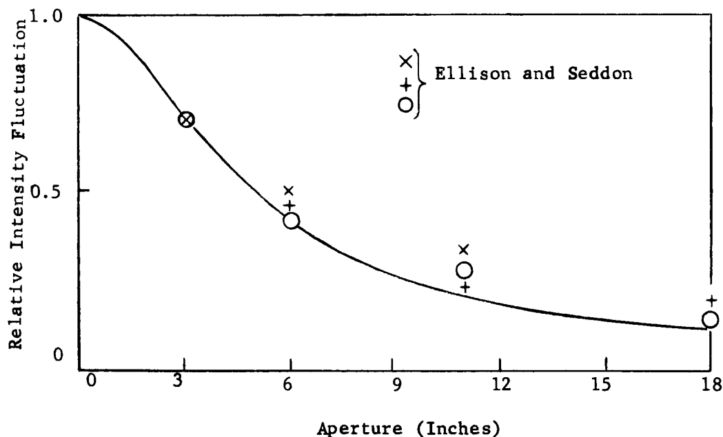
Figure 4-6. Scintillation Versus Telescope Aperture
