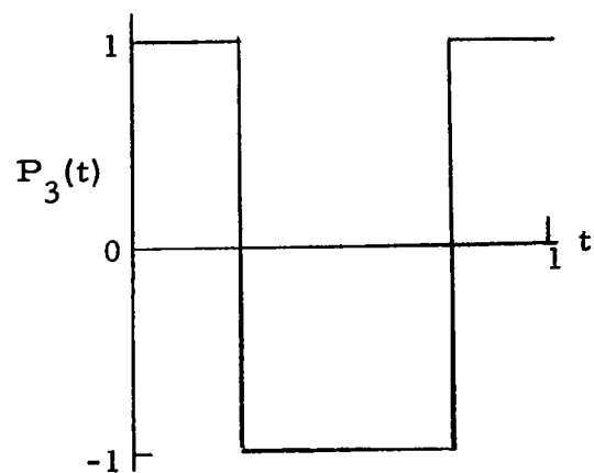
Figure 6. Walsh Functions
