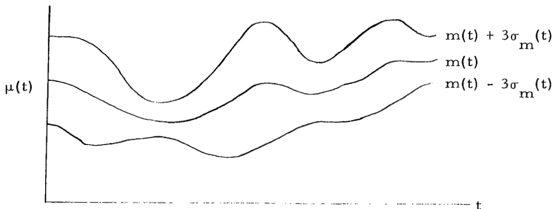
Figure 2. 89% Confidence Limits for Arbitrary Distribution based upon Tchebycheff Inequality
