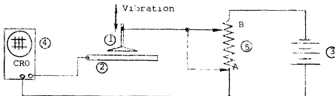
Fig. 4 SCHEMATIC OF CONTACT POTENTIAL APPARATUS
