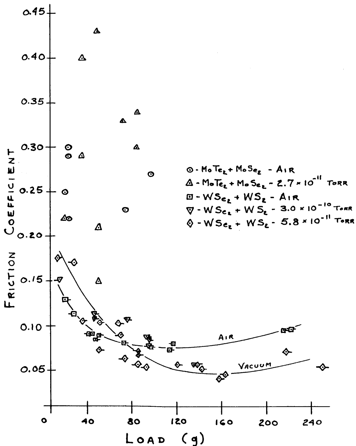
Fig. 5 FRICTION OF MODIFIED CRYSTAL STRUCTURE MATERIALS
