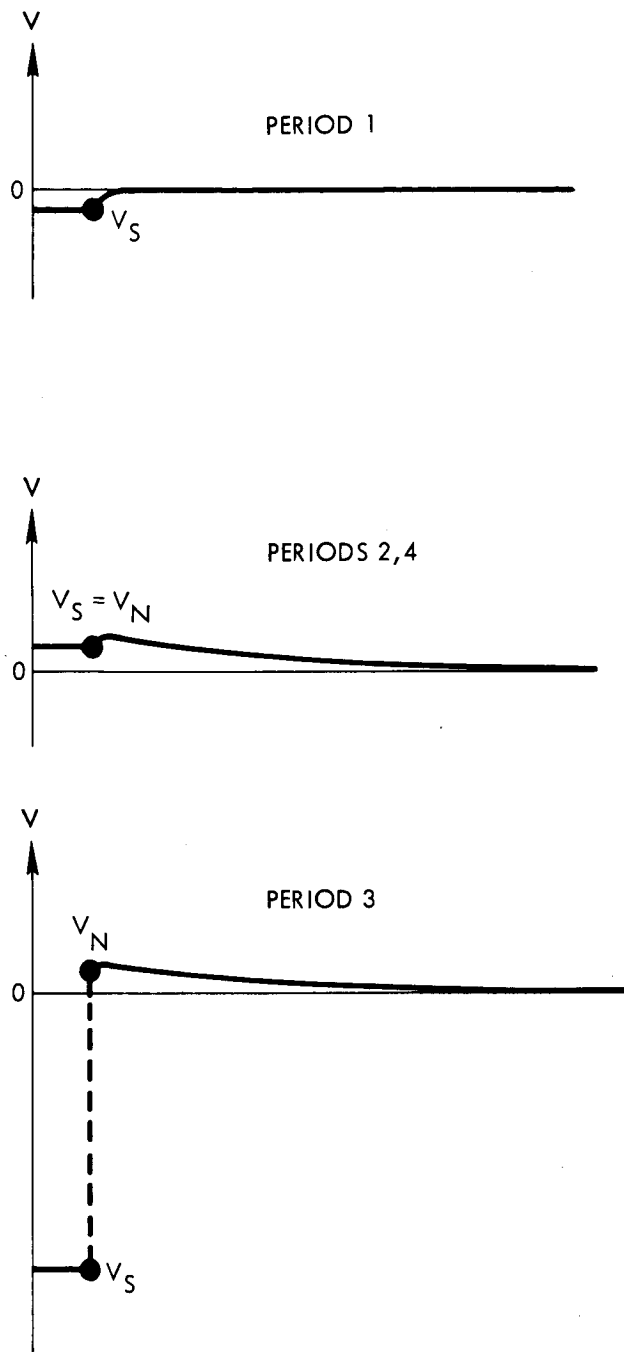
Figure 12. Model of potential configuration during the flight test. The plasma thrust beam is indicated by the curve from the dot outward to the potential of the ambient plasma ( V = 0 ). Vehicle potential, V_S , is indicated by the short horizontal bar.
