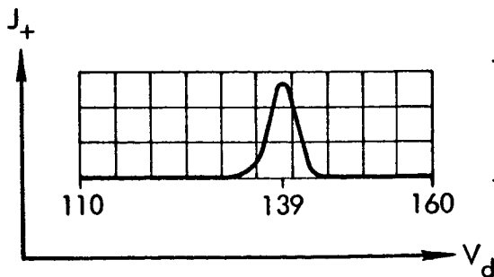
Figure 10a. Output of 127° analyzer. Perturbation voltage V_1 = 0 .
