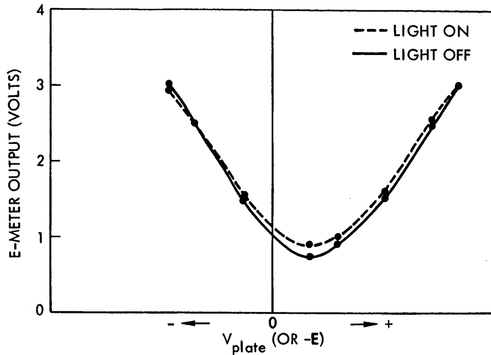
Figure 6. Photoelectric variation in E-meter response observed under uv illumination
