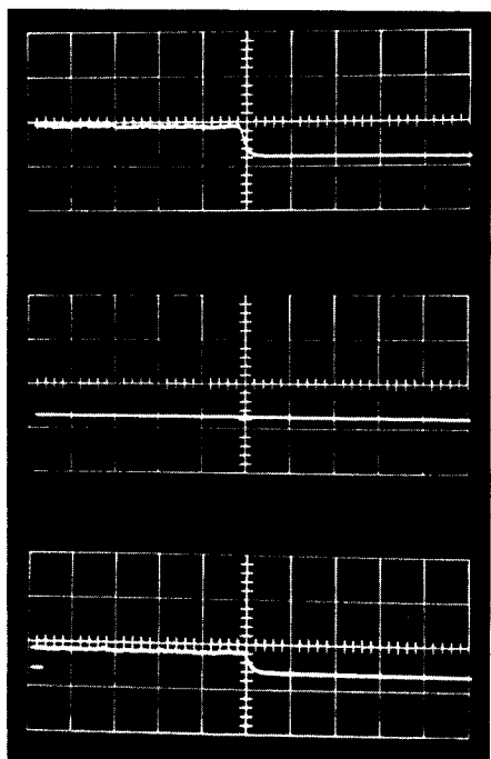
Figure 8. E-meter response in first plasma wind tunnel test. In all frames, vertical: E-meter high-sensitivity output (2V/div., zero at bottom) (Note: dc offset is about 2.4V.); horizontal sweep, 10 seconds full frame. Notes beside each frame indicate nature of change made as trace passed center of frame.
