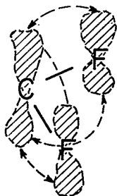
Figure 3a. Overlap of Non-Bonding Electrons of Fluorine with the Unfilled Orbital of Carbon.
