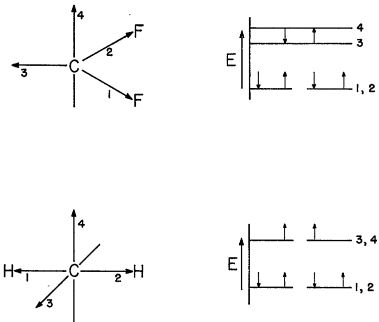
Figure 2. Possible Configurations for the Electronic Ground States of CF 2 and CH 2 .
