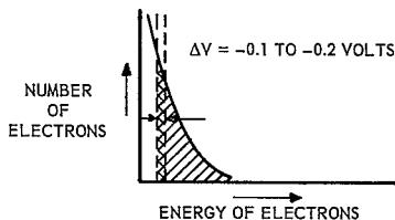
Figure 11. Effect of Retarding Potential Difference.
