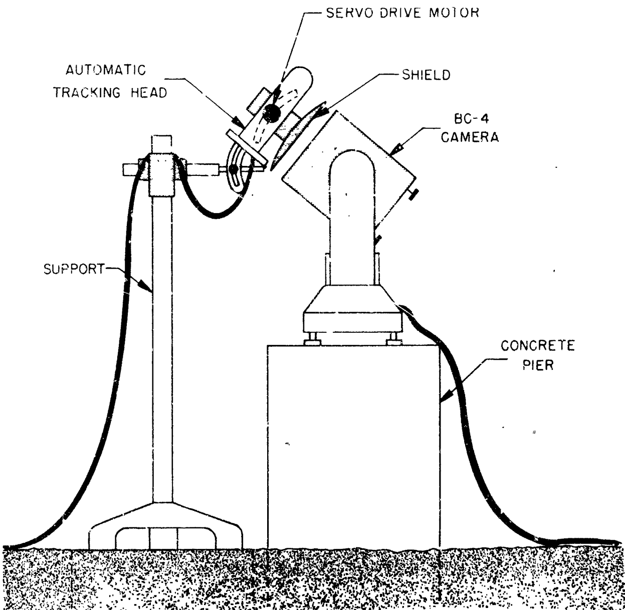
FIG. 3.7 LASER BEACON FILTER-COLLIMATOR TRACKING ASSEMBLY FOR BC-4 CAMERA
