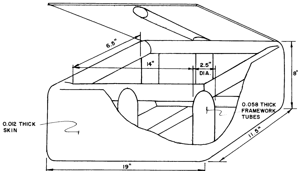
FRAME - MEMBRANE CONSTRUCTION
