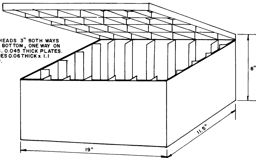
FRAME AND PLATE CONSTRUCTION 6
