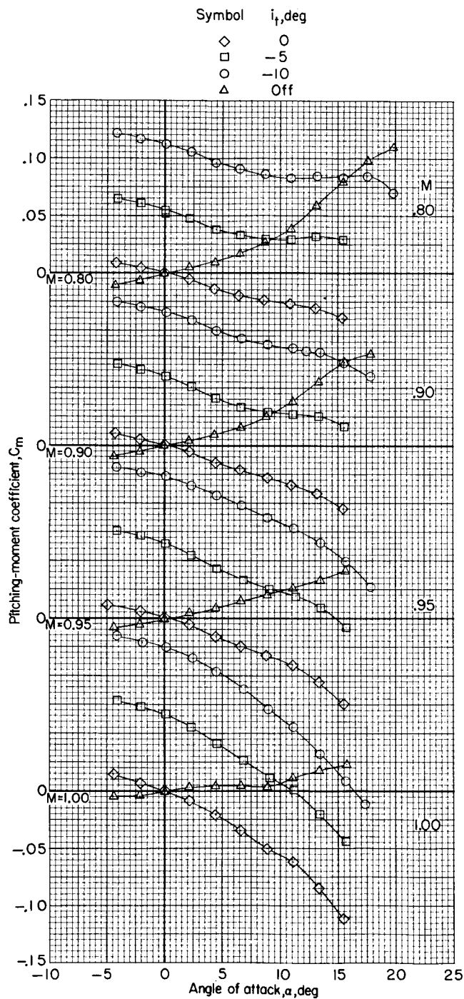
Figure 26.- Variation of pitching-moment coefficient with angle of attack at various horizontal-tail incidences. \Lambda = 75^\circ ; \beta = 0^\circ ; 8-foot transonic pressure tunnel.
