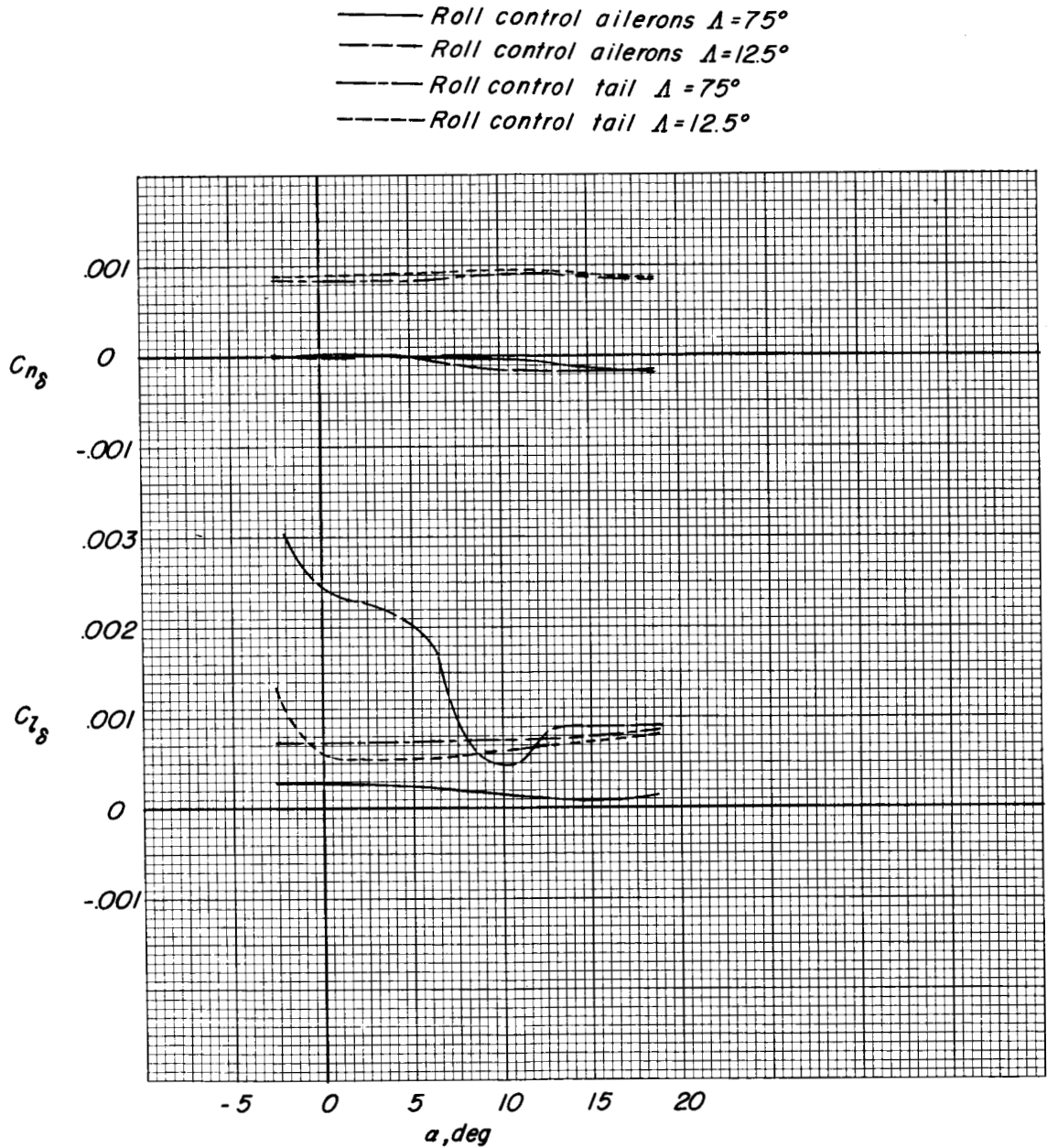
Figure 19.- Lateral control characteristics. M = 0.25 .
