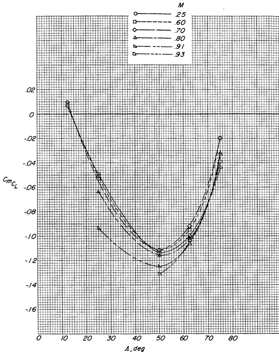
Figure 21.- Effect of wing leading-edge-sweep angle on the longitudinal stability for several Mach numbers.
