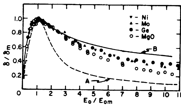
Fig. 8 Reduced yield curves for \text{Ni}^{20} , \text{Mo}^{20} , \text{Ge}^{23} and \text{MgO}^{46} . Curve A represents Baroodys equation (6.10) Curve B represents Eq. (7.3) for n = 1.35 .
