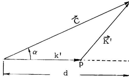
Fig. A.1. Vector diagram of conservation of momentum. Principle \vec{c} = \vec{k} + \vec{K} + \frac{2\pi\vec{p}}{\lambda} that
