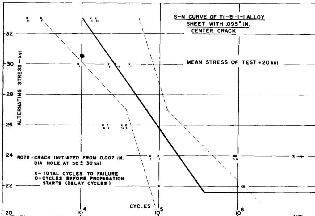
Figure 15. S-N Curve of Ti 8-1-1 alloy sheet with 0.095 in. center crack, 20 ksi mean stress.
