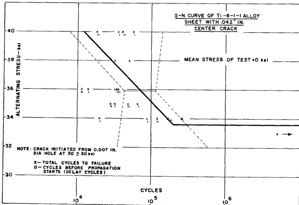
Figure 11. S-N Curve of Ti 8-1-1 alloy sheet with 0.042 in. center crack, 0 ksi mean stress.
