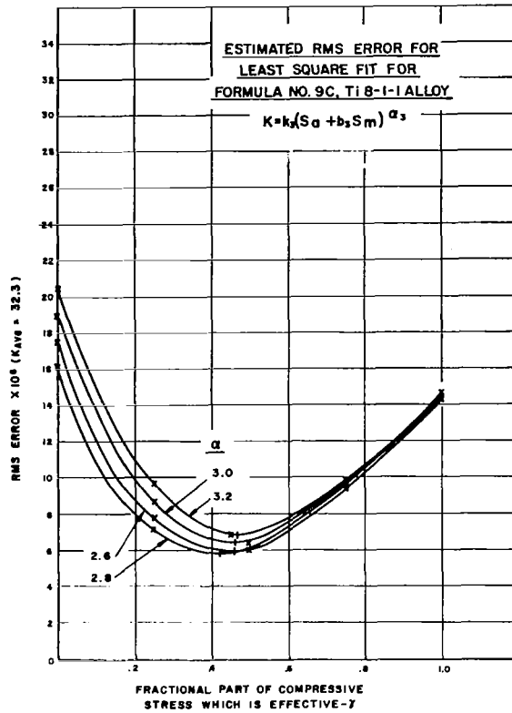
Figure 30. Estimated RMS error for least square fit for formula No. 9c Ti 8-1-1 alloy.
