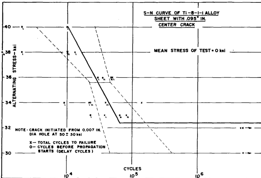
Figure 14. S-N Curve of Ti 8-1-1 alloy sheet with 0.095 in. center crack, 0 ksi mean stress.
