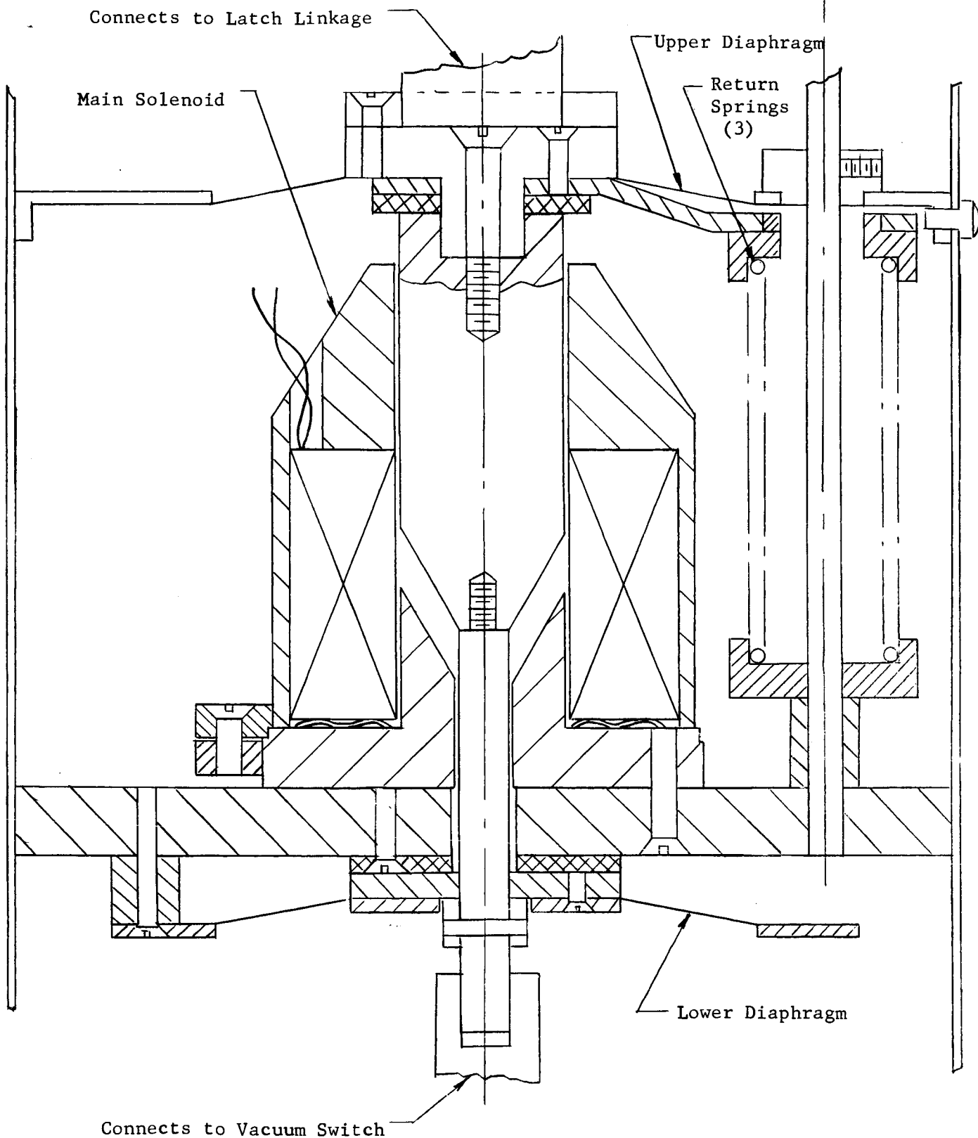
Figure 15. Main Solenoid & Diaphragms
