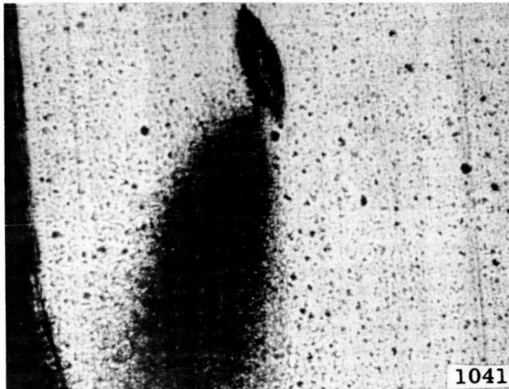
FIGURE 8: Cavitation Pitting in Columbium-1% Zirconium After 50 Hours Exposure to "Nose" Cavitation in Mercury at a Throat Velocity of 48 feet/second. Magnification 120X
