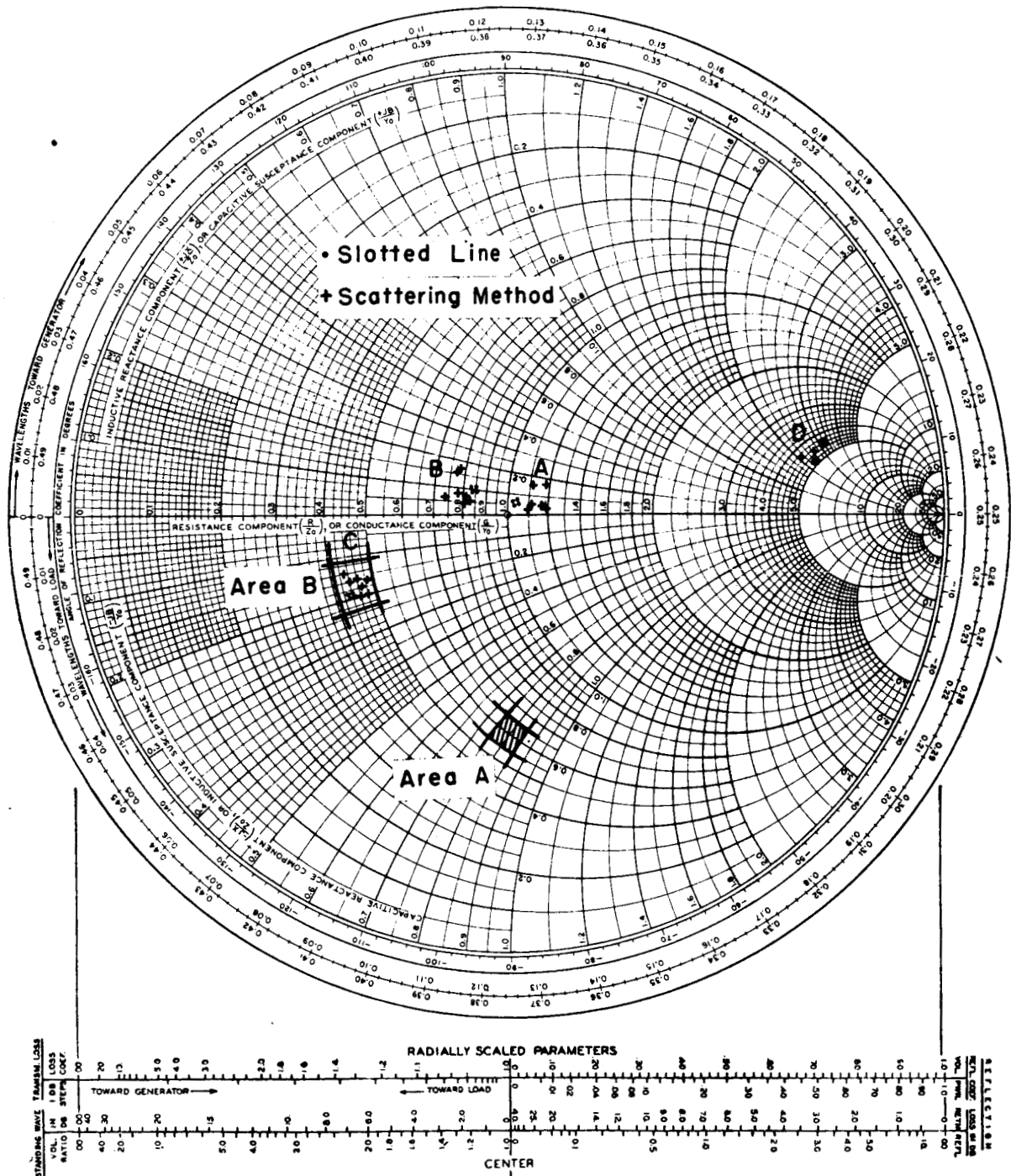
Fig. 16. Comparison of antenna impedance values obtained by slotted line and scattering method at 10.00 Kmc. Area A, typical illustration of estimating distribution of Z_a/Z_{c2} by graphical analysis. Area B, estimated error of antenna designated C in text.
