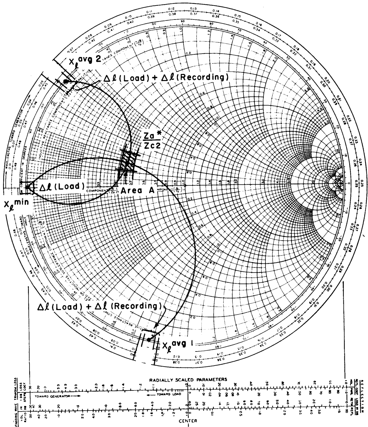
Fig. 18. Graphical determination of Z_a^*/Z_{c2} and error analysis of antenna C for \pm 0.0025\lambda load inherent error and recorder error of \pm 0.002\lambda in X_{l \text{ avg } 1} and \pm 0.0015\lambda in X_{l \text{ avg } 2} .
