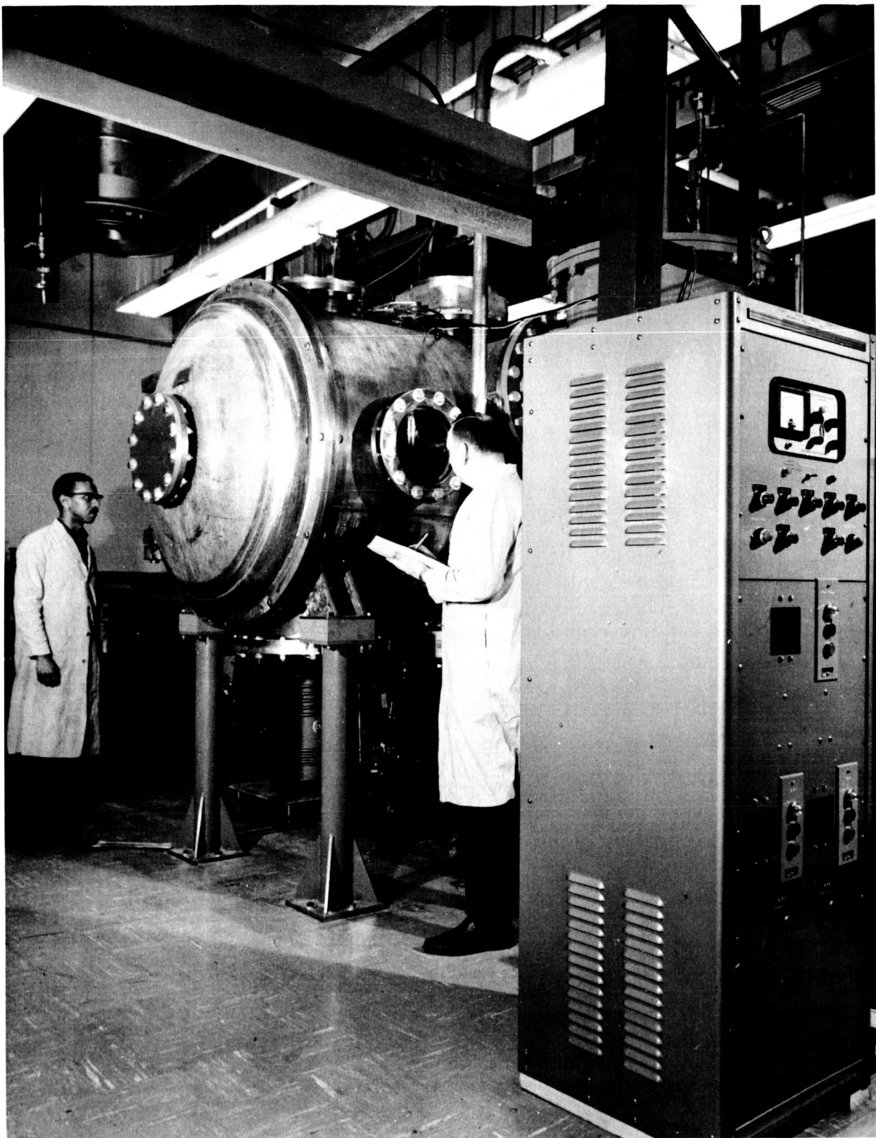
Figure 2. Vacuum Facility
