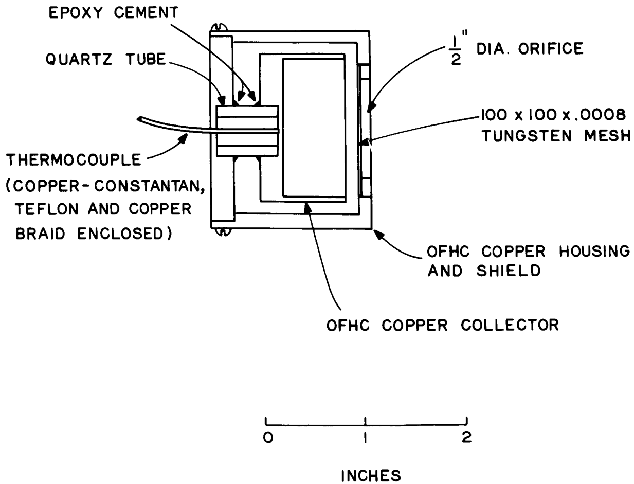
Figure 13. Diode Probe
