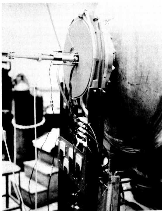
Figure 7. Photograph of Assembled Axial-Injection (Mark IV) Accelerator
