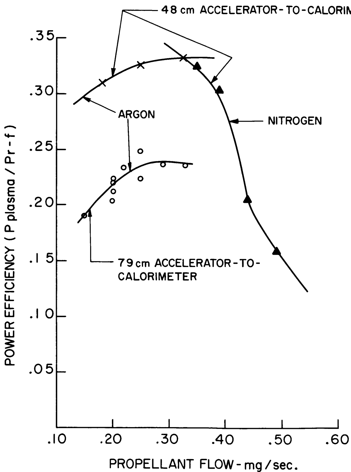
Figure 23. Dependence of Power Efficiency on Propellant Flow Rate, Propellant Species and Calorimeter Position, Mark IV-L Accelerator
