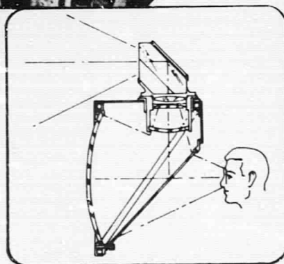
Spherical-mirror viewing system
