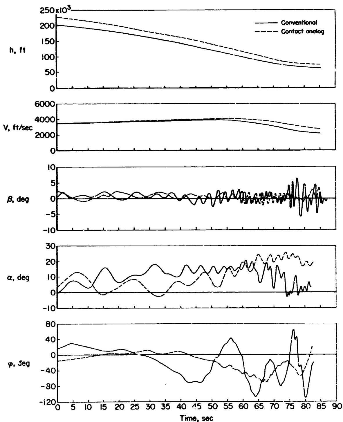
Fig. 9 Pilot performance during a simulated X-15 reentry using the standard X-15 display panel and the contact analog display system
