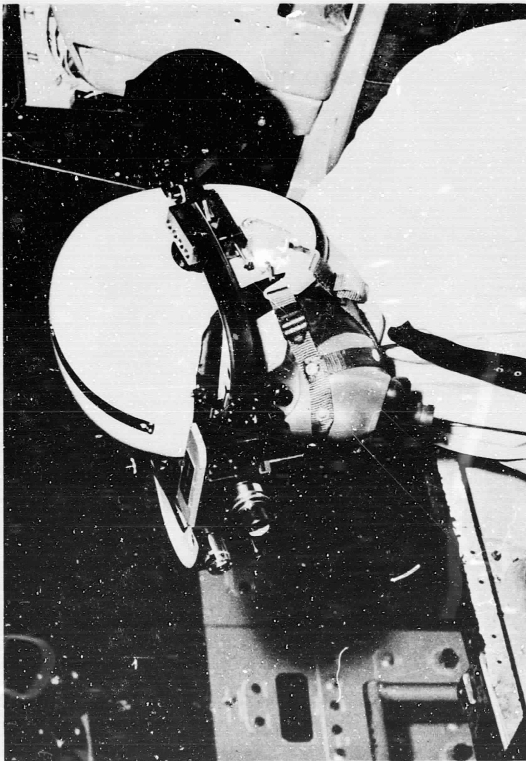
Fig.1 Eye-position recording camera
