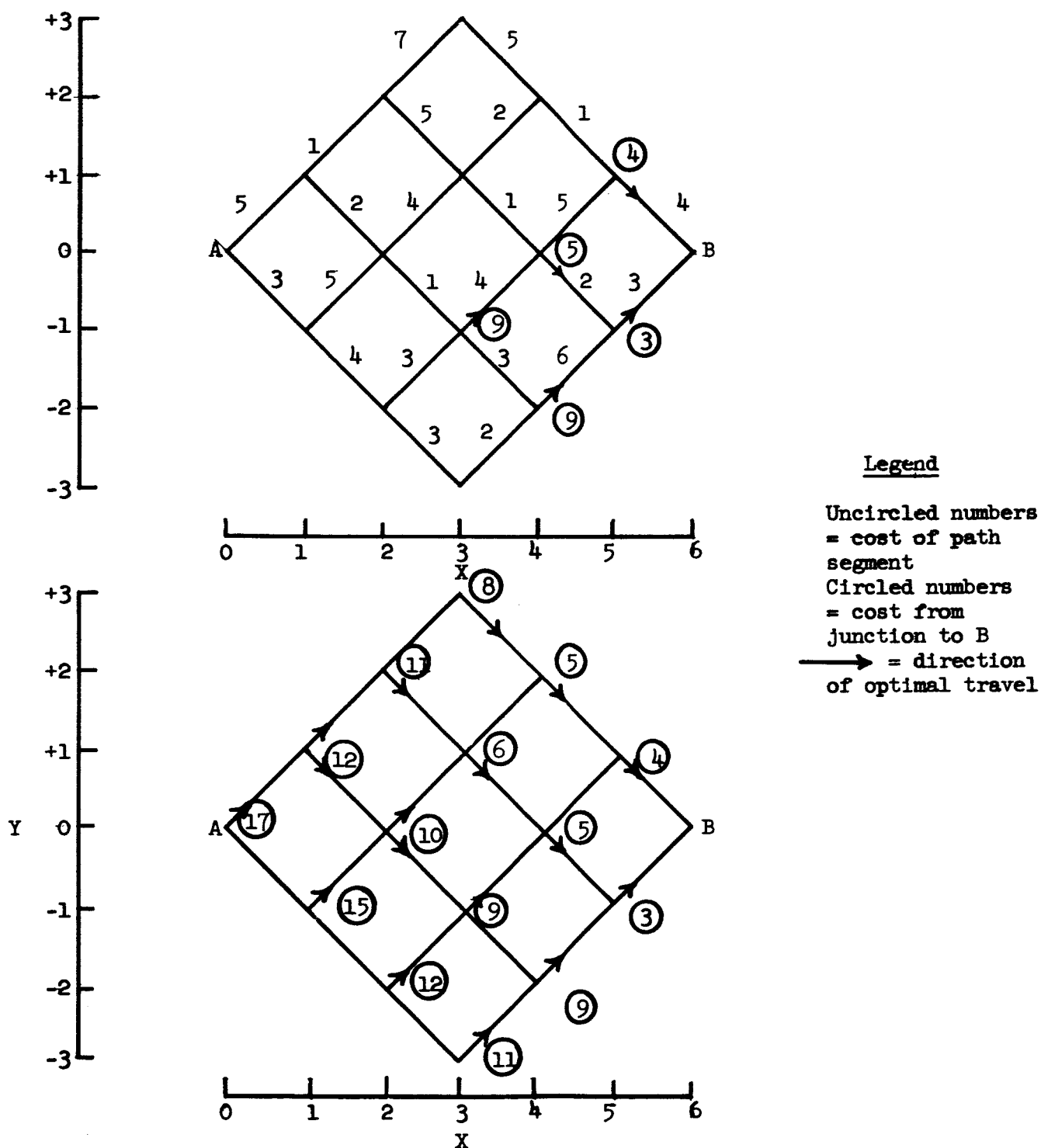
Figure 2. An example of dynamic programming 3
