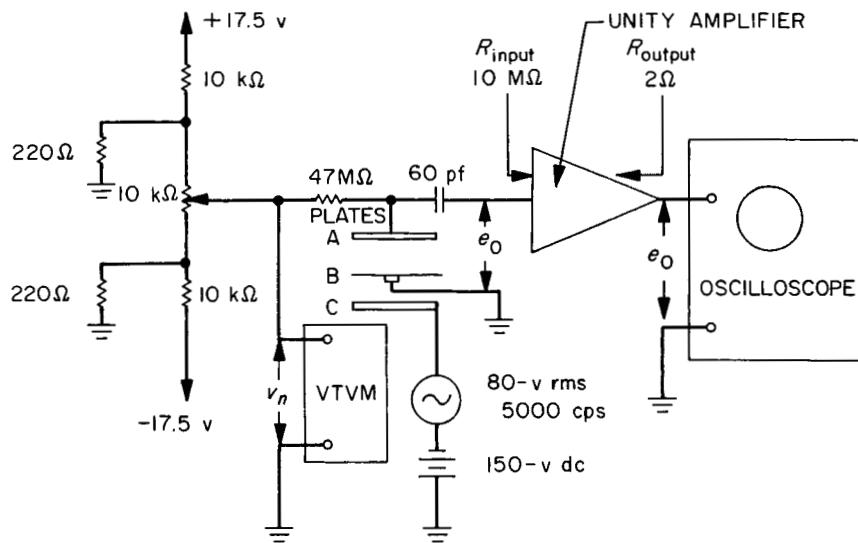
Fig. 7. Test setup used for measuring contact potential
