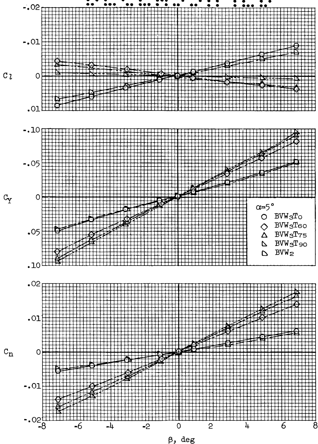
Figure 27.- Effect of tip deflection on the lateral and directional characteristics of the swept wing configuration at 5^\circ angle of attack.
