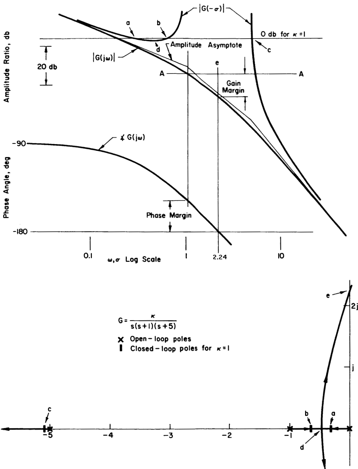
Figure D-1. Example of the Combined Use of Root-Locus and Bode Diagrams
