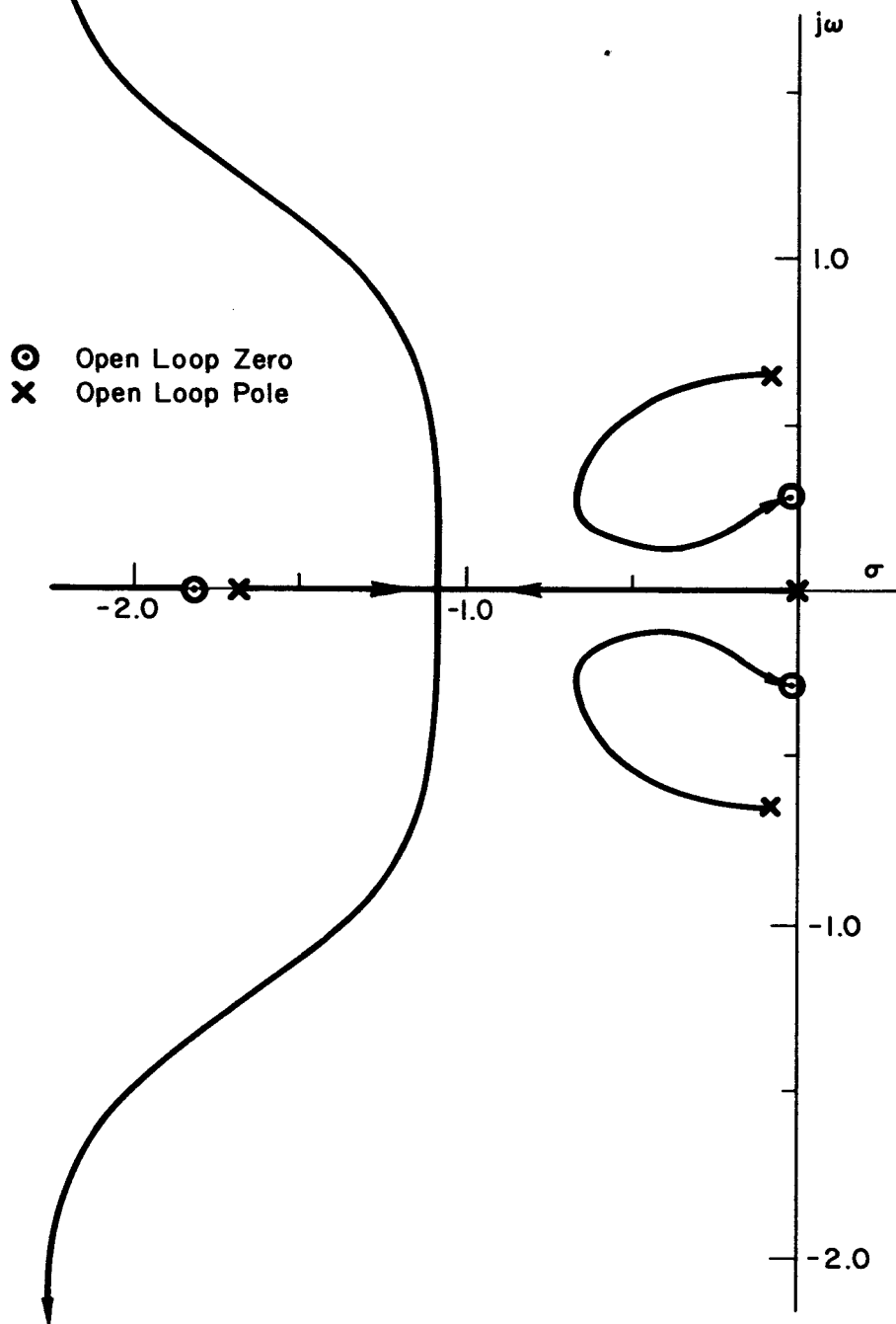
Figure 10. SCAT 16, Bare Airplane, Yaw-Rate Closure
