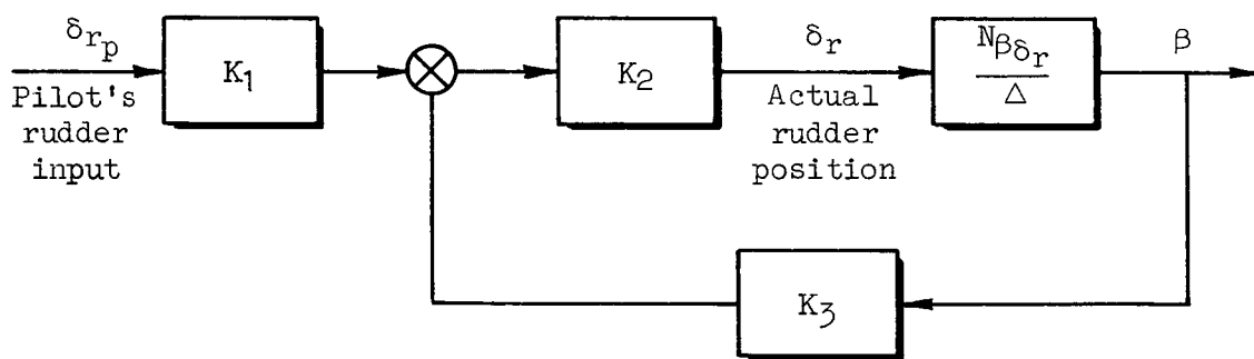
Figure 14. Sideslip-to-Rudder Feedback
