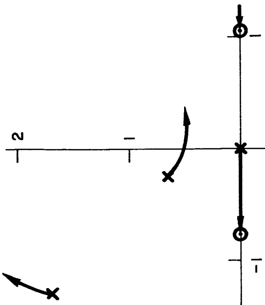
High-Gain Roll Inner Loop
