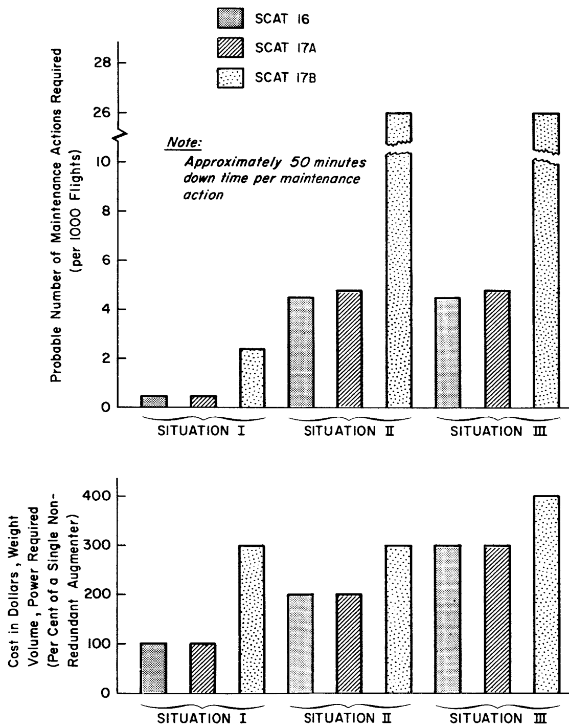
Figure 33. Probable Number of Maintenance Actions and Augmenter "Cost"
