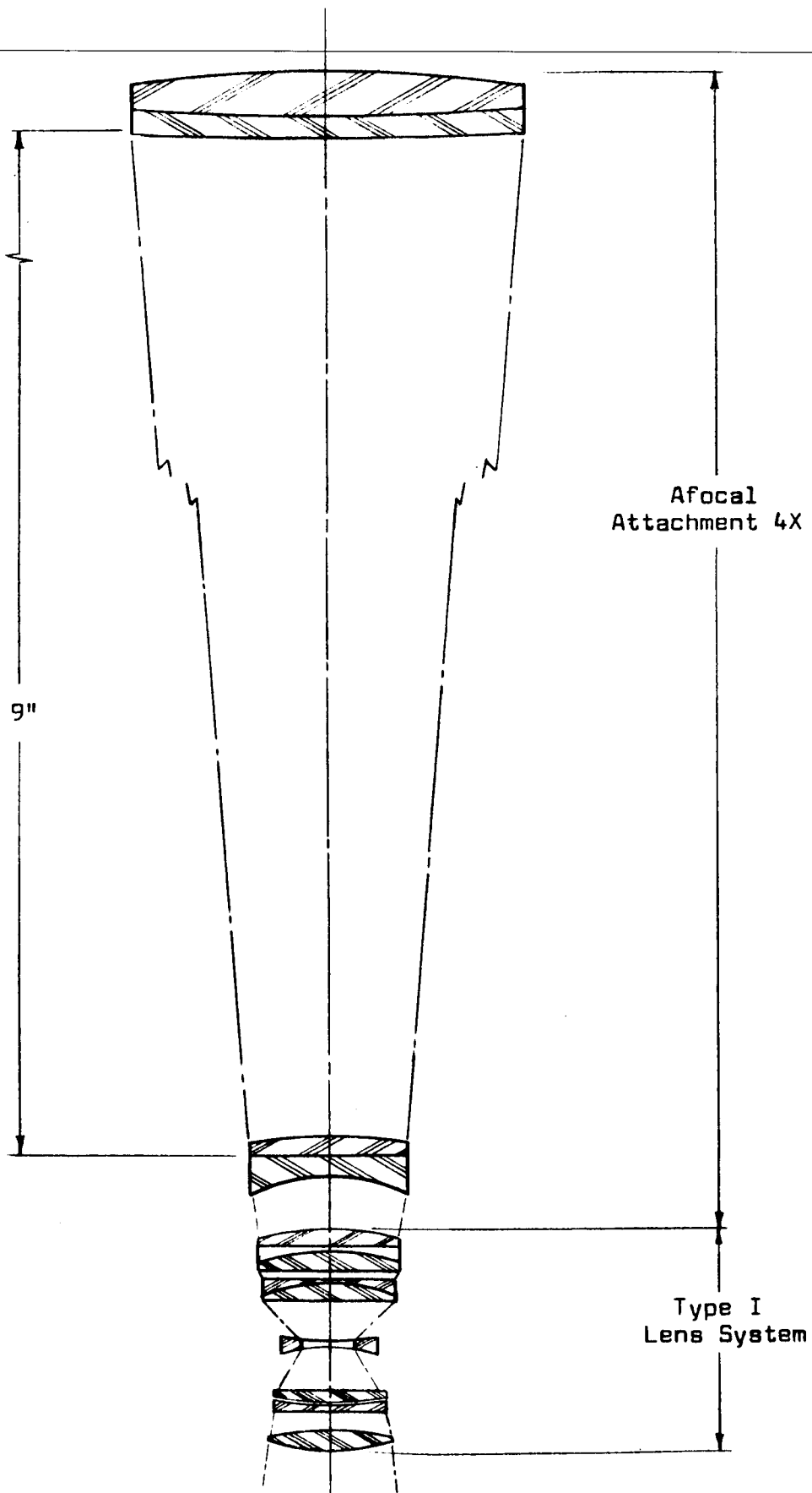
AFOCAL ATTACHMENT
