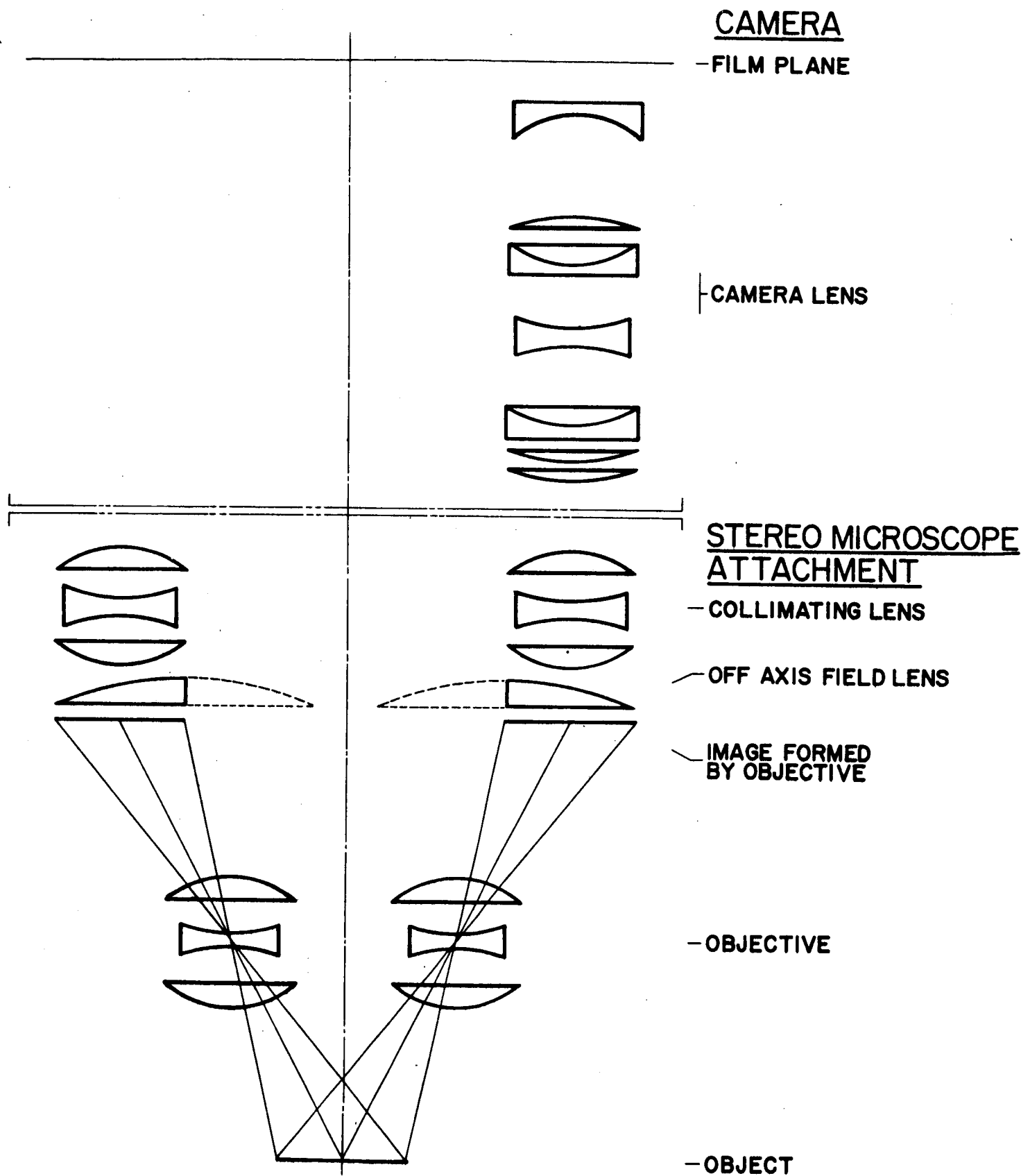
HIGH RESOLUTION - LOW DISTORTION STEREO MICROSCOPE ATTACHMENT
