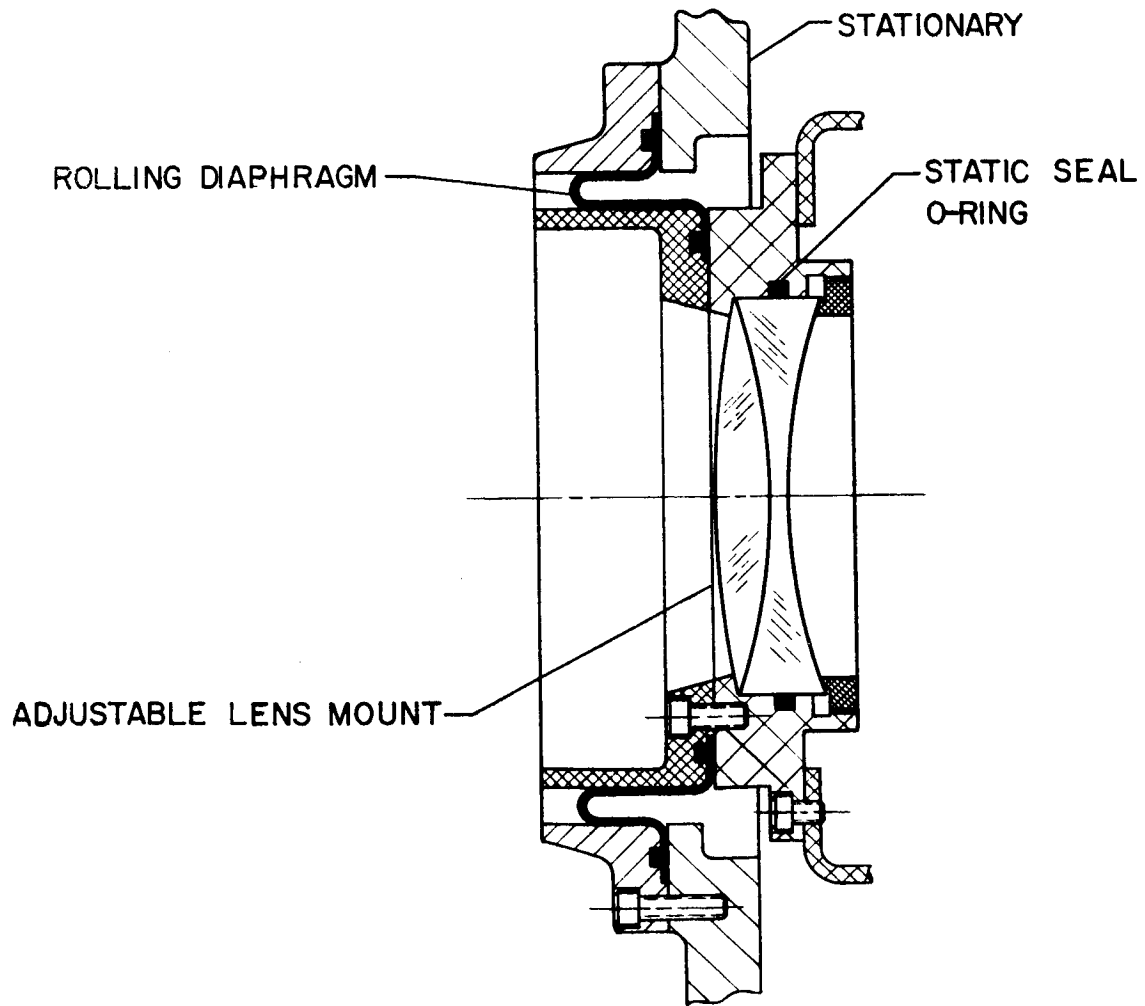
SEALS FOR LINEAR MOTIONS
